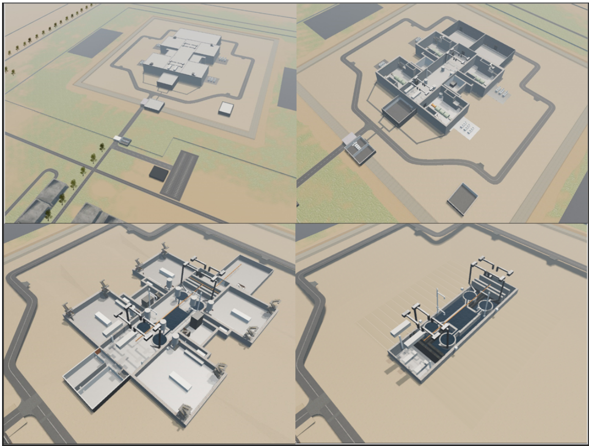
Figure 1 Hypothetical SMR Facility. Above-grade (top left), basement one (top right), basement two (bottom left), basement three (bottom right).
