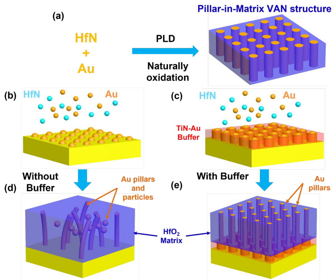
Fig. 1 Schematic of experiments design: (a) Schematic of \text{HfO}_2 -Au VAN structure designed, and (b, c, d, e) schematics showing crystallinity and orientations of the films deposited with and without TiN-Au buffer.
