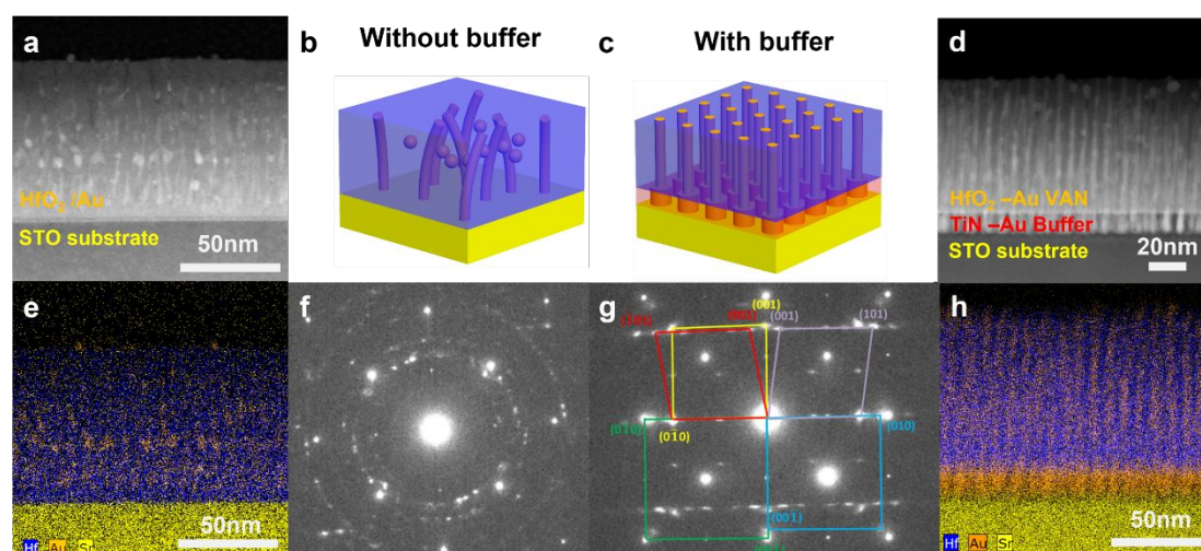
Fig. 3 Cross-section of HfO 2 -Au thin film on STO with and without TiN-Au buffer. (b,c) Schematic of the structures with and without TiN-Au buffer, (a,d) HAADF-STEM images of two films, (f,g) corresponding diffraction patterns, and (e,h) EDS element maps.
