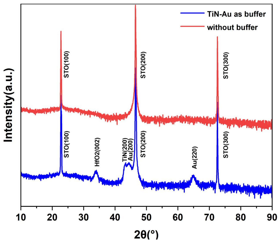
Fig. 2 XRD \theta - 2\theta pattern of HfO 2 -Au thin films grown on SrTiO 3 (STO) (001) with or without TiN-Au buffer layer.
