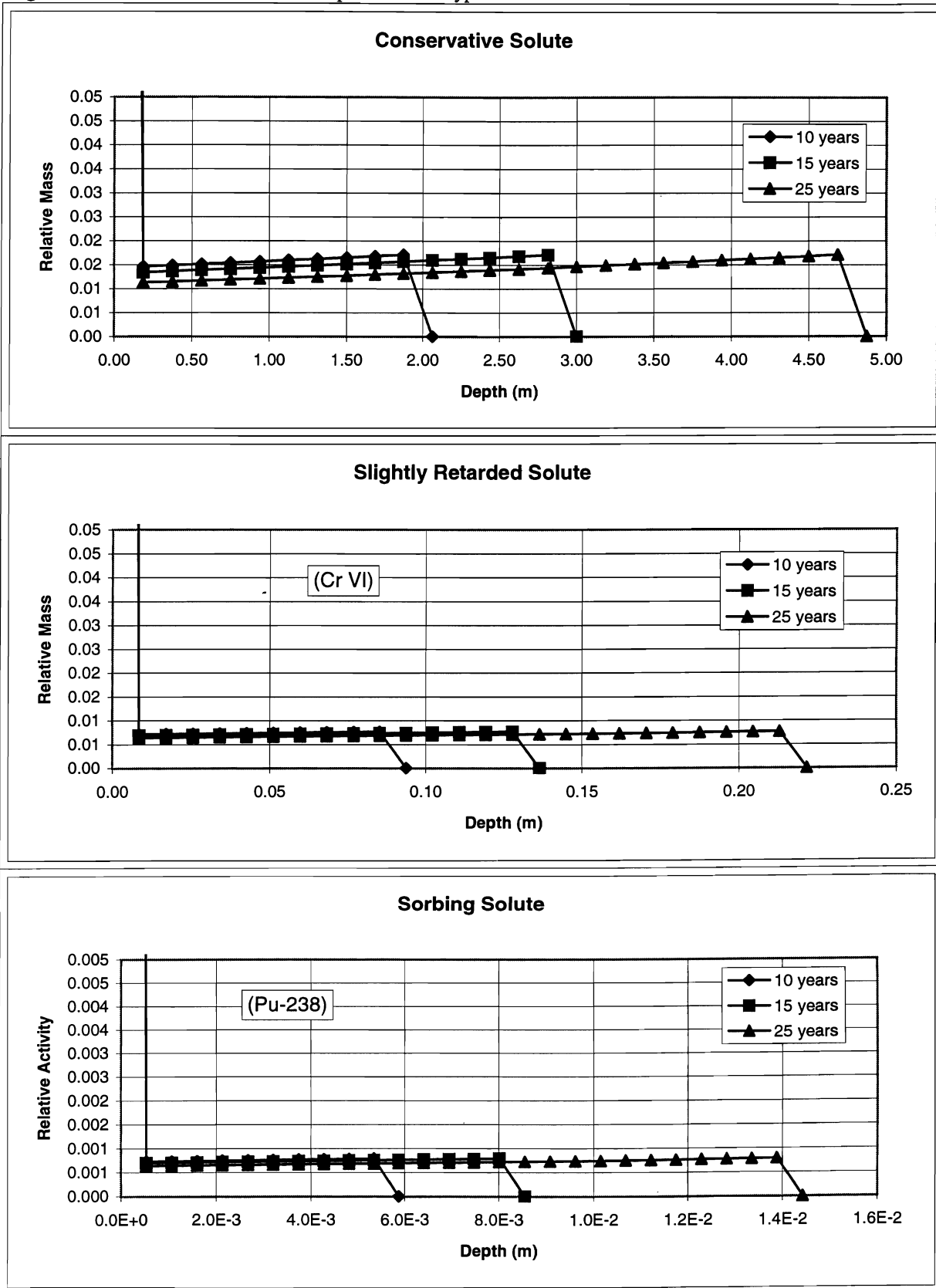
Figure 2. Plots of solute mass with depth for three types of solutes.
