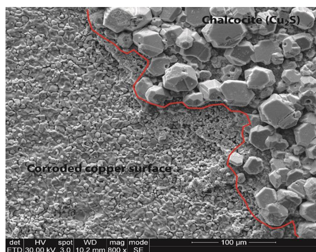
Fig. 4. Post-experiment SEM image of corroded copper surface (lower left) and the secondary chalcocite surface growth (upper right) [7, 9].
