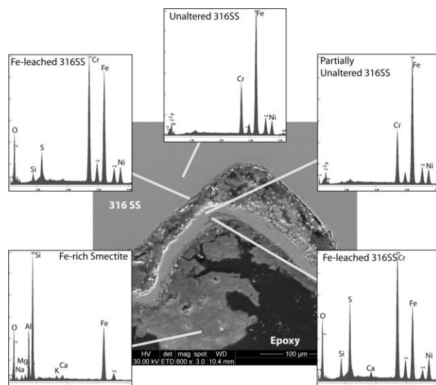
Fig. 2. SEM image showing a cross-section of 316SS run product depicting Fe-saponite/chlorite growth. Chemical analyses of 316SS and interface run products show significant Fe leaching from the steel surface and formation of a Cr-rich outer layer [4, 6].
