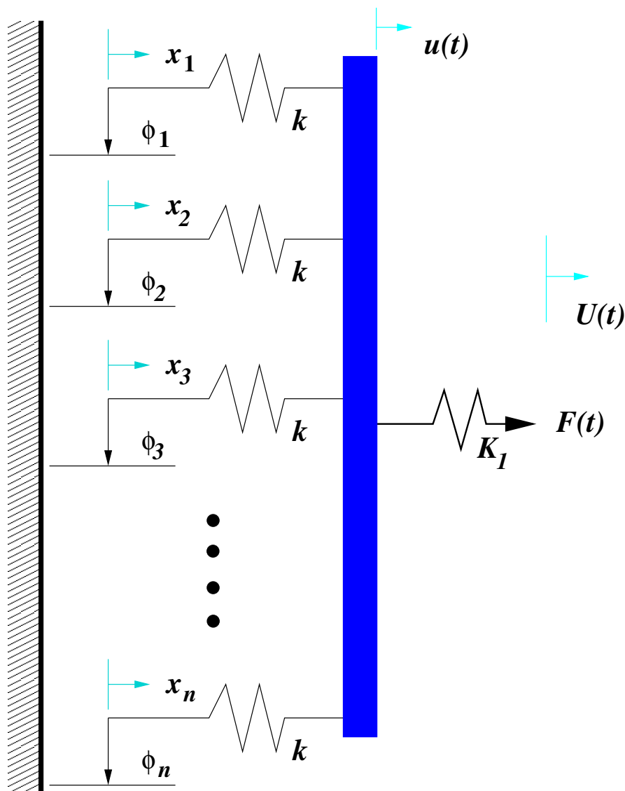
Figure 5-39. – Iwan Constitutive Model.
