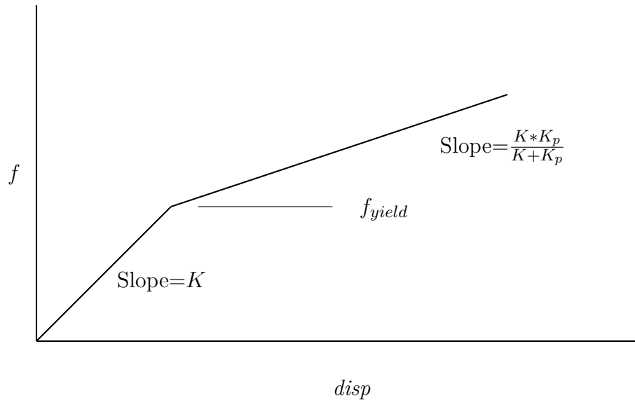
Figure 5-43. – Eplastic Model.
