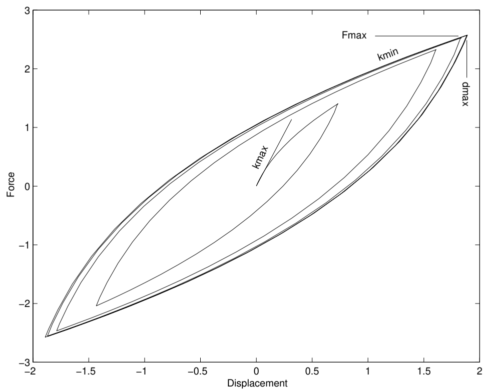
Figure 5-38. – Hys element parameters.
