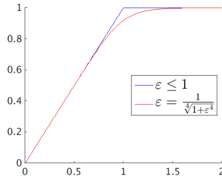
Figure 5-29. – Function for nquad_eps_max .
