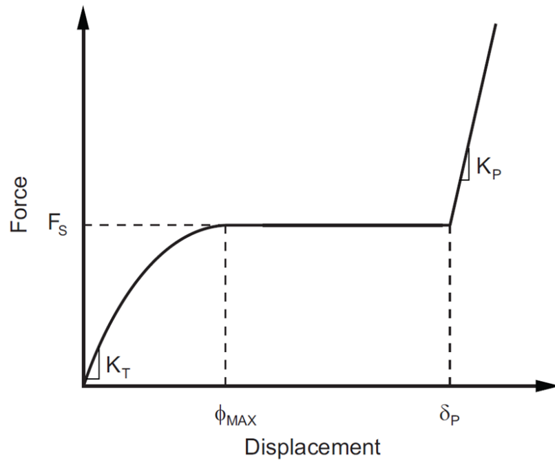
Figure 5-42. – Reduced Iwan Load Displacement Curve.
