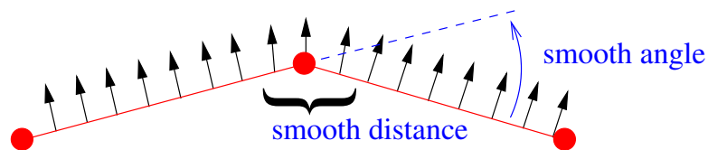
Figure 8-66. – Smoothing Parameters for Surface Normal Vectors. No smoothing occurs for faces that are misaligned by more than the specified “smooth angle”. Within the “smooth distance”, normal vectors vary linearly with relative distance from the node.
