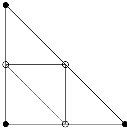
Figure 5-28. – Tria6 Element.
