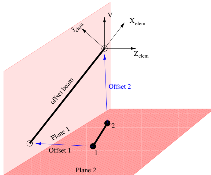
Figure 5-37. – Nbeam Orientation, Offset and Local Coordinate System. The coordinate system is in the plane of the offset beam . The plane is defined by the offset beam and the orientation vector, \vec{V} .
