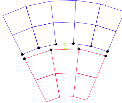
Figure 5-52. – Tied Joint Geometry. The two side set surfaces are shown separated for clarity. A virtual element is created which connects only the shear components of the joint. Normal components are interconnected using Tied MPCs.
