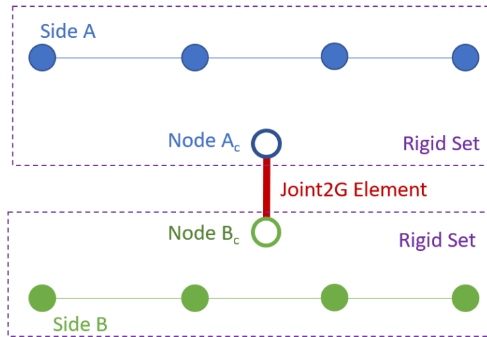
Figure 5-55. – Construction of tied joint with side=rigid.
