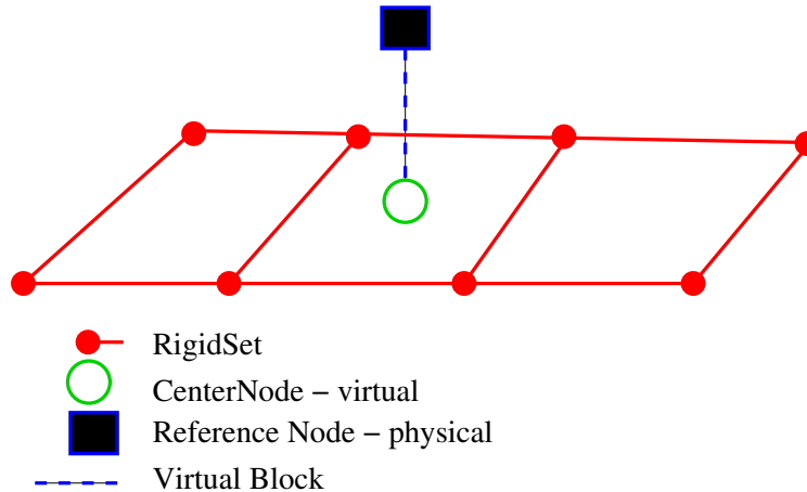
Figure 5-50. – Rigidset/TiedJoint Centernode Connection. The model illustrates the connection of a physical rigid set to a physical reference node via a virtual center node and virtual connection block.
