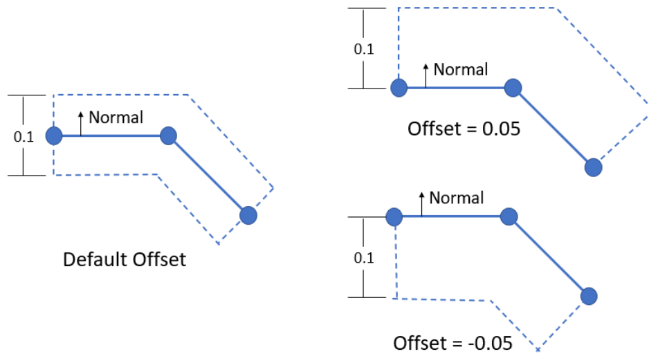
Figure 5-34. – Offset examples for shell of thickness 0.1.
