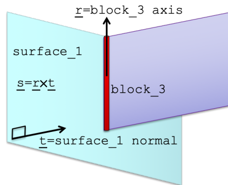
Figure 5-44. – Line weld definitions for attaching the purple and cyan shells. The line weld follows the red beam, which is contiguously meshed with the purple shell.
