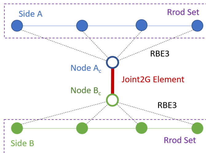
Figure 5-56. – Construction of tied joint with side=Rrod.
