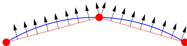
Figure 8-65. – Normal Definitions on Faceted Geometry. When low order elements are used to describe a curved boundary, the normal is poorly defined at the edge of the facets.
