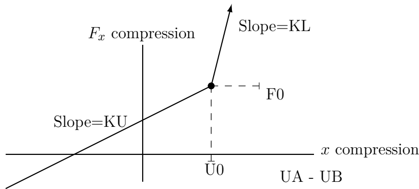
Figure 5-46. – Gap element Force-Deflection Curve.
