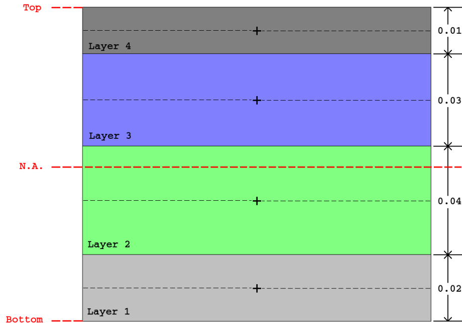
Figure 5-33. – Stacking arrangement for a multi layer shell element.
