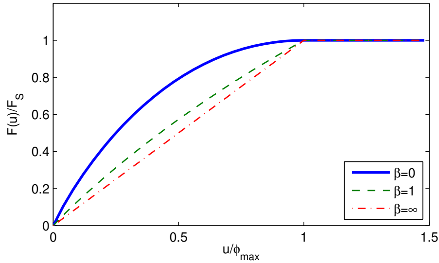
Figure 5-41. – Dimensionless static loading curves for the four-parameter Iwan model with \chi = -1/2 and three values of \beta , as the model goes into macroslip.
