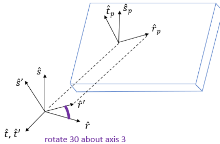
Figure 5-31. – Rotation of global coordinate system about axis prior to projection to shell.
