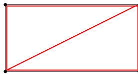
Figure 5-51. – Rrodset Constraints. The black lines indicate the edge of the element. Red lines are corresponding linear constraints.
