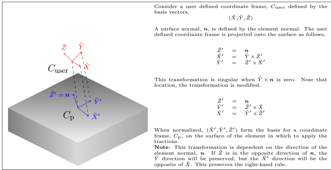
Figure 6-58. – Coordinate Frame Projection for Traction
