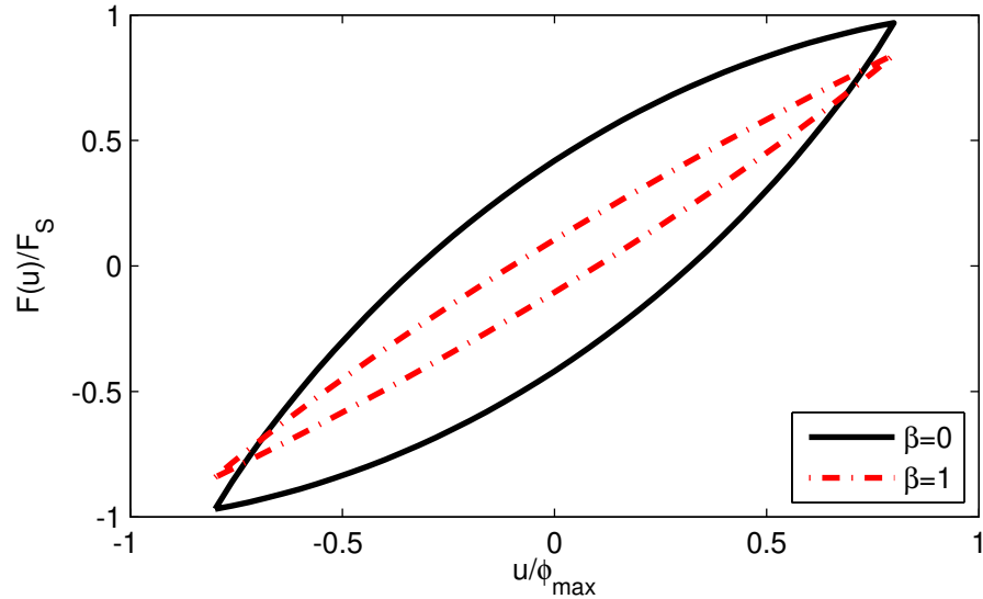
Figure 5-40. – Dimensionless hysteresis curves for the four-parameter Iwan model with \chi = -1/2 and two values of \beta .
