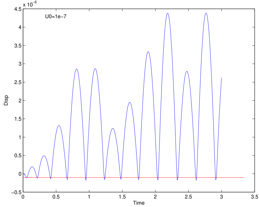
Figure 5-47. – Mass bouncing off a Gap. With this large time step the model is not conserving energy. Reducing the time step is required to correct the problem.
