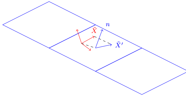
Figure 5-53. – The surface normal, n , is defined by the normal of the surface at the centroid point. The shear axis direction (in this example \tilde{X} ) is projected onto the surface as \tilde{X}' . Together, \tilde{X}' and surface normal provide the basis for the generated coordinate frame.
