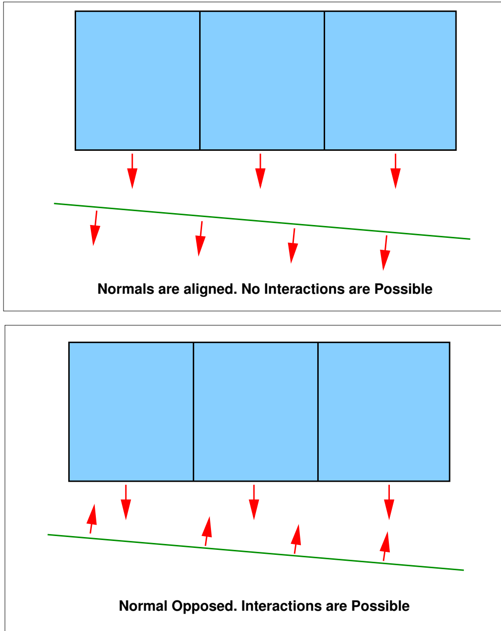
Figure 8-63. – Shell Normal in Contact or Tied Interactions.
