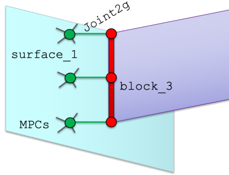
Figure 5-45. – Line weld Joint2G connections. The Joint2G elements are initially zero-length, and the green and red nodes coincident, but they are depicted with a finite deformation to delineate the individual components.
