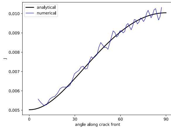
(c) Case 3: procedural transfer - CTet10 to UGHex8
