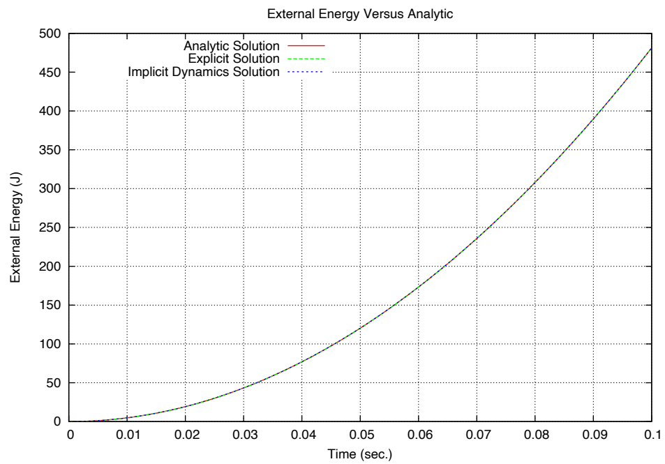
Figure 4-4. Energy-time curve
