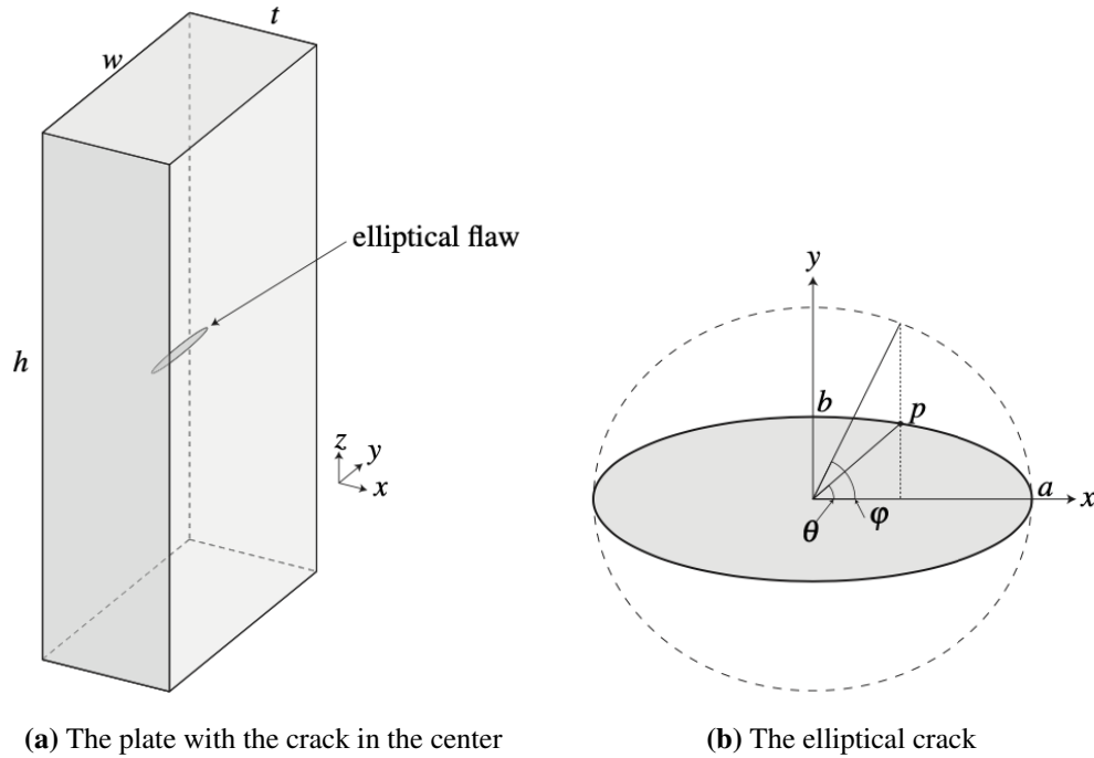
Figure 6-1. Geometry of the plate with an embedded elliptical crack. The FE model is one-eighth of the plate (one-quarter of the crack) and uses x-, y-, and z-symmetry BC's.
