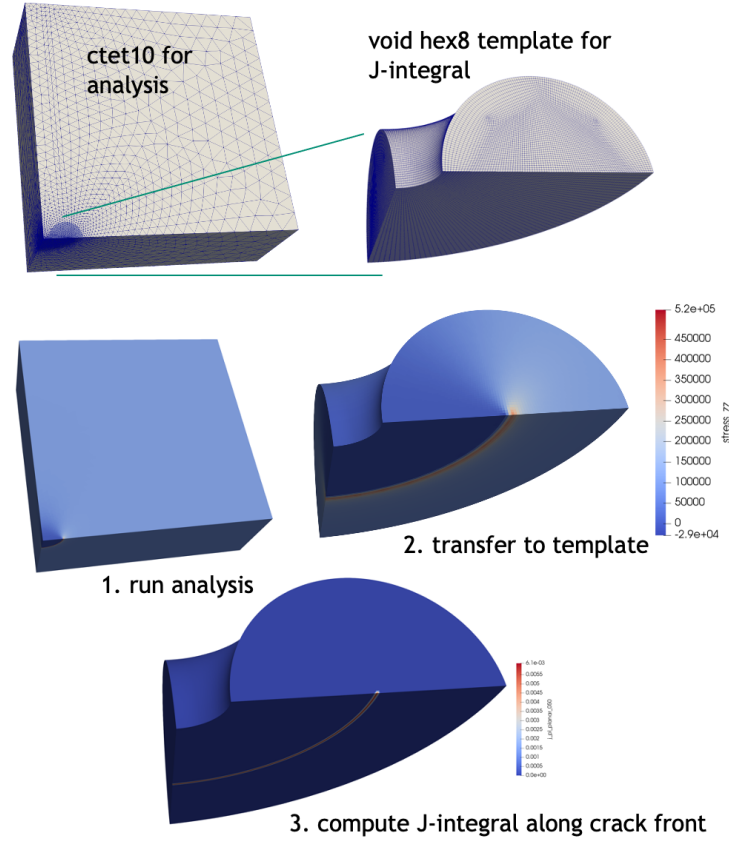
Figure 6-2. Illustration of crack template-based approach for J-integral calculations.
