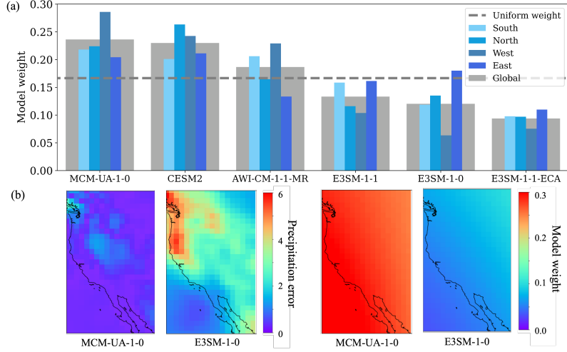
Figure 5: (a) Temporally averaged weights in the entire domain (Global) and the four regions (see Appendix A.2); (b) Prediction error and model weights of models MCM-UA-1-0 and E3SM-1-0 in the West region.
