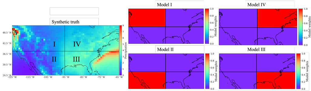
Figure 7: (a) Rescaled ERA5 precipitation data serving as a synthetic truth; (b) Model weights recovered by BNN. BNN only assigns weights to the regions where they are skillful.
