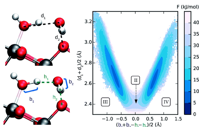
Figure 4. Enhanced sampling allows mapping the free-energy landscape of proton transfer at an aqueous TiO 2 interface as a function of collective variables based on O–O and O–H distances. 47 The predicted barrier of 25 kJ/mol would make proton transfer too rare to capture in conventional MD simulations. Adapted with permission from ref 47. Copyright 2020 Royal Society of Chemistry under (CC BY-NC 3.0).).
