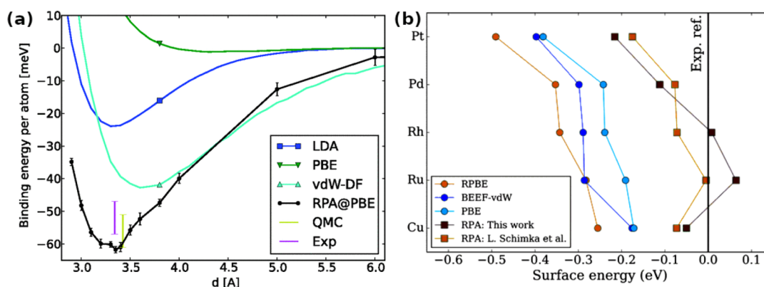
Figure 11. (a) Semilocal and nonlocal vdW-DF density functionals underestimate binding energy of graphite, while RPA agrees closely with QMC simulations and experiment. 160 (b) DFT also underestimates surface energies of metals, while RPA agrees with experiment. 183 (a) Adapted with permission from ref 160. Copyright 2013 American Physical Society. (b) Adapted with permission from ref 183. Copyright 2018 American Chemical Society.
