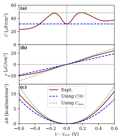
Figure 16. (a) The experimental capacitance of Ag(100) in aqueous solution of 0.1 mol/L KPF 6 (solid red), from ref 262, with the capacitance maximum (green dots) and the value at the PZC (blue dashes) marked. (b) Surface charge evaluated using the capacitance from experiment (solid red), the maximum (green dots), and the PZC (blue dashes). (c) Change in surface free energy relative to the PZC using the three capacitances defined above.
