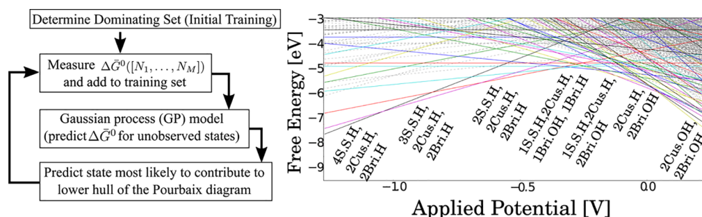
Figure 13. Determination of stable surface structures of \text{IrO}_2 as a function of electrochemical potential, 218 combining heuristics to generate structures, with ab initio methods and Gaussian process approximate models to evaluate energies of structures. The algorithm (left panel) captures a large number of surface structures, as depicted in the Pourbaix diagram (right panel). Adapted with permission from ref 218. Copyright 2016 American Chemical Society.
