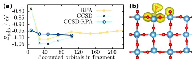
Figure 12. (a) Embedding coupled-cluster singles and doubles (CCSD) within random phase approximation (RPA) calculations results in better convergence with size of fragment compared to equivalent embedding within DFT. Results shown here for the adsorption energy of water on a TiO 2 (110) surface, with (b) showing the electron density from the occupied orbitals of the fragment treated using CCSD. 209 Adapted with permission from ref 209. Copyright 2021 with the permission of AIP Publishing.)
