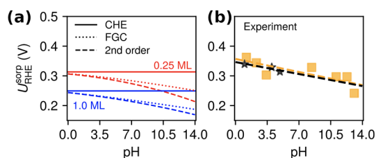
Figure 15. (a) Hydrogen binding on Pt(111), with hydrogen coverage of 1/4 monolayer (red) and 1 monolayer (blue). Full grand-canonical (FGC) and second-order models produce hydrogen binding curves as a function of pH that are similar to those measured from experiment (b), whereas the computational hydrogen electrode results do not vary with pH. Adapted with permission from ref 256. Copyright 2020 Springer Nature under (CC 4.0).
