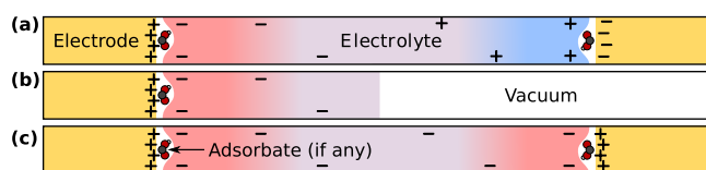
Figure 2. Electrochemical simulation cells can target (a) a full cell with oppositely charged electrodes, (b) a single half cell with a vacuum interface, or (c) back-to-back half-cells with the same electrode charge. The electrode and adsorbate regions are typically modeled atomistically, while the electrolyte region could be described atomistically, as a continuum or a combination thereof. Atomistic modeling could employ force fields or electronic structure methods, on a single atomic configuration or several configurations sampled by, e.g., molecular dynamics.
