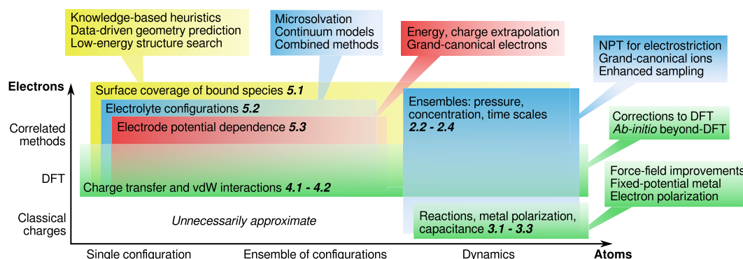
Figure 1. Approximations in computational electrochemistry organized by electronic structure accuracy (y axis) and degree of atomic-configuration sampling (x axis), consequent considerations for accuracy (sticky notes with review section numbers), and typical solutions (call-out boxes). The gradient across a sticky note indicates where each accuracy consideration is most important. The gradient across a sticky note indicates where each accuracy consideration is most important.
