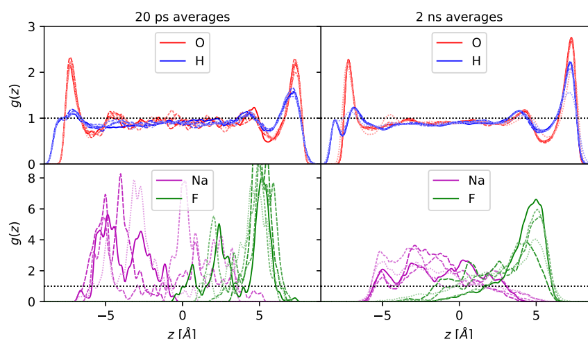
Figure 3. Water and ion density profiles from classical MD simulation of an aqueous 1 M NaF electrolyte in a 10 \times 10 \times 20 \text{ Å}^3 simulation cell typical for AIMD (contains 54 water molecules and 1 ion pair) between Ag(100) electrodes charged to \pm 10 \mu\text{C}/\text{cm}^2 (full cell, as in Figure 2a). Left panels show results averaged over five sequential 20 ps segments typically feasible in AIMD, while the right panels show averages over 2 ns segments from the same initial configuration (each averaged over 500 equally spaced configurations). The dotted lines at 1 correspond to bulk densities. Ion profiles do not spread out sufficiently to form a diffuse layer even in such a small cell until nanosecond time scales.
