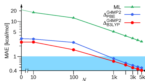
Figure 10. Mean absolute error (MAE) in atomization energies of molecules from machine learned (ML) models compared to a beyond-DFT method (G4MP2) as a function of number of molecules, N , in the training set reduces drastically when the model is trained to the difference \Delta_{G4MP2}^{DFT} between DFT (either PBE or B3LYP) and the beyond-DFT method. 150 Such \Delta -learning approaches allow beyond-DFT accuracy at DFT cost with far fewer expensive beyond-DFT calculations. Adapted with permission from ref 150. Copyright 2015 American Chemical Society.)
