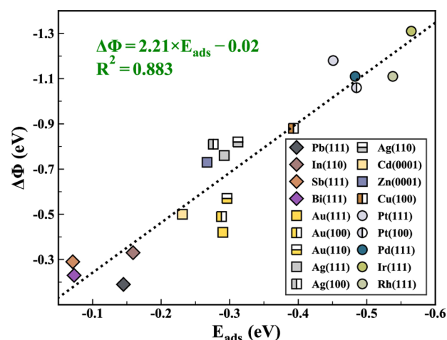
Figure 14. Difference between the PZC and work function ( \Delta\Phi ) from experiment as a function of the adsorption energy for water on metal surfaces calculated with AIMD. Surfaces include sp (diamonds), sd (squares), d (circles) metals. Adapted with permission from ref 229. Copyright 2021 American Chemical Society.
