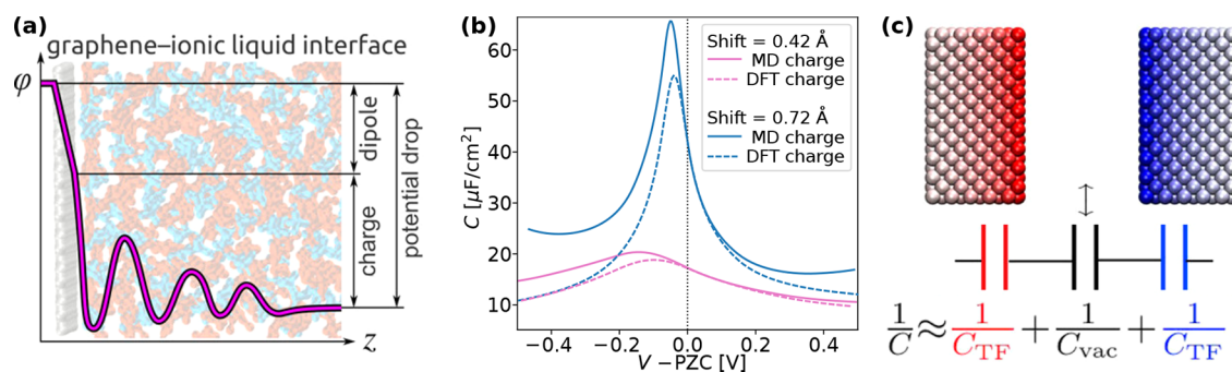
Figure 9. Underestimation of electrochemical capacitance by classical MD can be fixed by (a) a dipole correction that accounts for the electronic induced charge distribution, 114 or equivalently, (b) a shift of the electrode charge density toward the electrolyte. 21,115 (c) Additionally, a semiclassical Thomas–Fermi model can approximately incorporate electronic screening of the electrode to decrease the overall capacitance for electrodes that are not perfect conductors. 117 (a) Adapted with permission from ref 114. Copyright 2020 American Chemical Society. (b) Adapted with permission from ref 21. Copyright 2022 AIP Publishing. (c) Adapted with permission from ref 117. Copyright 2020 AIP Publishing.
