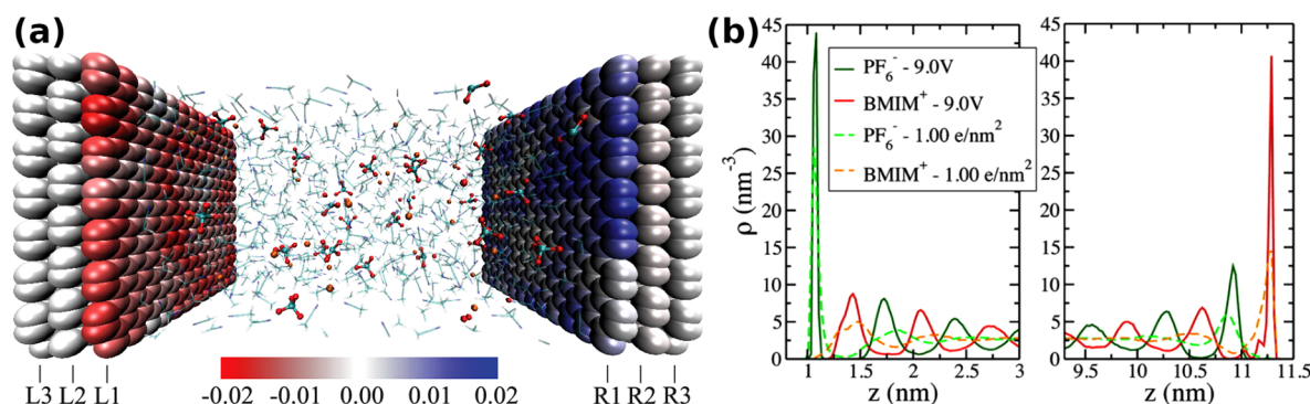
Figure 6. (a) Fixed-potential MD simulations capture localized induced-charge response of the metal electrode, 85 causing (b) an increased effective attraction of charged electrolyte species to the electrode, leading to substantial differences in ion distributions next to the electrode. 86 (a) Reproduced with permission from ref 85. Copyright 2014 AIP Publishing. (b) Adapted with permission from ref 86. Copyright 2013 American Chemical Society.
