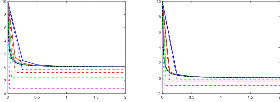
FIG. 1. The solution of u' = -10u^2 for the DIRK (dashed lines) and SSP-iMDRK (solid lines) compared to the correct solution (dash-dot line) for \Delta t = \frac{1}{n} where n = 4, 8, 16, 32, 64 in blue, red, green, magenta, and cyan, respectively. We see that if \Delta t is not small enough the qualitative behavior of the numerical solution using the DIRK methods is poor. However, the SSP-iMDRK methods converge to a solution that is qualitatively correct for all values of \Delta t tested. Left: second order methods. Right: third order methods.
