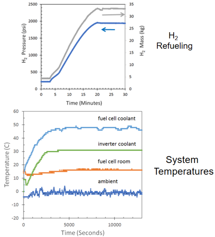
Figure 5: Test data logged during the outside MarFC test. (Top) H 2 refueling rate data; (Bottom) MarFC system temperatures during operation.
