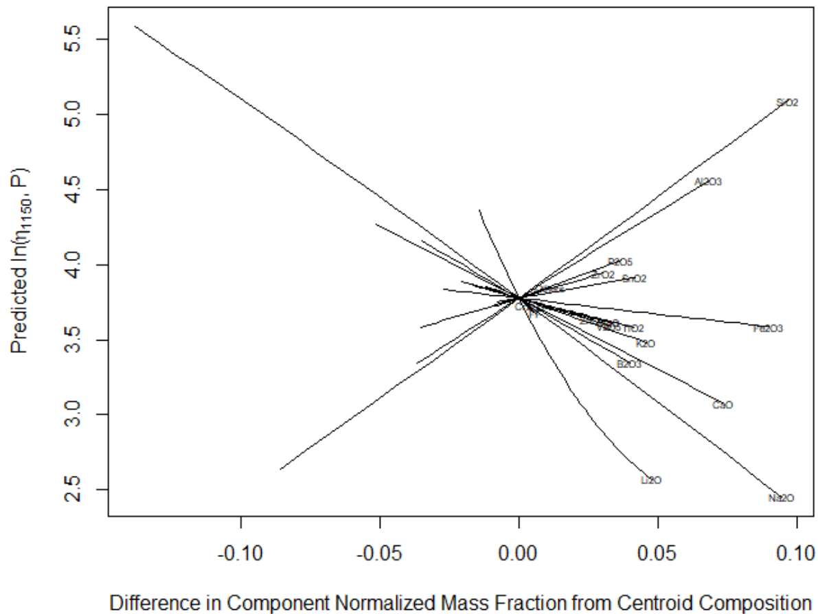
Figure 5.16. Response Trace Plot for 21-Term Reduced Partial Quadratic Mixture Model on the Natural Logarithm of Viscosity at 1150 °C for LAW Glasses
