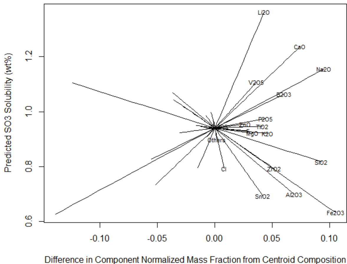
Figure 7.8. Response Trace Plot for the 19-Component Full Linear Mixture Model on Melter \text{SO}_3 Tolerance at 1150 °C for LAW Glasses
