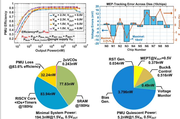
Figure 13.8.5: Measured PMU efficiency versus P_{OUT} across different V_{IN} and V_{OUT} and measured MEPT voltage and energy per cycle errors across 10 chips (top); measured SoC system power breakdown at 180Hz and measured PMU quiescent power breakdown at V_{IN} = 1.5V and V_{OUT} = 0.5V (bottom).
