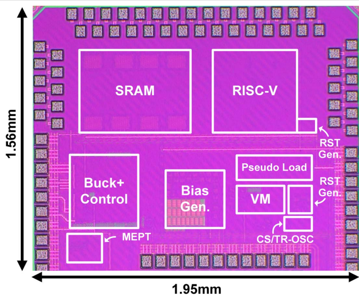
Figure 13.8.7: Die micrograph of the ULP IoT SoC.
