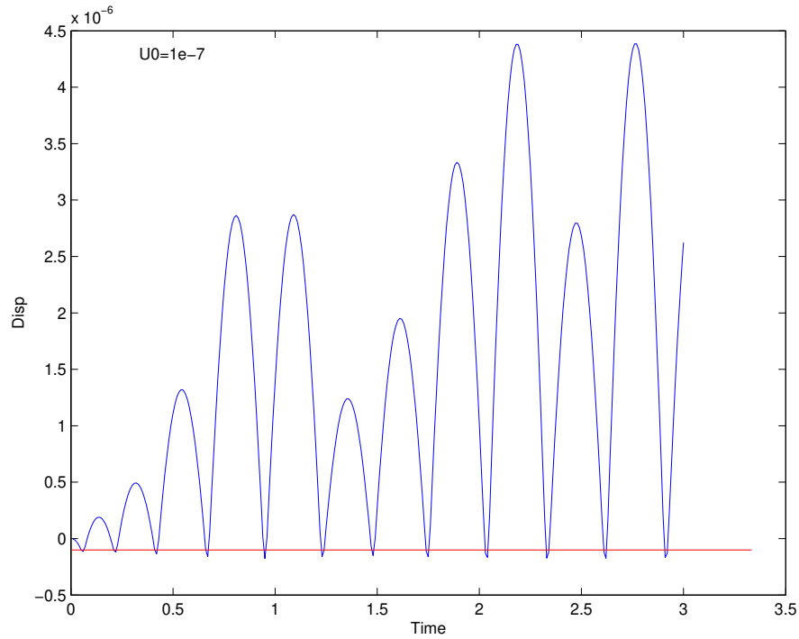
Figure 5-47. – Mass bouncing off a Gap. With this large time step the model is not conserving energy. Reducing the time step is required to correct the problem.
