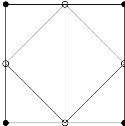
Figure 5-27. – Quad8T Element.
