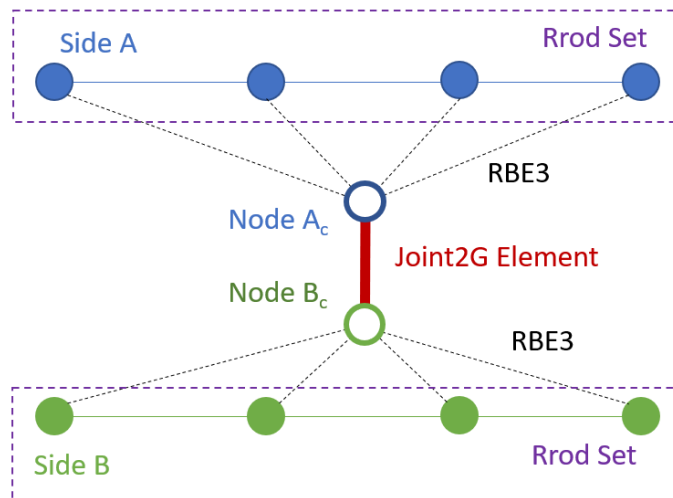
Figure 5-56. – Construction of tied joint with side=Rrod.
