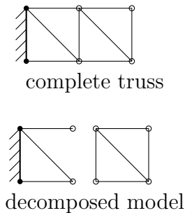
Figure 1-2. – Truss Decomposition Issues.
