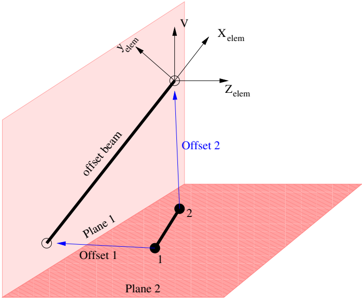
Figure 5-37. – Nbeam Orientation, Offset and Local Coordinate System. The coordinate system is in the plane of the offset beam. The plane is defined by the offset beam and the orientation vector, \vec{V} .
