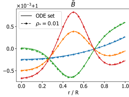
FIG. 2. Comparison between equation (25) and MITNS solution for the dimensionless magnetic field, for the same cases presented in Figure 1, using \tilde{v}_A^2 = 1000 .
