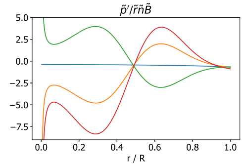
FIG. 4. ODE set calculated dimensionless diamagnetic angular velocity.
