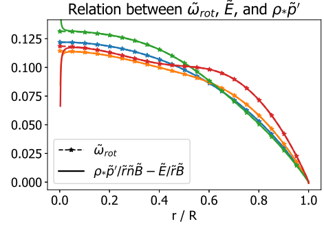
FIG. 5. Comparison between \tilde{\omega}_{rot} , electric field and the pressure gradient terms from equation (60), as calculated by MITNS for the same cases presented in Figure 1.
