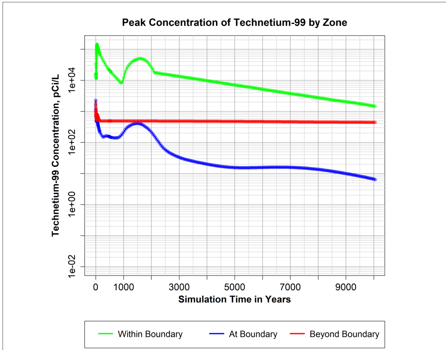
Figure C-22. Peak Concentration of Technetium-99 from the Start of Simulation to the end of the Simulation Within, At, and Beyond the Compliance Boundary Assuming the Best Estimate Initial Concentration
