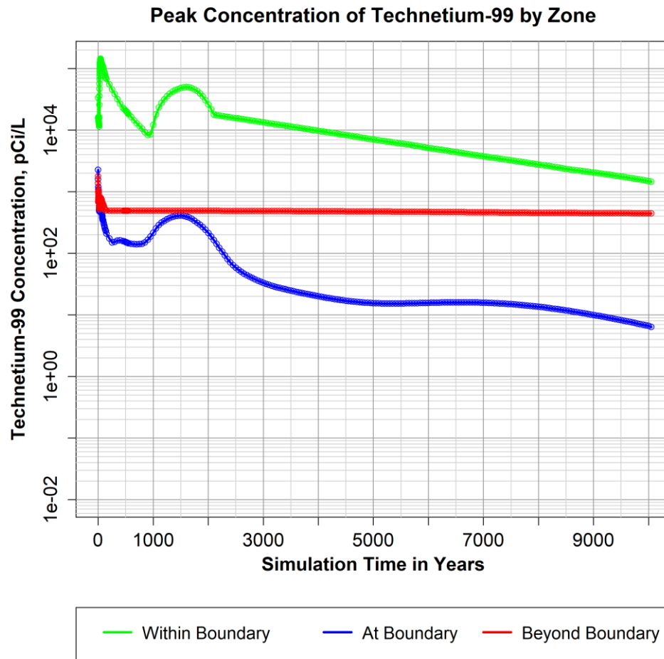
Figure 8. Peak Concentration of Technetium-99 from the Start of Simulation to the End of the Simulation Within, At, and Beyond the Compliance Boundary Assuming the Best Estimate Initial Concentration
