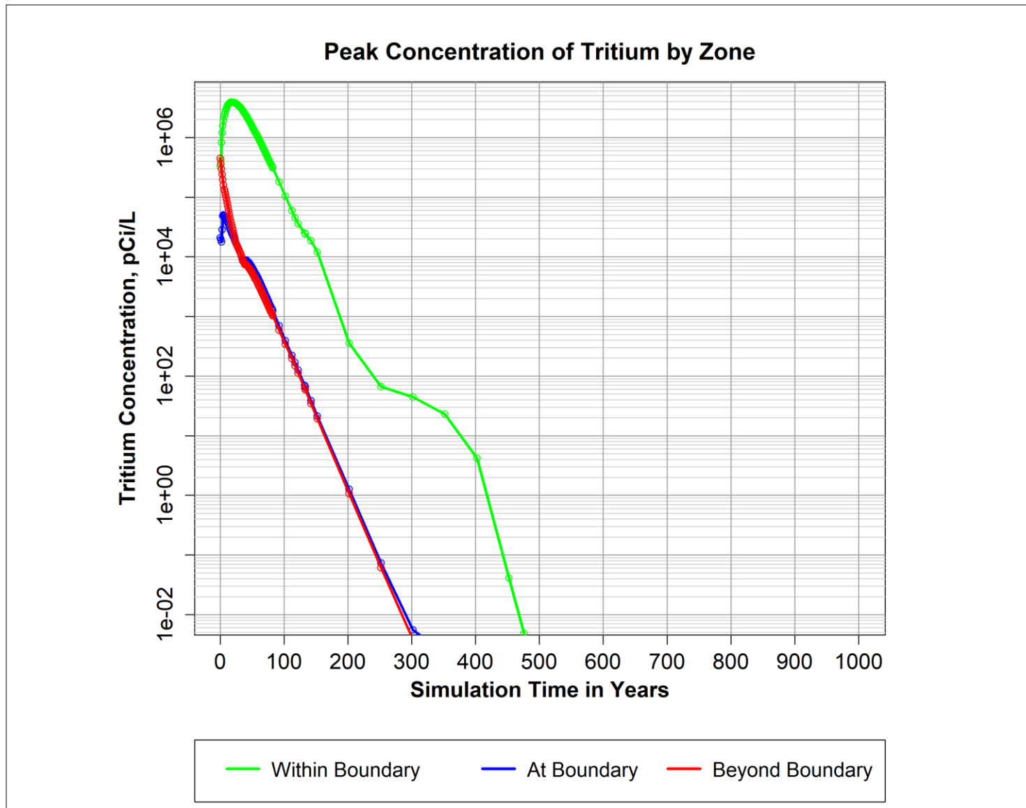
Figure C-32. Peak Concentration of Tritium from the Start of Simulation Until the End of the Compliance Period Within, At, and Beyond the Compliance Boundary Assuming the Best Estimate Initial Concentration
