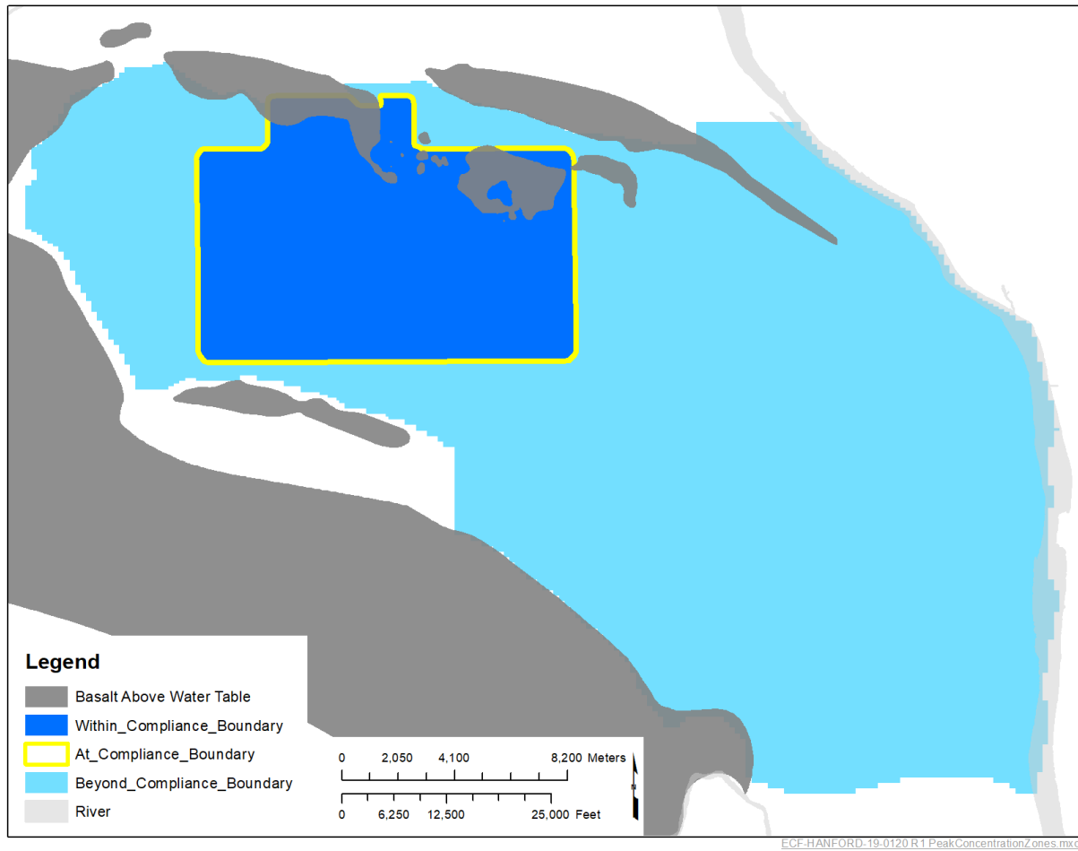
Figure 6. P2R Version 8.3 Peak Concentration Summary Zonation Extents
