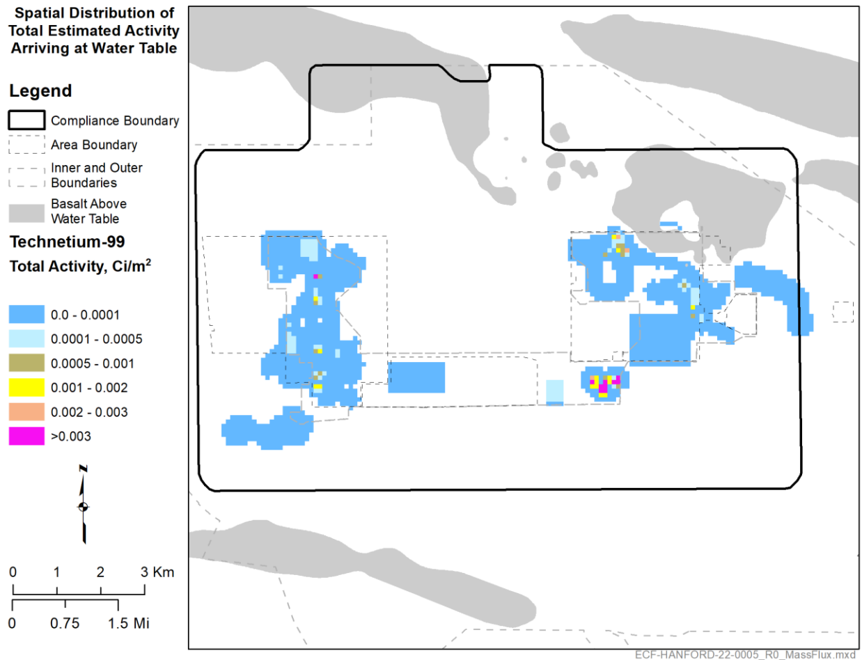
Figure 2. Spatial Distribution of Simulated Activity Entering the Saturated Zone from the Vadose Zone for Technetium-99 over the Entire Length of Simulation Temporal Discretization
