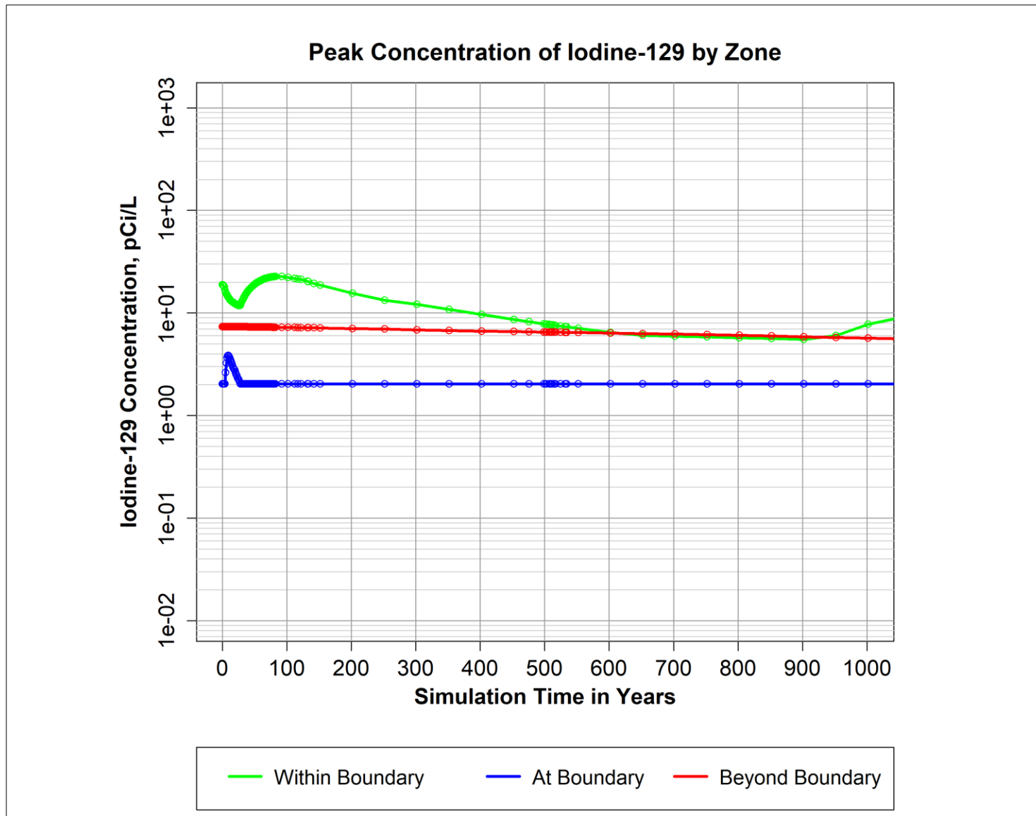
Figure C-10. Peak Concentration of Iodine-129 from the Start of Simulation Until the End of the Compliance Period Within, At, and Beyond the Compliance Boundary Assuming the Best Estimate Initial Concentration
