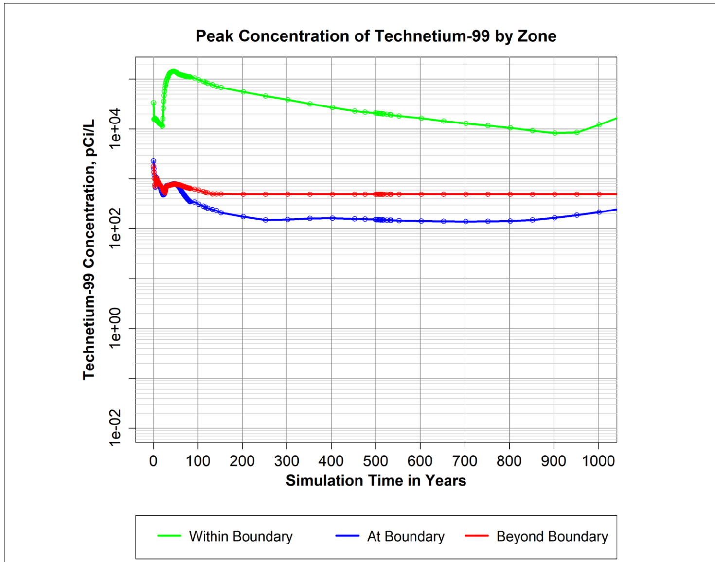
Figure C-21. Peak Concentration of Technetium-99 from the Start of Simulation Until the End of the Compliance Period Within, At, and Beyond the Compliance Boundary Assuming the Best Estimate Initial Concentration
