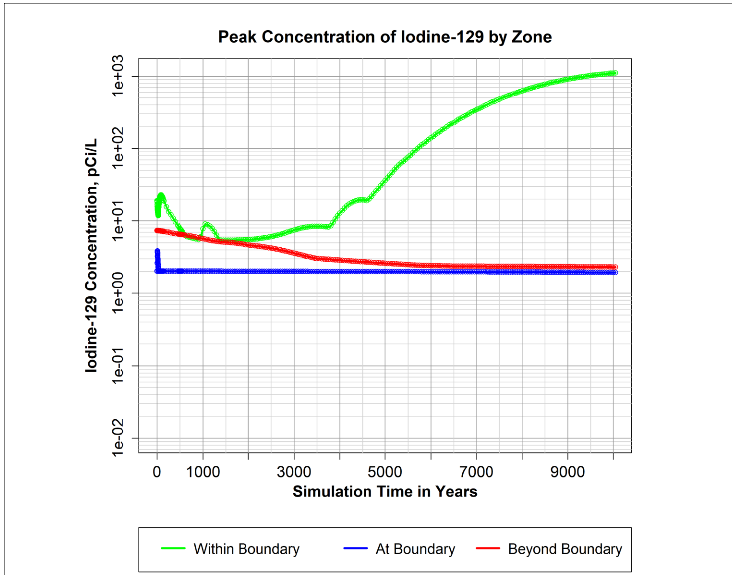
Figure C-11. Peak Concentration of Iodine-129 from the Start of Simulation to the end of the Simulation Within, At, and Beyond the Compliance Boundary Assuming the Best Estimate Initial Concentration
