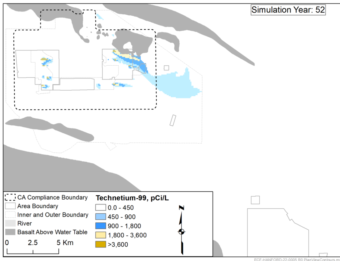
Figure 5. Plan View Contours of the Tc-99 Plume at Simulation Time 52 Years Based on Best Estimate Concentration Initial Conditions
