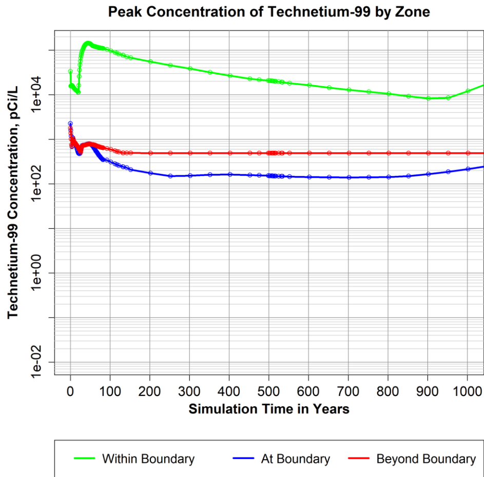
Figure 7. Peak Concentration of Technetium-99 from the Start of Simulation Until the End of the Compliance Period Within, At, and Beyond the Compliance Boundary Assuming the Best Estimate Initial Concentration
