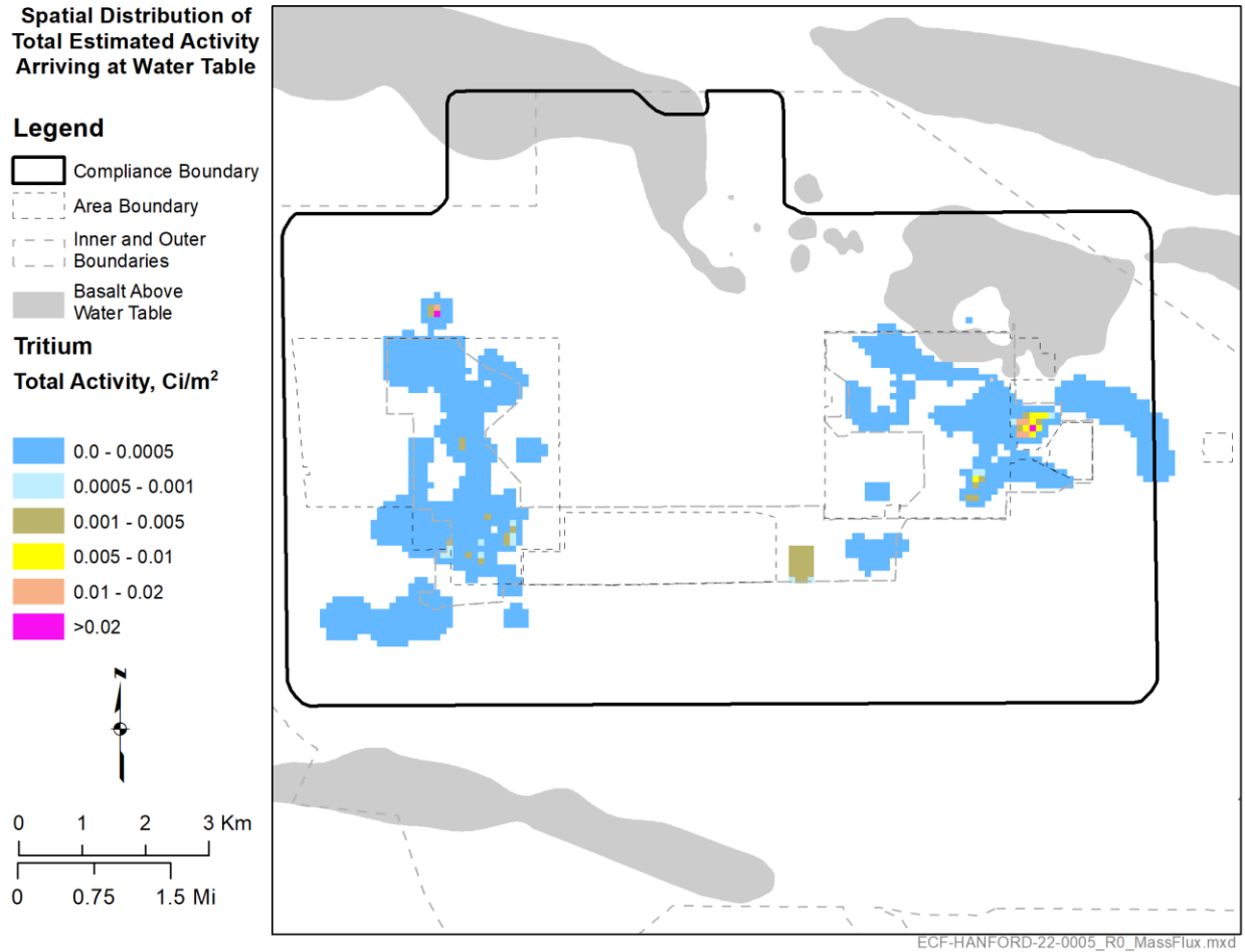
Figure 4. Spatial Distribution of Simulated Activity Entering the Saturated Zone from the Vadose Zone for Tritium over the Entire Length of Simulation Temporal Discretization
