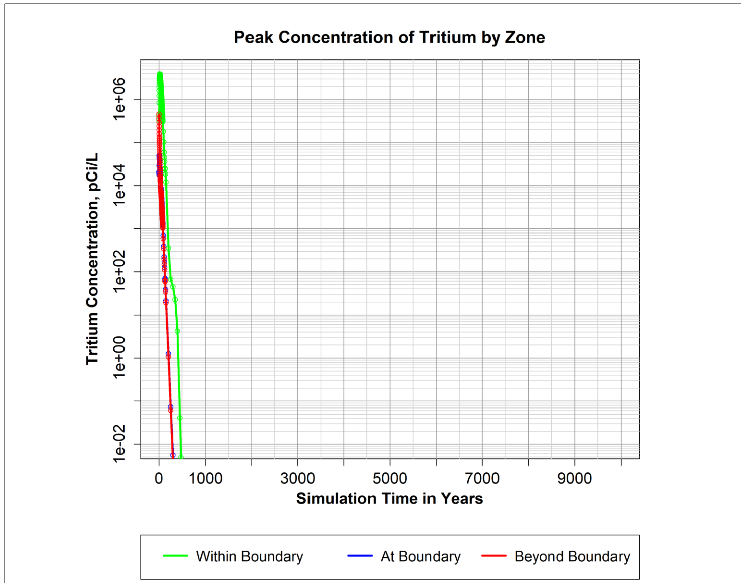
Figure C-33. Peak Concentration of Tritium from the Start of Simulation to the end of the Simulation Within, At, and Beyond the Compliance Boundary Assuming the Best Estimate Initial Concentration
