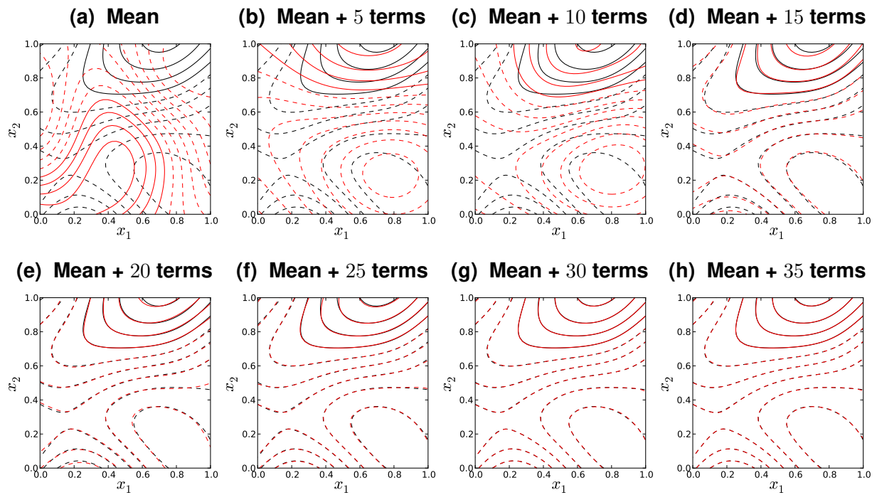
Figure 5-44. Reconstructing 2D realizations with an increasing number of KL expansion terms for c_l = 0.5
