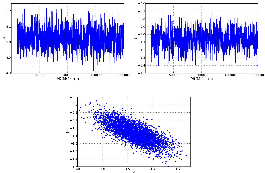
Figure 5-21. MCMC chains for parameters a and b , as well as a scatter plot for a and b
