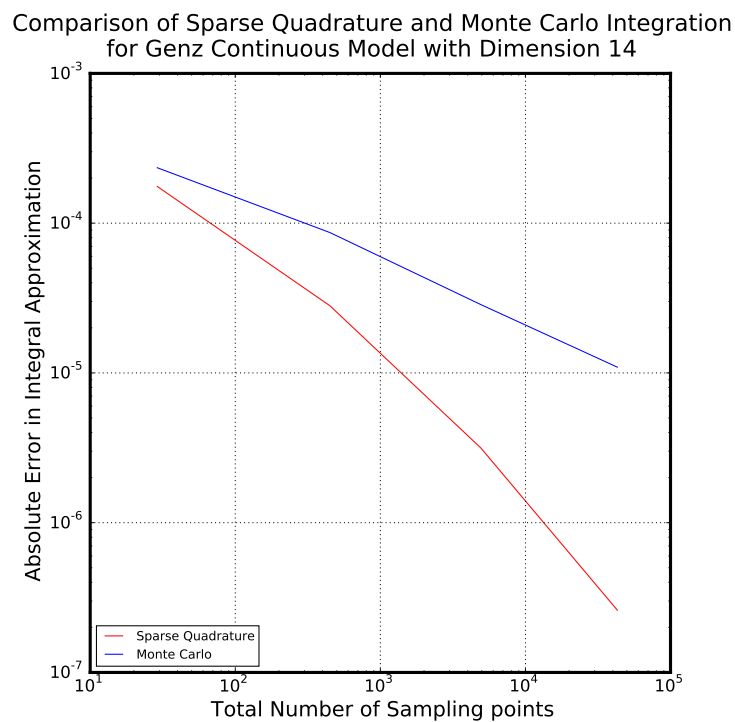
Figure 5-10. Samples results of sparse_quad.py
