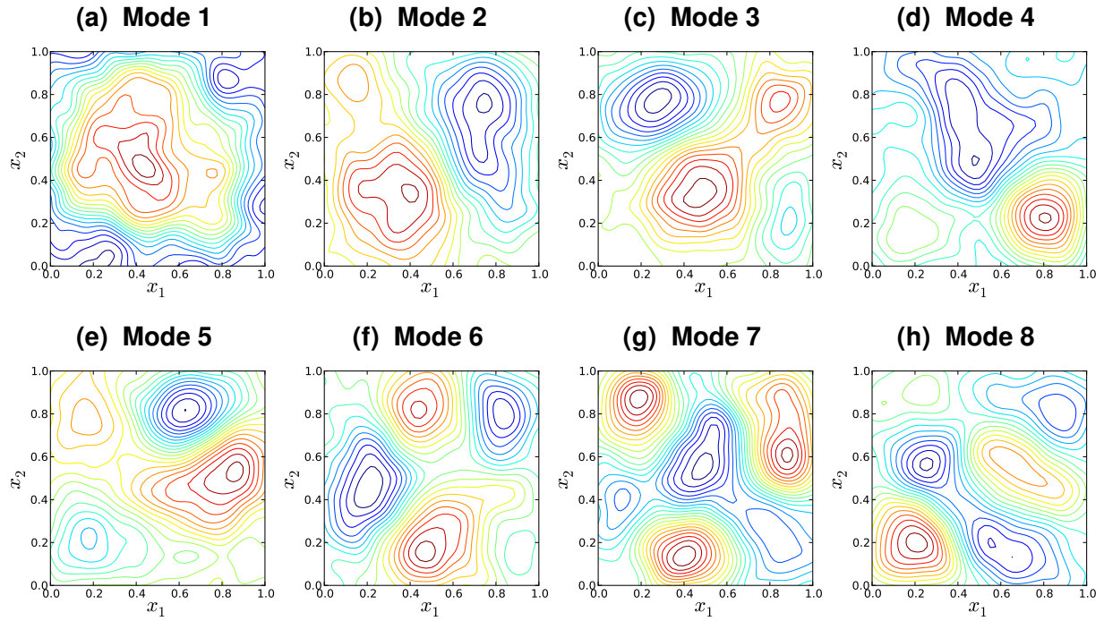
Figure 5-40. Illustration of first 8 KL modes, computed based on a numerical covariance matrix estimated using 2^{12} 2D RF realizations with c_l = 0.1
