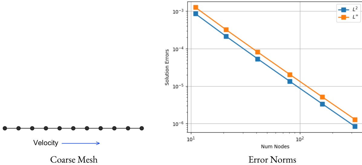
Figure 3.8-1.. Steady Advection Conduction: 3D Bar2 Meshes
