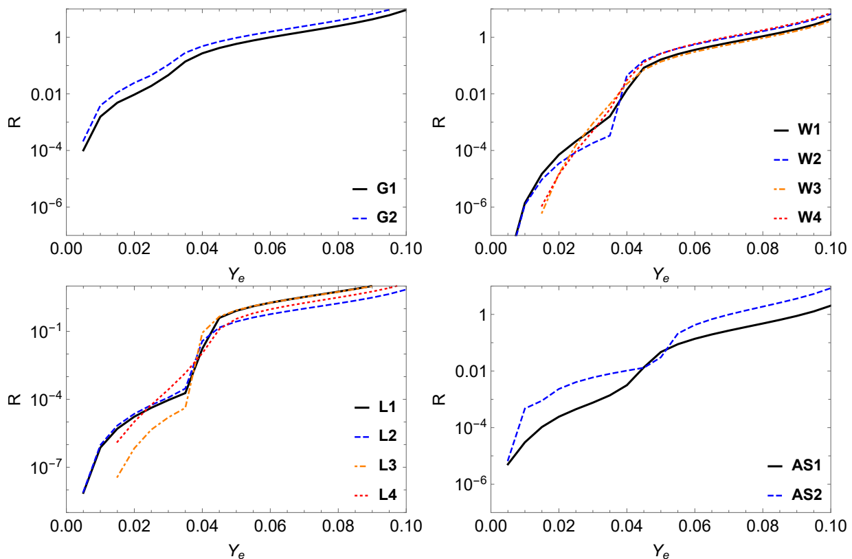
FIG. 8: The factor R as a function of Y_e in gnocchi (upper left), waffle (upper right), lasagna (lower left) and anti-spaghetti (lower right).
