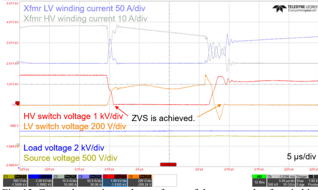
Fig. 13. Zoomed experimental waveforms of the proposed soft-switching solid-state transformer (S4T) to verify the ZVS and the controlled dv/dt.
