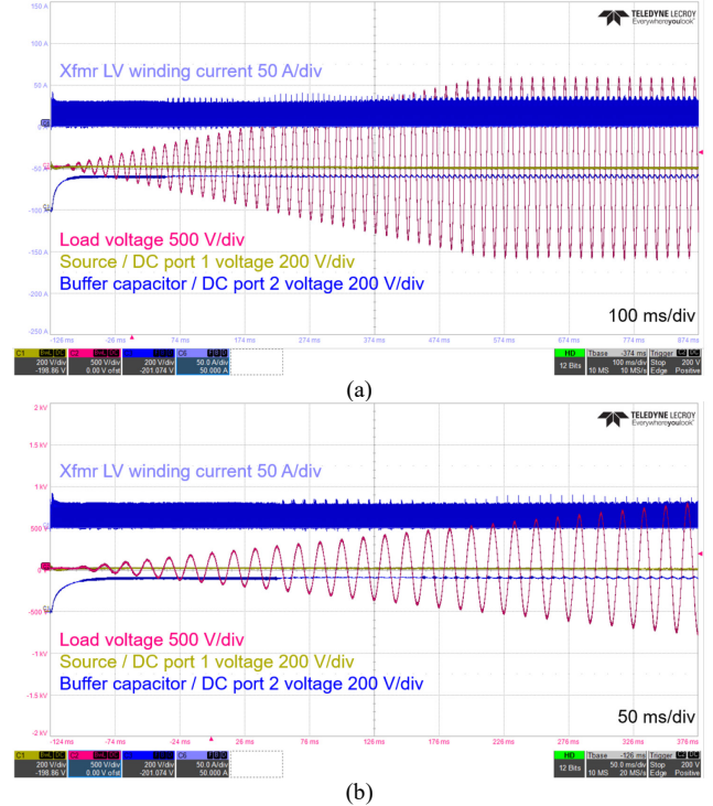
Fig. 15. (a) Experimental waveforms of the proposed soft-switching solid-state transformer (S4T) during dynamic voltage ramp-up. The staircase-like shape on the load-voltage waveform is due to the oscilloscope resolution, which is in fact smooth as shown in the zoomed version. (b) Zoomed output-voltage level.
