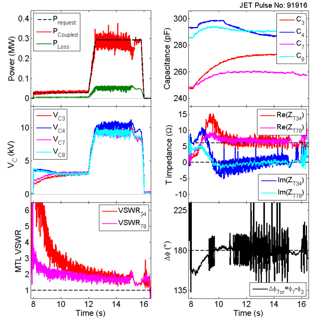
Fig. 2. Example of feedback control on a JET pulse (bottom half array operation). Top left: power request, coupled power and power losses. Middle left: capacitor voltages. Top right: capacitor values actuated by the first stage matching to achieve the requested Z_T = 6 + 0j \Omega (middle right graph). Bottom left: the SSM actuates the SSM stub and trombones to bring the MTL VSWR down towards an offset matched condition. Bottom right: the toroidal phase feedback actuates the MTL trombones to obtain the requested toroidal phasing (dipole phasing – 180° in this case).
