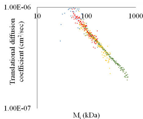
Figure 9. Diffusion coefficient vs molecular weight ( M_i ) for: L1.1 (red), L2.2 (green), C3.1 (dark blue) and C4.1 (orange).
