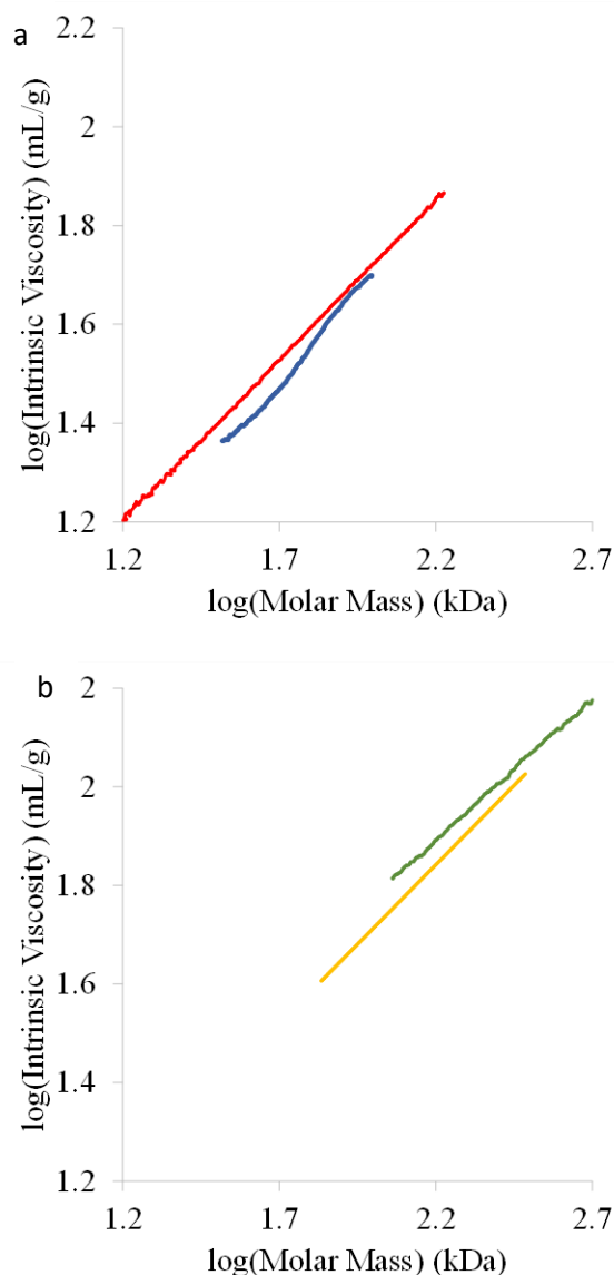
Figure 8. MHS plots of cyclic and linear polyDODTs: L1.1 (red) - C3.1 (dark blue) (a) and L2.2 (green) - C4.1 (orange) (b).
