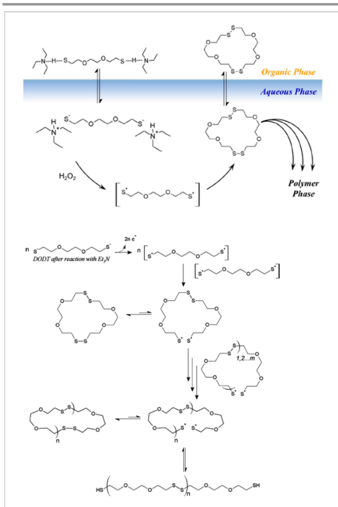
Figure 1. Proposed mechanism of R3P of DODT. The organic phase is TEA/monomer, a clear oily liquid. Reproduced with permission from. 8
