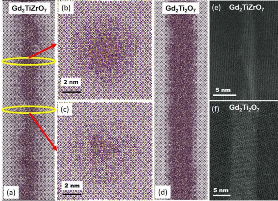
Figure 21: (a-d) MD simulations and (e,f) TEM images of tracks in Gd_2TiZrO_7 and Gd_2Ti_2O_7 pyrochlores irradiated with 2.3 GeV Pb ions. Details of the damage morphology change with slight variation of the chemical composition. Figure is reprinted from [183].
