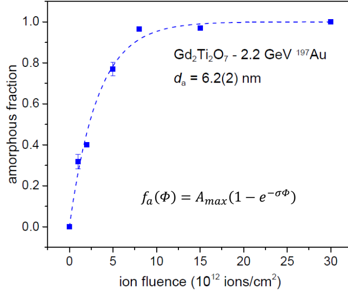
Figure 6: Typical evolution of damage (here amorphous fraction f_a ) as a function of fluence \phi . To analyze the damage cross section \sigma , the data are fit by a direct impact model (each ion produces an amorphous track) based on an exponential function which considers the effect of overlapping tracks. By assuming cylindrical symmetry one obtains the amorphous track diameter d_a . Figure has been modified from [137].
