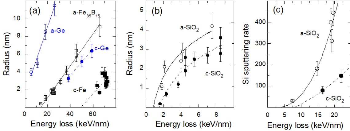
Figure 14: Comparison of amorphous and crystalline materials: track radius versus electronic energy loss of (a) amorphous \text{Fe}_{85}\text{B}_{15} [5] and crystalline Fe [189] irradiated with 10 MeV/u ions and amorphous (a-Ge) [218] and crystalline (c-Ge) Ge [212] irradiated with 1 MeV/u and 0.05 MeV/u ions, respectively, (b) vitreous (a- \text{SiO}_2 ) [180] and crystalline (c- \text{SiO}_2 ) \text{SiO}_2 [160] irradiated with 1 MeV/u ions, and (c) sputtering rate for a- \text{SiO}_2 [219] and c- \text{SiO}_2 [176] for beam energy of 1 MeV/u.
