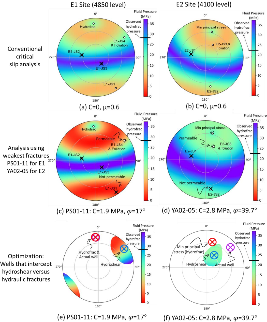
Figure 6. Lower-hemisphere stereoplots of the critical fluid pressure to induce fracture activation (shear or tension) in E1 and E2 site. (a) and (b) shows the conventional critical slip pressure analysis with cohesion of 0 MPa and friction coefficient of 0.6 (Byerlee, 1978) for E1 and E2 site, respectively. Cross symbol means not suitable for hydroshearing. (c) shows the analysis for E1 site assuming the measured weakest fracture strength of PS01-11 with cohesion of 1.9 MPa and friction angle of 17^\circ for all joint sets. (d) shows the analysis for E2 site assuming the measured weakest fracture strength of YA02-05 with cohesion of 2.8 MPa and friction angle of 39.7^\circ for all joint sets. (e) and (f) shows the orientation of the hydraulic fracture, the fracture sets that are best suited for hydroshearing and the actual well placement decision for hydroshearing or hydraulic fracturing in the E1 and E2 sites, respectively. In (e) and (f), color for critical fluid pressure is only shown for orientations within 30^\circ of joint set that the PS01-11 and YA02-05 are sub-parallel to.
