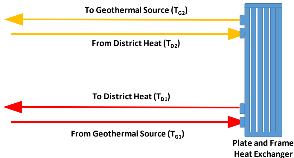
Figure F-3: Primary Heat Exchanger Schematic
