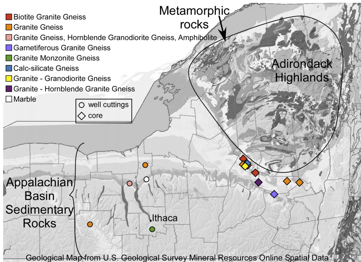
Figure A3: From B. Valentino (2016), map showing the compositions of well cuttings and cores of crystalline basement rocks in New York State.
