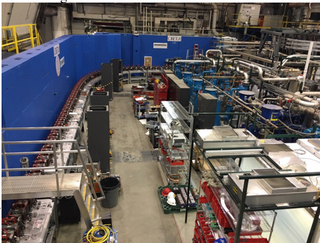
Figure 3: Straight section and the FFA arc of CBETA.
