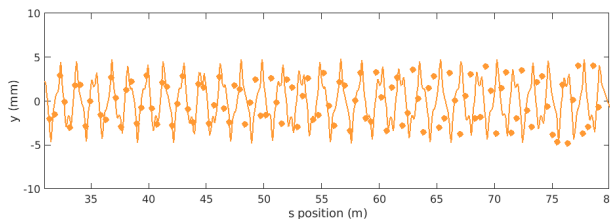
Figure 8: Vertical response results.
