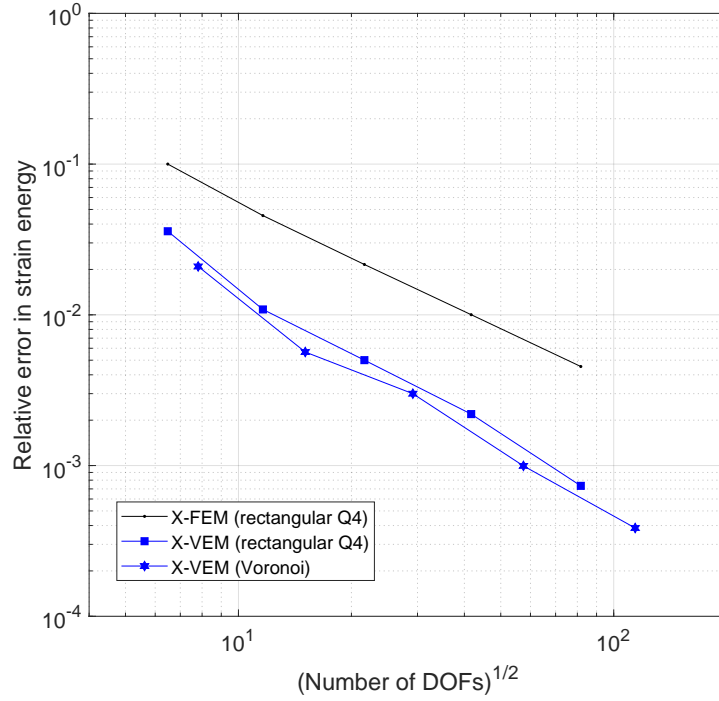
Figure 17: Convergence in terms of relative error in strain energy for the inclined crack problem using \alpha = 1 .
