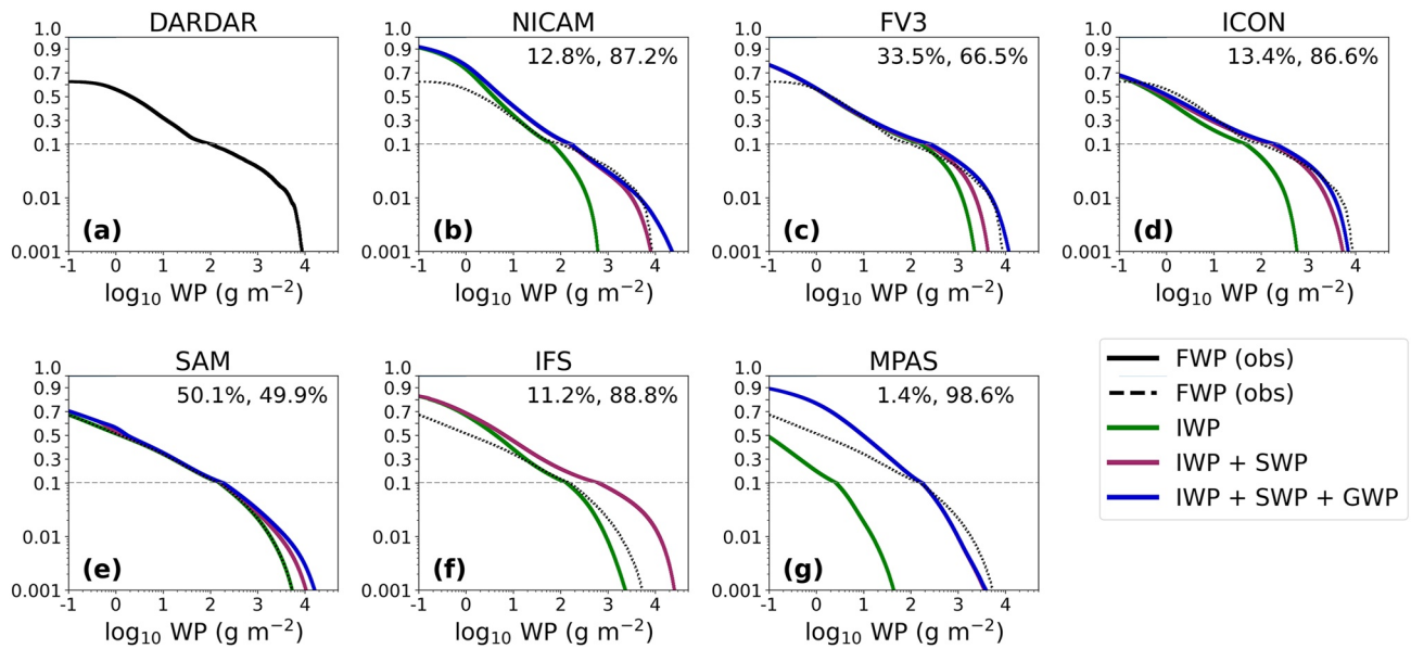
Figure 11. Cumulative distribution functions for ice (IWP; green line), ice + snow (IWP + SWP; pink line), and ice + snow + graupel (IWP + SWP + GWP; blue line) water paths for all models in the Sahel compared to DARDAR frozen water path observations (FWP; solid black line in (a), dashed in (b–g)). Values are accumulated from largest to smallest. ARPNH and UM are omitted because they do not save the 2D output of column-integrated snow or graupel water paths. The y-scale is logarithmic below 0.1 and linear above; the apparent discontinuity at 0.1 is an artifact of this split. The numbers in the upper-right corner of each panel show (left) the percentage of the total FWP from ice and (right) the percentage of total FWP from snow and graupel. These numbers cannot be deduced directly from this figure but are included to emphasize the large contributions of snow and graupel. Again, note that the IFS microphysics scheme does not include graupel.
