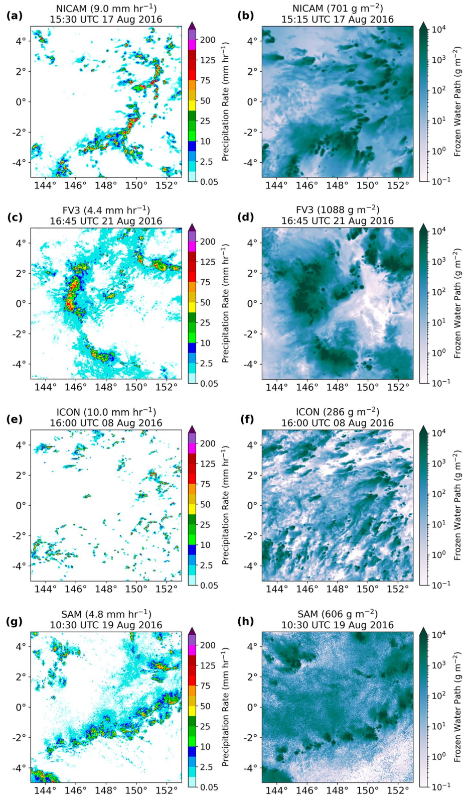
Figure 5. As in Figure 4, but for the TWP.
