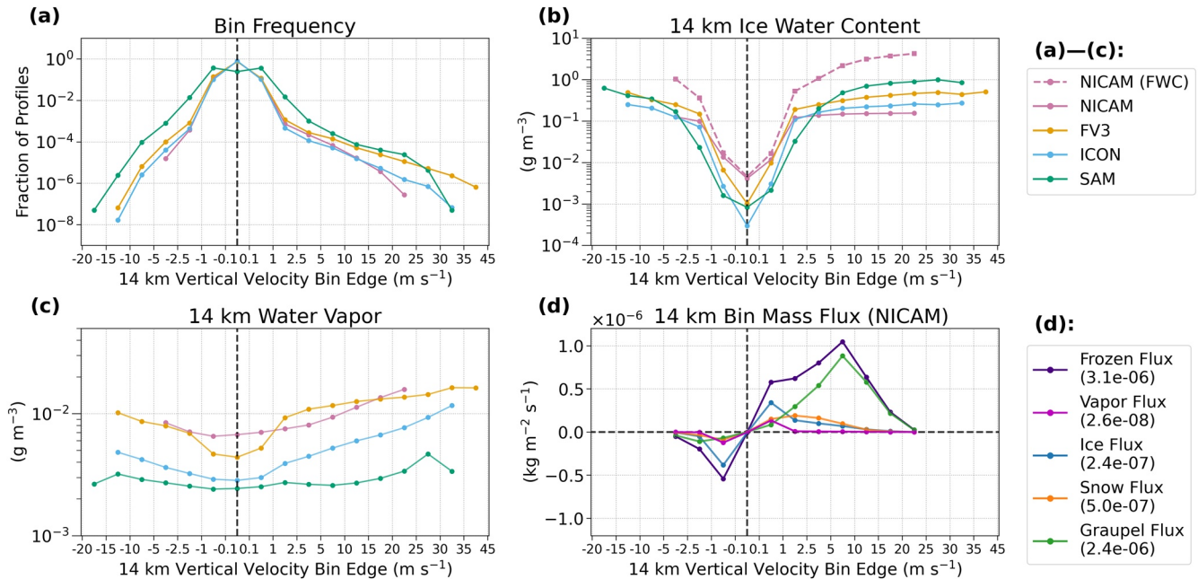
Figure 13. Selected variables sampled at all 14 km grid points for days 3–40 in the Sahel and averaged over vertical velocity bins: (a) bin frequency; (b) cloud ice water content (pink dashed line shows NICAM frozen water content); (c) water vapor content; and (d) frozen water, water vapor, ice, snow, and graupel mass fluxes for NICAM only.
