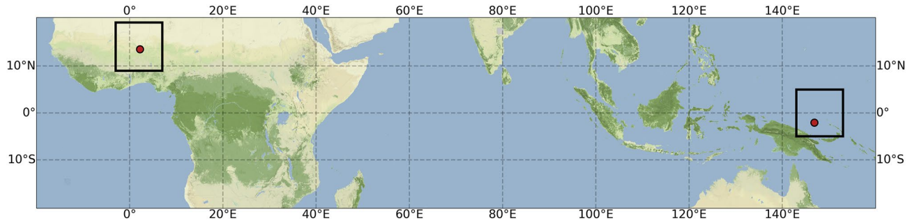
Figure 1. Locations of the analysis regions in (left) the Sahel, 3^{\circ}\text{W} – 7^{\circ}\text{E} , 9^{\circ}\text{N} – 19^{\circ}\text{N} ; and (right) the tropical West Pacific, 143^{\circ}\text{E} – 153^{\circ}\text{E} , 5^{\circ}\text{S} – 5^{\circ}\text{N} . Red dots indicate locations of the (left) AMMA and (right) ARM sites.
