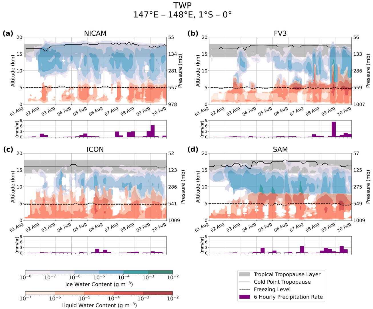
Figure 7. As in Figure 6, but for the TWP. Model output is averaged over a 1^\circ \times 1^\circ box located at 147^\circ\text{E} – 148^\circ\text{E} , 1^\circ\text{S} – 0^\circ , approximately centered over the ARM site in Manus, Papua New Guinea.
