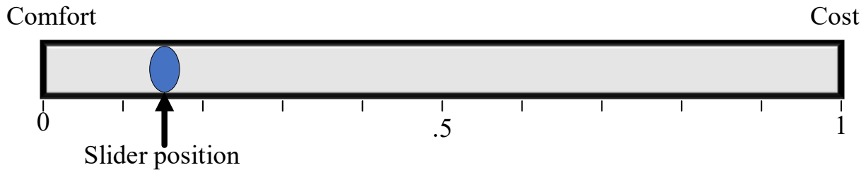
Figure 21. Slider representation.
