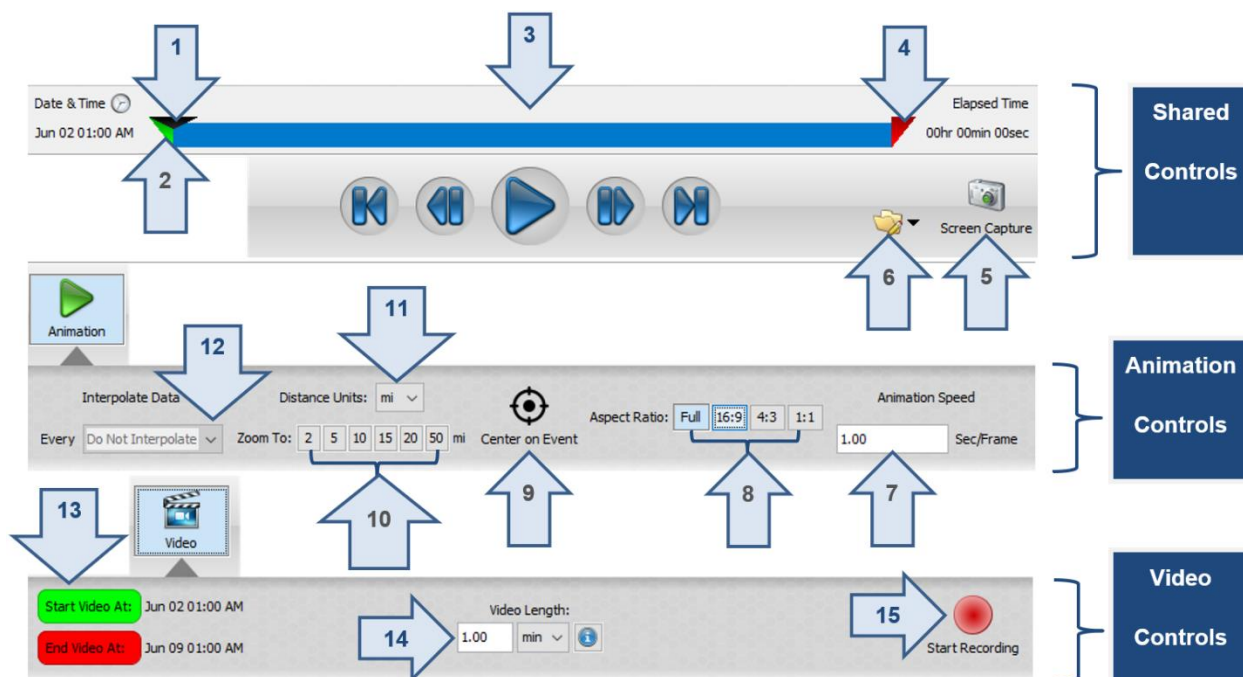
Figure 2-4. Animation/Video Controls
