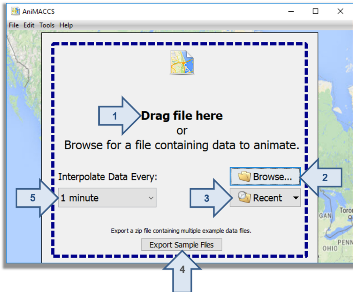
Figure 2-1. Start Screen
