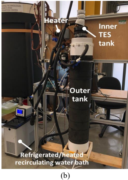
Figure 1. An experimental apparatus for characterizing the performance of a lab-scale DPUTB: (a) schematic and (b) photo.
