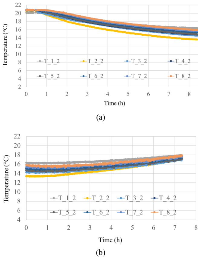
Figure 4. Outer tank temperature during (a) charging test and (b) discharging test.
