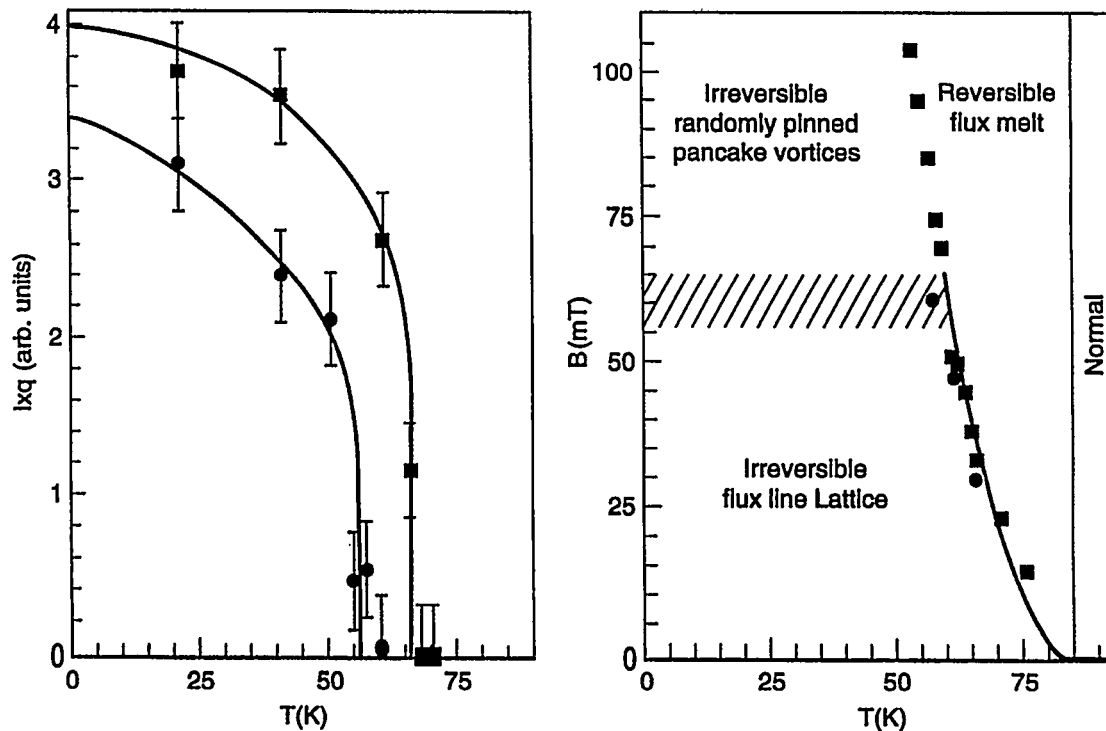
Figure 11. Left: Temperature-dependent neutron diffraction intensity which monitors the melting of the flux (magnetic vortex) lattice in a bismuth-based copper oxide high- T_c superconductor. Data are for 30 mT = 300 gauss (squares) and 60 mT = 600 gauss (circles). Right: Flux lattice-flux liquid phase diagram. Experiments were performed at Risø DR3 (DK) reactor. Figures provided by H. A. Mook (Oak Ridge, U.S.) and T. Forgan (Birmingham, UK).
