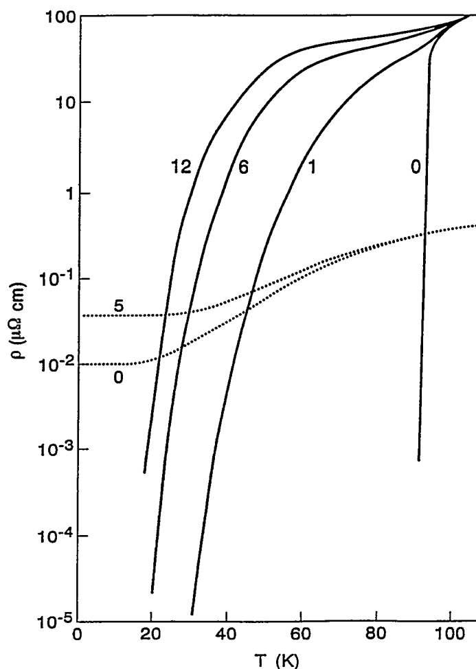
Figure 10. Temperature-dependent resistivity of high- T_c superconductor (solid lines) and elemental copper (dashed lines) in external magnetic fields denominated in kilogauss. Figure provided by D. J. Bishop (AT&T Bell Laboratories, U.S.).
