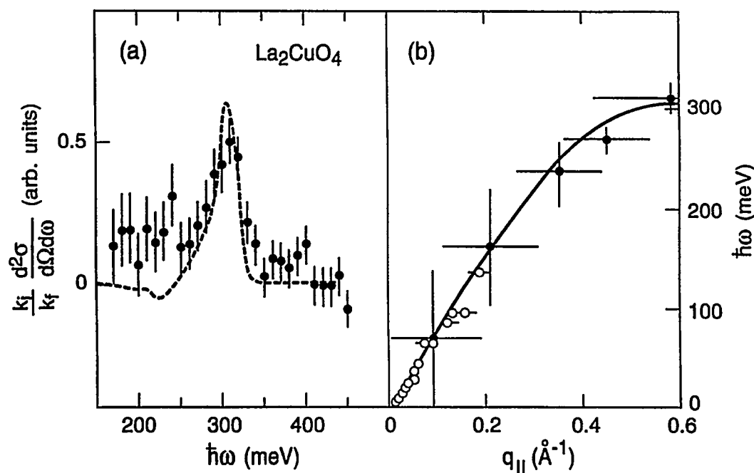
Figure 13. Zone boundary spin wave dispersion relation for antiferromagnetic \text{La}_2\text{CuO}_4 , parent of the high transition temperature superconductors. Spin waves are the magnetic analogs of collective atomic vibrations (phonons) in solids. Data were taken using the HET (High Energy Transfer) instrument of ISIS (filled circles) in the UK, and the IN1 hot source and IN8 thermal spectrometers at the ILL (open circles) in Grenoble, France. Figure provided by S. M. Hayden (Bristol, UK).
