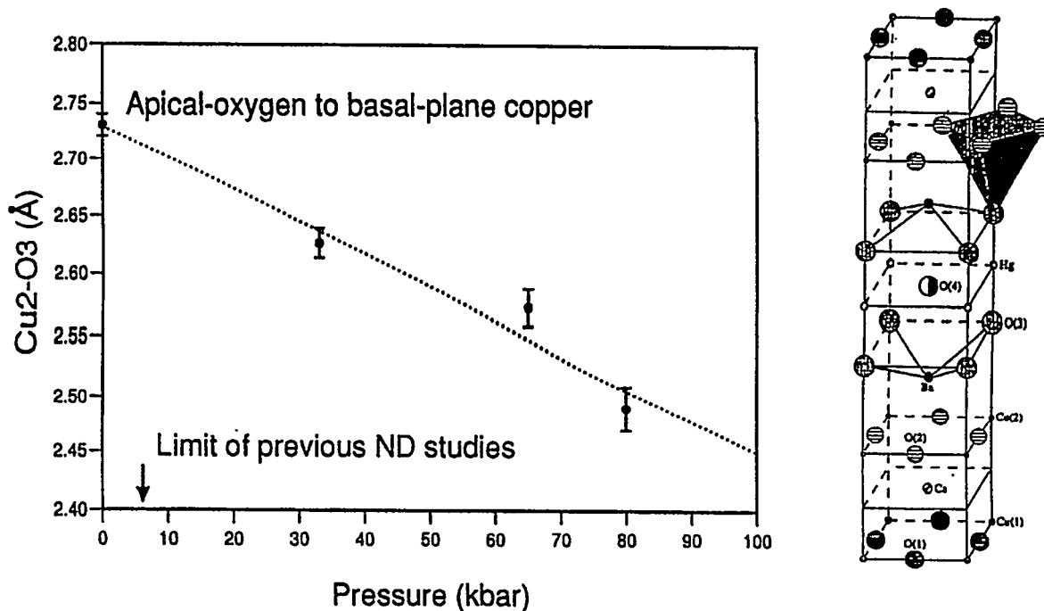
Figure 8. Pressure dependence of distance between apical oxygen and nearest copper atom, which is shortened by 0.25 \text{ \AA} as the superconducting transition temperature rises from 132 \text{ K} \sim (-143^\circ\text{C}) . This material is the mercury-based high- T_c superconductor whose crystal structure is illustrated at right. The apical oxygen is at tip of inverted pyramid and directly opposite the copper atom (small filled sphere) at the center of pyramid base. The experiment was performed at ISIS. Figure provided by W. David (RAL).
