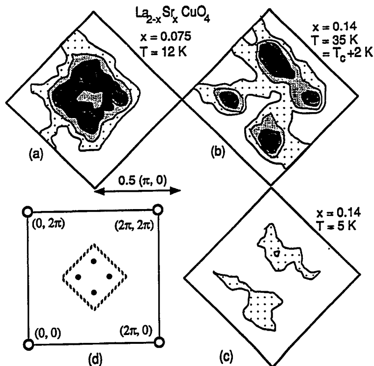
Figure 9. Maps of electronic correlations in \text{La}_{2-x}\text{Sr}_x\text{CuO}_4 for superconducting ( x = 0.14 ) and nonsuperconducting samples ( x = 0.075 ). The hatched diamond in frame (d) shows the region of probed wave numbers relative to the Bragg peak locations. For x = 0.14 (frames b and c), the signal essentially disappears on cooling through the superconducting transition temperature because the carriers pair to form spin singlets which cannot scatter neutrons. Data were collected at Risø DR3 reactor (DK). Figure provided by S. M. Hayden (Bristol, UK).
