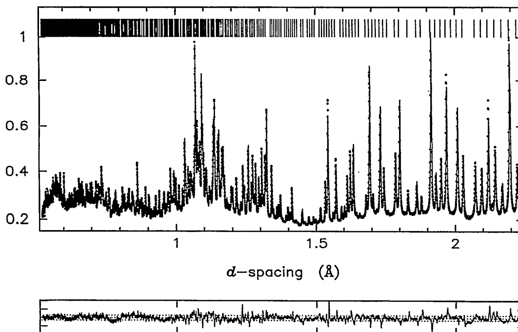
Figure 6. Ultrahigh-resolution powder diffraction pattern collected for C 60 (fullerene) using pulsed spallation source ISIS in UK. Because of the large number of resolved peaks, the atomic positions and thermal parameters can be determined with unprecedented precision. Top frame shows data (circles) and fit to data (line) while bottom frame shows the goodness of fit, as measured by the difference between the data and the fit. Figure provided by W. David (RAL).
