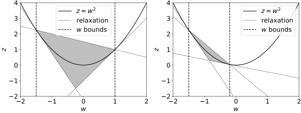
Figure 1: Linear relaxations of z = w^2 with different bounds on w .
