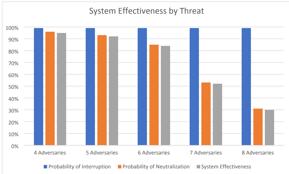
Figure 2 System Effectiveness of The Physical Protection System
