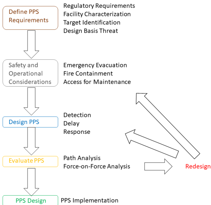
Figure 4 Security-by-Design DEPO 23
