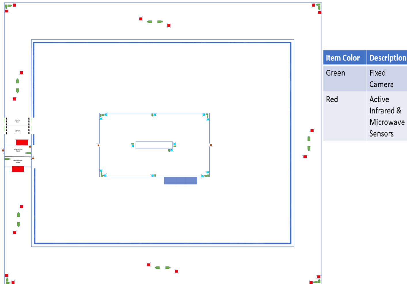
Figure 6 External Physical Protection System
