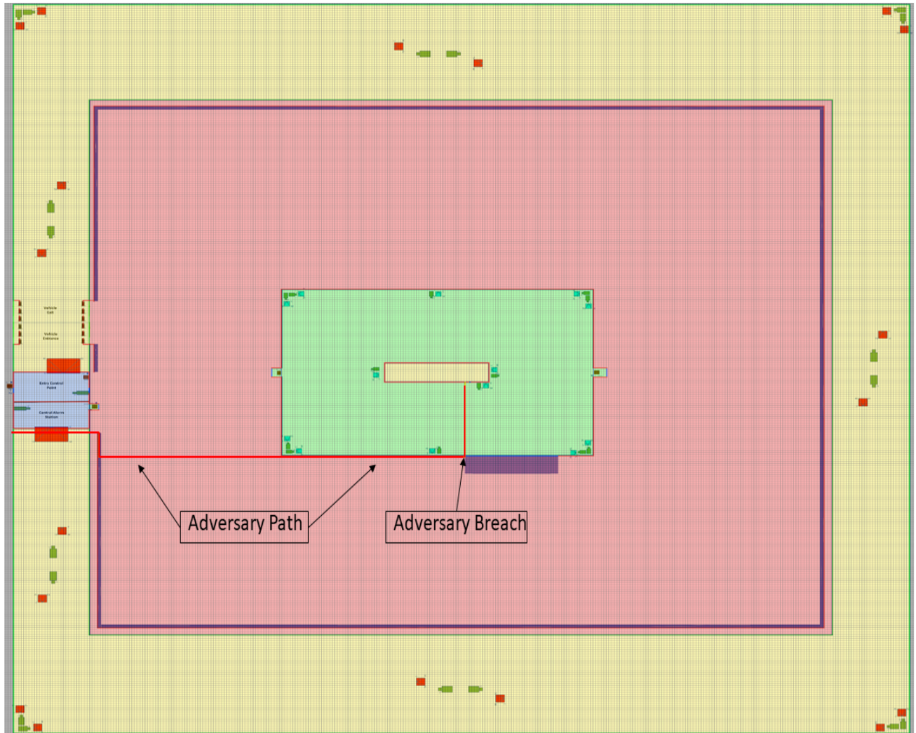
Figure 10 Upgrade One MVP
