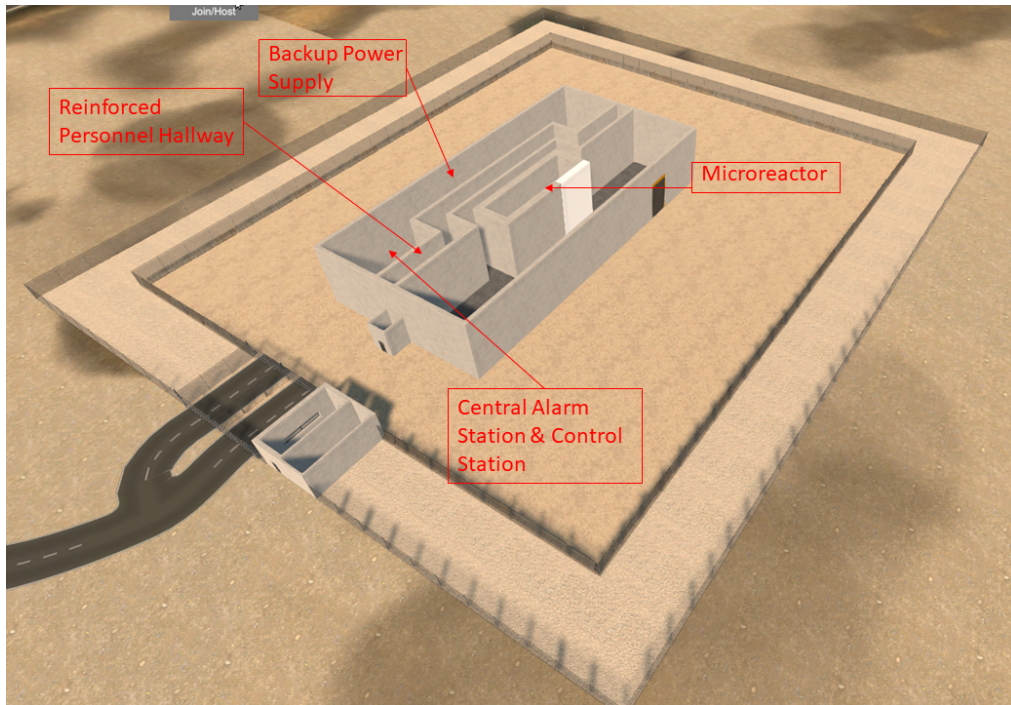
Figure 1 Hypothetical Facility Layout
