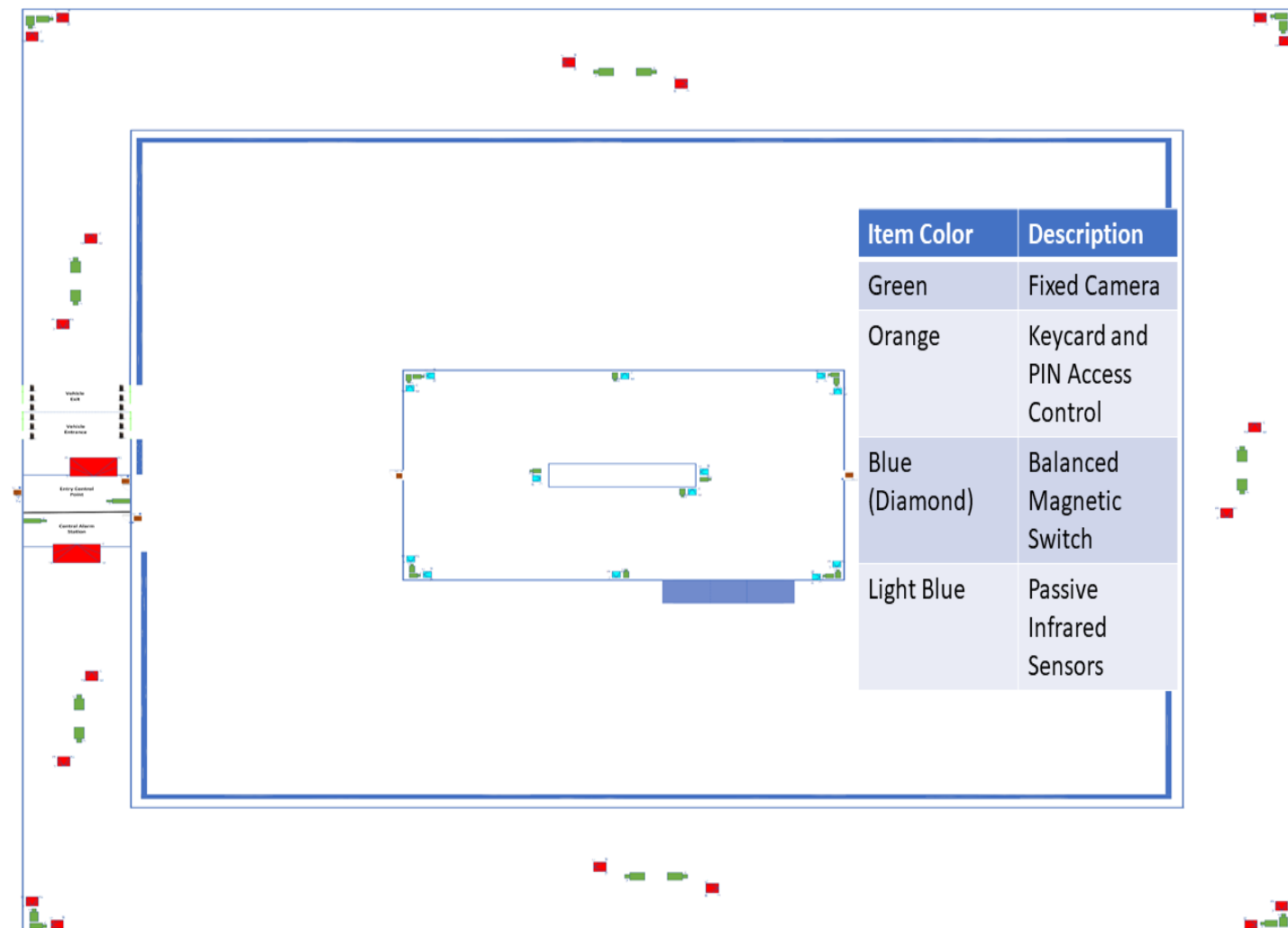
Figure 7 Internal Physical Protection System
