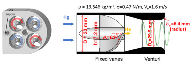
Figure 3: (left) 3D view of the swirl bubblers and the vanes orientations. (right) 2D view of a single swirl bubbler and key parameters.
