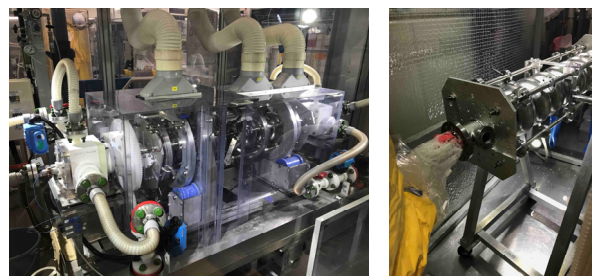
Figure 4: LSF9-1 EP processing (left) and iris brushing (right) at KEK STF.
