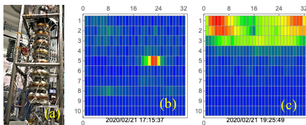
Figure 5: 1622 sensors attached to LSF9-1 (a) and X-ray hot spots captured by Kyoto U sX-mapping system (b, c).
