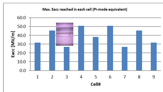
Figure 7: Gradient capability of each cell of LSF9-1. Inset shows the RF surface image of quench location in Cell#3.
