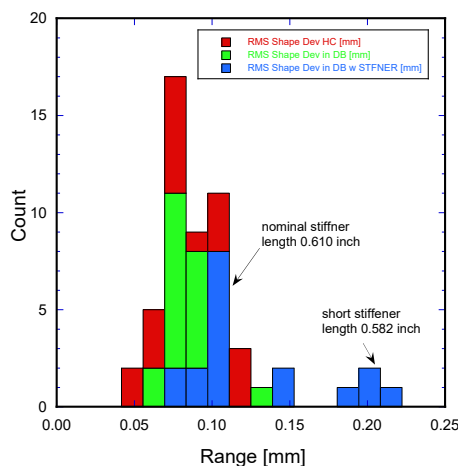
Figure 2. Half-cell shape accuracy statistics.
