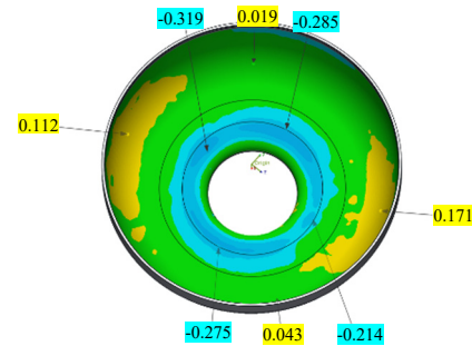
Figure 1. Half-cell C5 shape accuracy measured with a FARO laser scanner. Point deviation in mm.
