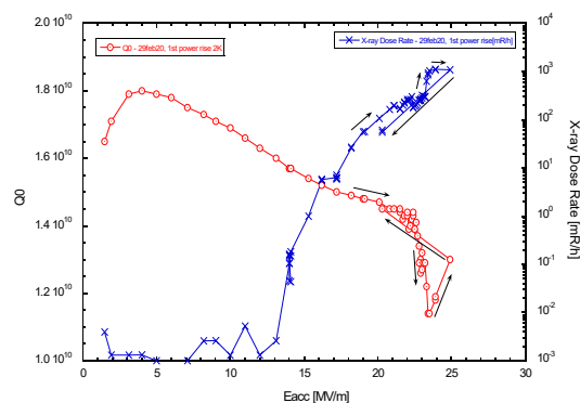
Figure 6: Best \pi -mode performance achieved so far by the cavity LSF9-1 at 2 K.
