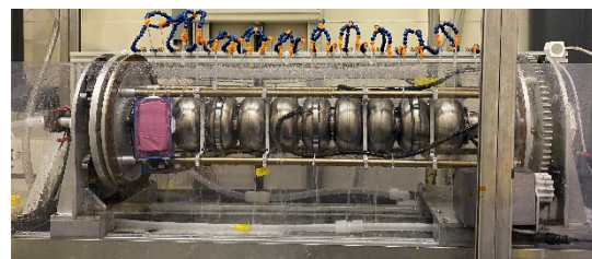
Figure 8: LSF9-1 EP 40 \mu m at joint ANL/FNAL facility.
