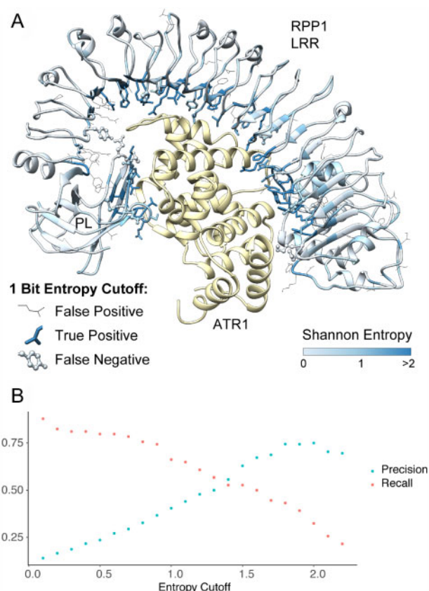
Figure 6 RPP1 contact residues show high sequence diversity. A, Structure of RPP1 LRR-ATR1 complex (PDB ID: 7CRB) colored by entropy scores, with contact residues shown as sticks for predicted true positives and ball and stick for false negatives using a 1 bit entropy cutoff. False positive predictions at the same cutoff are represented as wire. B, Precision and recall for the prediction of RPP1-ATR1 binding site residues based on the choice of entropy cutoff.
