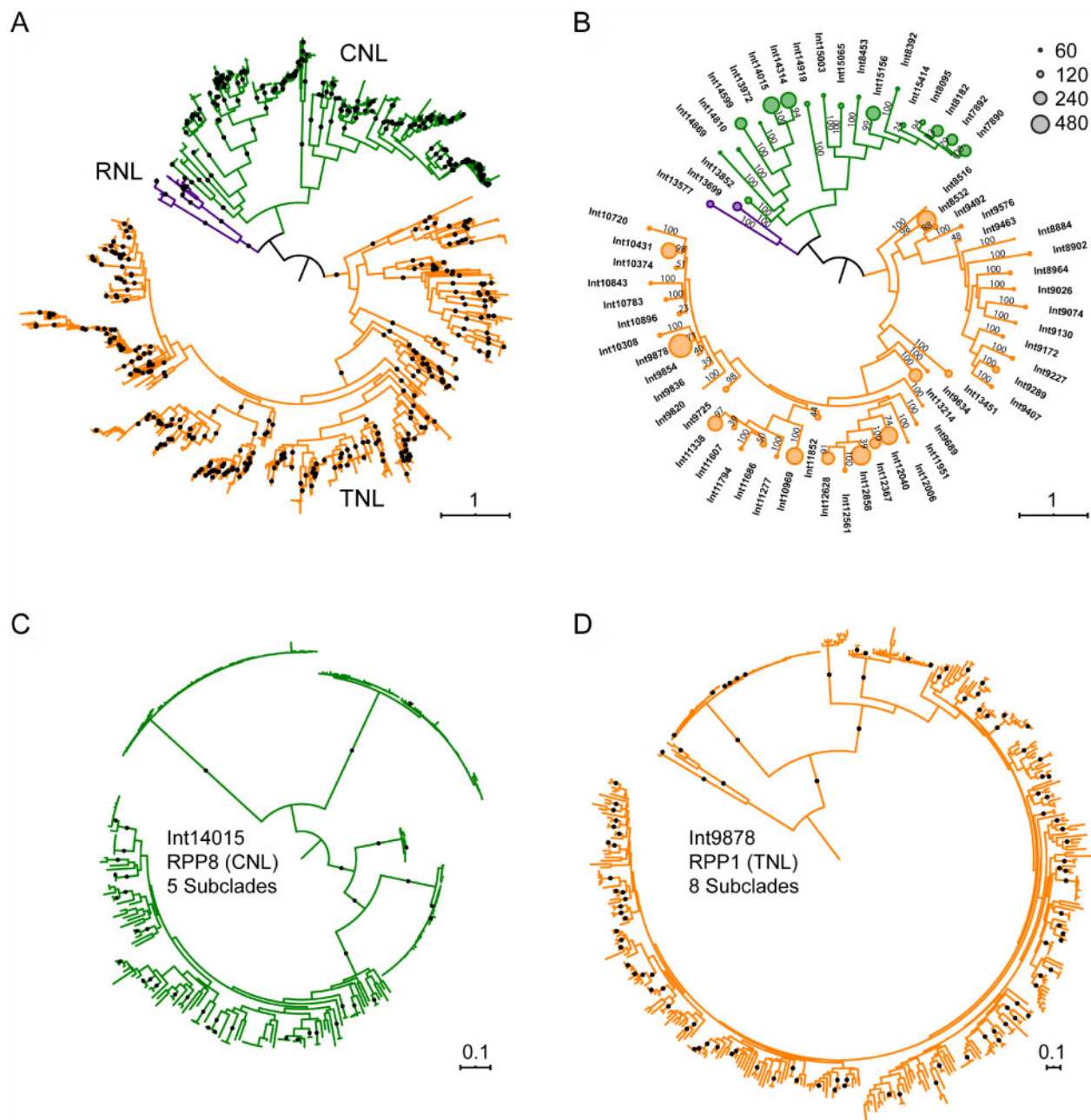
Figure 1 Phylogenetic analyses of Arabidopsis pan-NLRome. A, Maximum likelihood tree for 7,818 Arabidopsis NB-ARC sequences rooted on a branch connecting TNL and non-TNL clades. Ninety-nine percent or better bootstrap values are shown as dots. B, Same tree as in (A) partitioned into 65 initial clades, with circle radius proportional to clade size, and indicating bootstrap support for each clade. C, Int14015 clade tree (rooted midpoint) based on a full-length alignment of the clade sequences. Ninety-nine percent or better bootstrap values are shown as dots. D, Int9878 clade ML tree (rooted midpoint) based on a full-length alignment of the clade sequences. Ninety-nine percent or better bootstrap values are shown as dots; branch length represents the number of substitutions per site.
