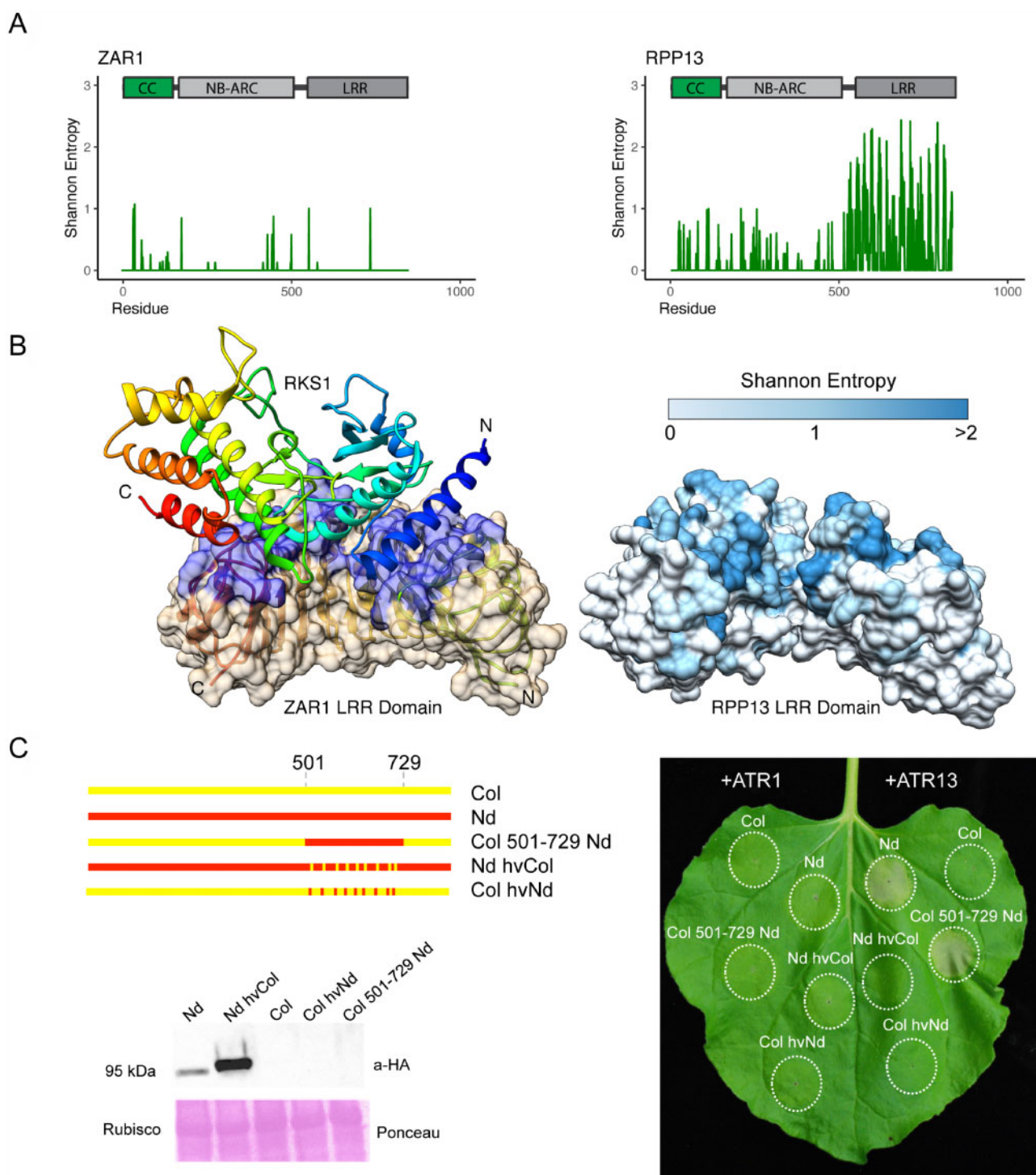
Figure 5 Highly variable residues in RPP13 overlap with the observed ZAR1-RKS1 binding site and are required for ATR13 recognition. A , Shannon entropy plots and domain diagrams for ZAR1, an indirect recognition CNL, and RPP13, a related hvNLR. B , Cryo-EM structure of RKS1 bound to ZAR1 (CC and NB-ARC domains omitted for clarity; PDB ID: 6J5W). RKS1 shown as a secondary structure diagram with rainbow coloring from blue (N-terminus) to red (C-terminus), ZAR1 LRR as a secondary structure diagram and transparent surface with RKS1 contact residues colored blue. RPP13 LRR domain homology model with surface oriented as in ZAR1 and colored by Shannon Entropy of the RPP13 clade alignment from low (light blue) to high entropy (dark blue). C , Chimeric constructs of RPP13 regions 501–729 containing highly variable LRR repeats. The constructs were designed by targeting amino acids with Shannon entropy > 1.5 bits and functionally tested by Agrobacterium -mediated transient expression assays in N. benthamiana together with cognate ATR13d41-Emco5 effector or ATR1d51-Emoy2-negative control at the final OD 600 of 0.6 with constructs mixed in equal ratio. The image was taken at 3 days post infiltration. Each construct was tested on 14 leaves and showed consistent presence/absence of HR on all leaves. Immunoblotting showed stable expression of both functional and mutated RPP13-Nd variants. No RPP13-Col variants could be detected despite having an intact HA tag similar to what has been reported previously (Rentel et al., 2008).
