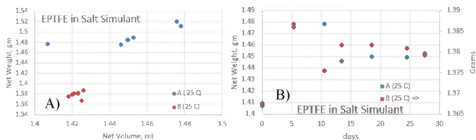
Figure 24. Density (A) and rate of mass gain (B) of ePTFE in Average Salt Simulant
