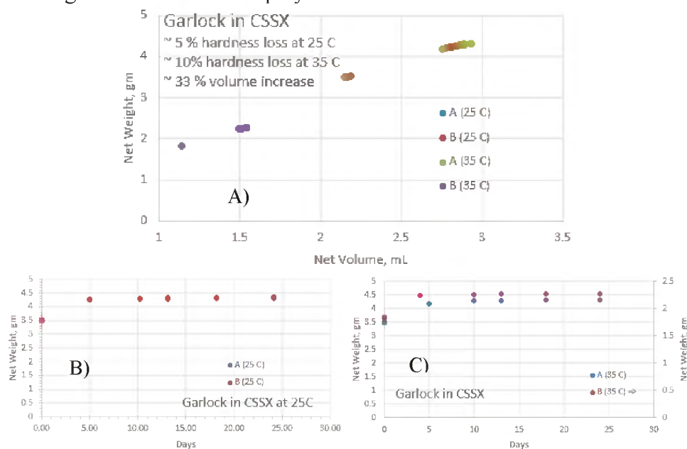
Figure 19. Density and mass gained by Garlock® Blue-Gard® 3700 in CSSX
