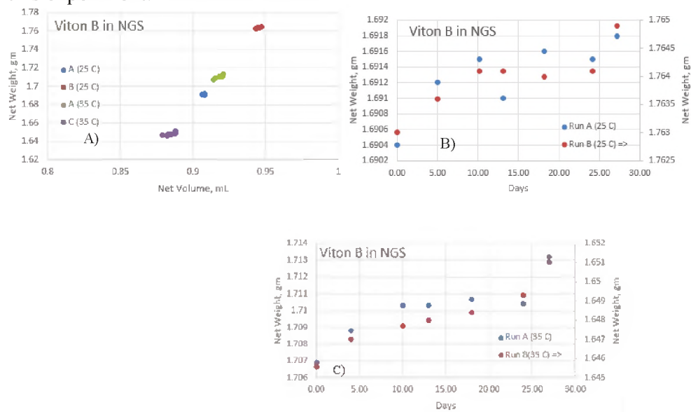
Figure 6. Density (A) and rate of mass gained at 25 °C (B), and at 35 °C (C) of Viton™ B in NGS solvent
