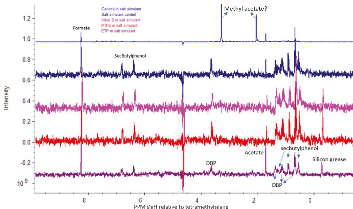
Figure 21. H-NMR (solvent suppression) of the Average salt simulant that contacted the gasket materials
