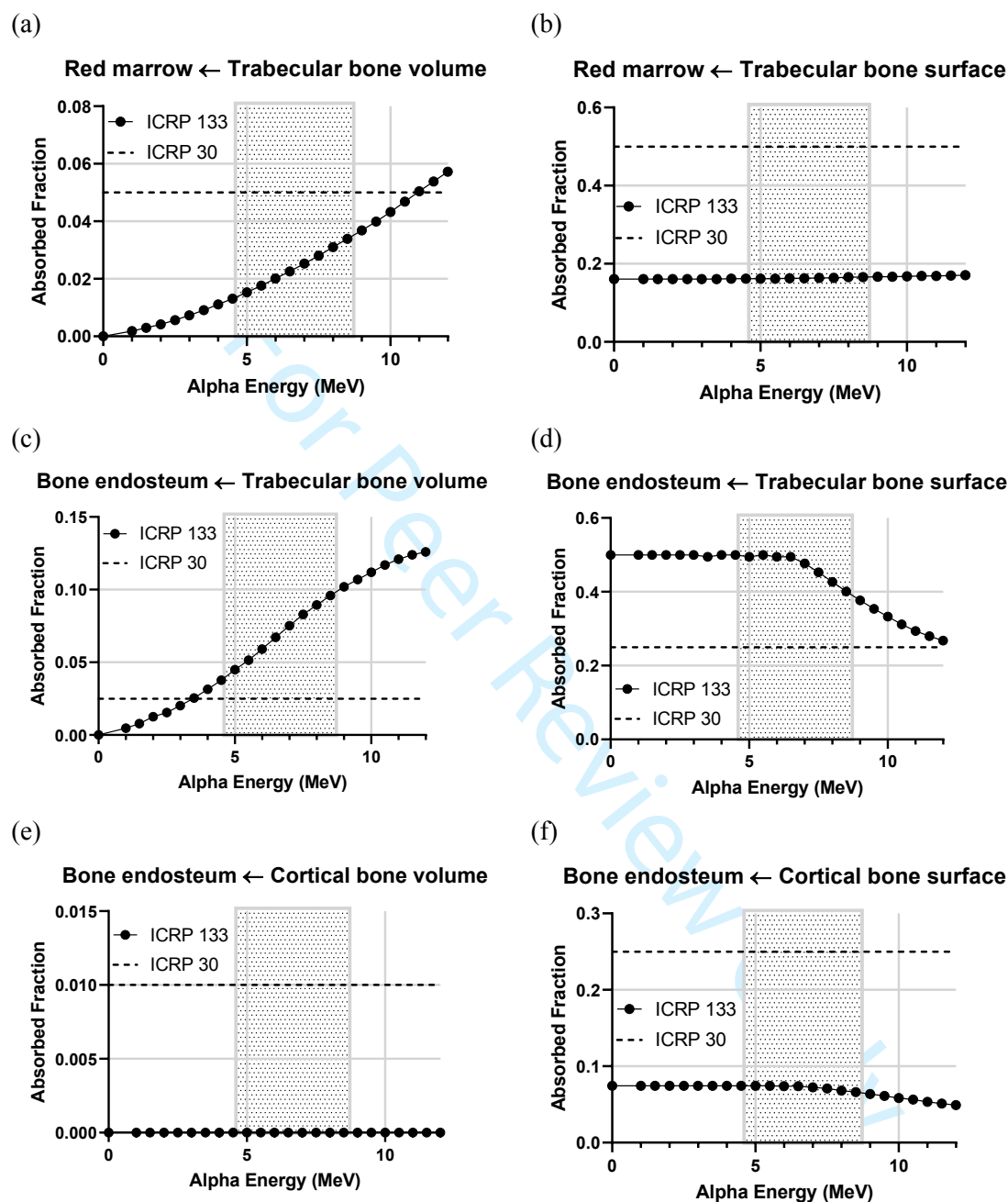
Figure 6. Plots of the fraction of the energy absorbed in a target tissue per alpha energy emitted from a skeletal source region. Data points (circles) are from ICRP Publication 133 (2016) and dashed lines are the values in ICRP Publication 30 (1979). The shaded region represents the range of alpha particle energies emitted in the ^{226}\text{Ra} and ^{228}\text{Ra} decay chains.
