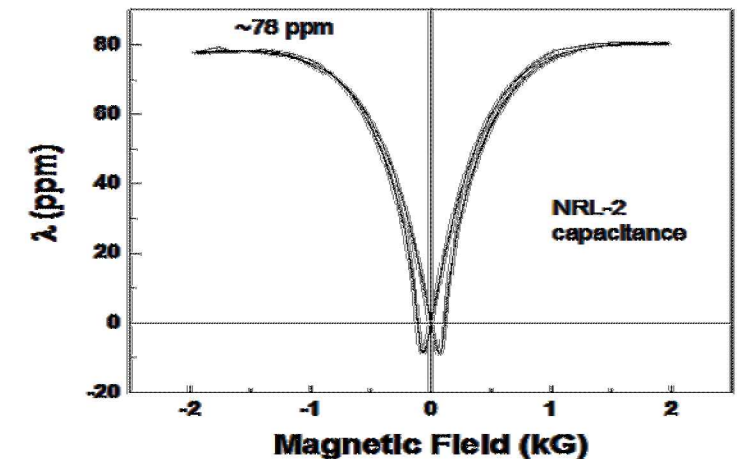
Magnetostriction measurement on original material performed at the NRL.
