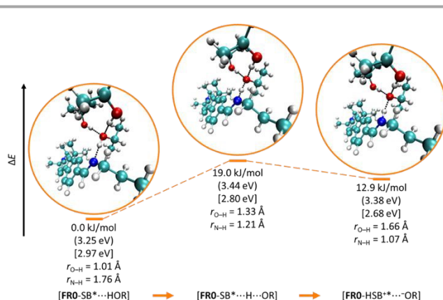
Fig. 11 Snapshots of the proton abstraction process from i -propanol. The SMD/CAM-B3LYP/6-31+G* optimized geometries of the [FRO-SB*...HOR] reactant, [FRO-SB*...H...OR] transition state, and [FRO-HSB*...OR] product of the ESPT process between FRO-SB in its S_1 electronic state and three i -propanol molecules (see the ESIT † for the computational details). The \Delta E values in kJ/mol are given relative to the reactant energy. The energies inside parentheses, in eV, are given relative to the [FRO-SB...HOR] minimum in the ground electronic state S_0 , while those inside square brackets correspond to the S_0 \rightarrow S_1 vertical transitions at each respective geometry. The r_{O-H} and r_{N-H} distances at each geometry represent the internuclear separations between the proton being transferred and the oxygen of i -propanol and the imine nitrogen of FRO-SB , respectively.
