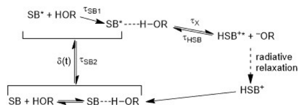
Fig. 5 Kinetic model for the ESPT reaction between FRO-SB and the alcohol solvent ROH.
