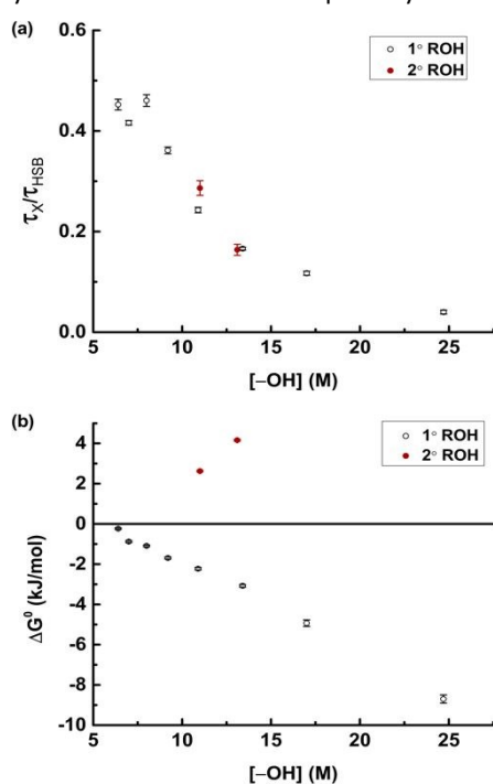
Fig. 6 Trends in dynamics and free energy as a function of relative [-OH]. (a) The ratio of the time constants \tau_x and \tau_{\text{HSB}} is plotted as a function of relative [-OH]. (b) \Delta G^0 for proton abstraction obtained from the ratio of FRO-SB* to FRO-HSB* emission as a function of relative [-OH]. We note good agreement between the time-resolved and the steady-state data for the linear alcohols.
