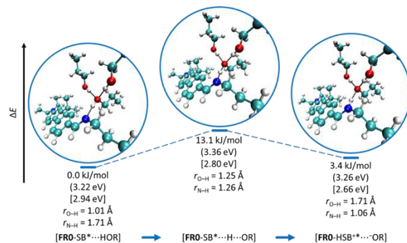
Fig. 10 Snapshots of the proton abstraction process from n -propanol. The SMD/CAM-B3LYP/6-31+G* optimized geometries of the [FRO-SB*...HOR] reactant, [FRO-SB*...H...OR] transition state, and [FRO-HSB*...OR] product of the ESPT process between FRO-SB in its S_1 electronic state and three n -propanol molecules (see the ESIT † for the computational details). The \Delta E values in kJ/mol are given relative to the reactant energy. The energies inside parentheses, in eV, are given relative to the [FRO-SB...HOR] minimum in the ground electronic state S_0 , while those inside square brackets correspond to the S_0 \rightarrow S_1 vertical transitions at each respective geometry. The r_{O-H} and r_{N-H} distances at each geometry represent the internuclear separations between the proton being transferred and the oxygen of n -propanol and the imine nitrogen of FRO-SB , respectively.
