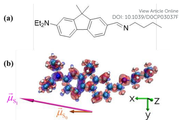
Fig. 1 The FRO-SB molecule and how its electronic density changes upon excitation. (a) FRO-SB super photobase. (b) The structure of the isolated FRO-SB molecule in its ground electronic S_0 state, the dipole moments characterizing the S_0 (shorter orange vector) and electronically excited S_1 (longer magenta vector) states, and the S_1 - S_0 total electronic density difference, resulting from the CC/EOMCC calculations described in the main text. The red/blue color indicates an increase/decrease in the electron density upon the S_0 \rightarrow S_1 excitation.
