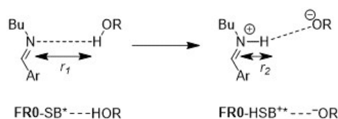
Fig. 8 Schematic representation of the r_1 and r_2 N-H internuclear distances needed to create the grid defining the ESPT reaction pathway.
