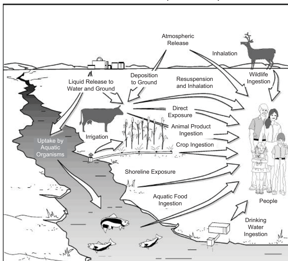
FIGURE 3-2 Potential Radiation Exposure Pathways to Man
