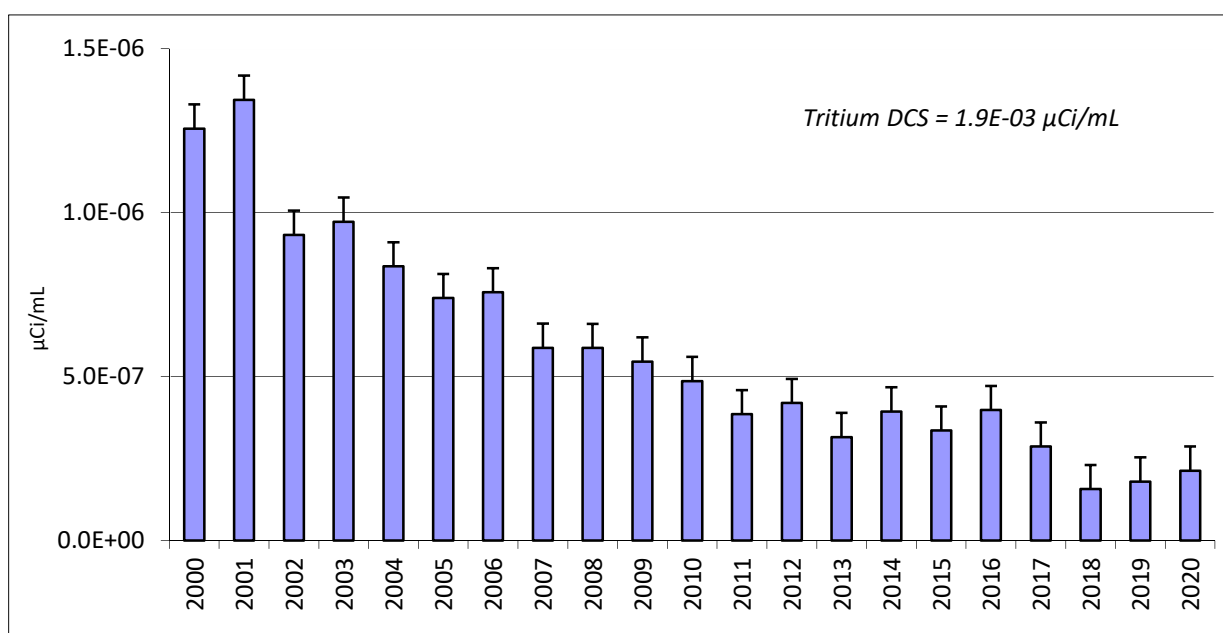
FIGURE 2-6 Average Concentration of Tritium in Surface Water at WNNADR: 2000-2020
