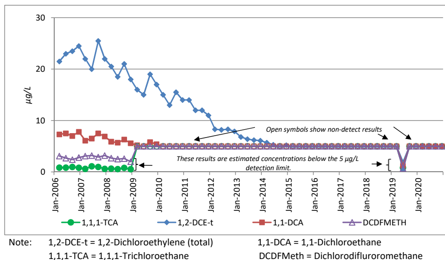
FIGURE 4-11 Concentrations of 1,2-DCE-t, 1,1,1-TCA, 1,1-DCA, and DCDFMeth at Well 8612 in the S&G Unit
