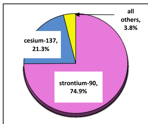
FIGURE 3-5 Dose Percent by Radionuclide from Waterborne Releases in 2020
