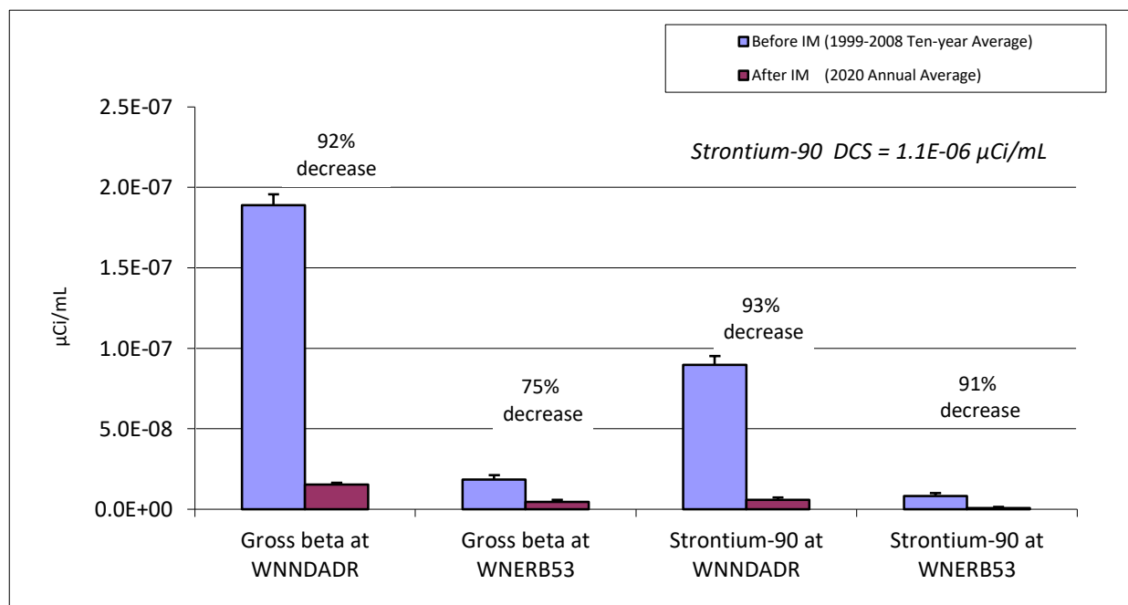
FIGURE 2-5 Average Gross Beta and Strontium-90 Concentrations in Surface Water on the South Plateau at WNNADR a and WNERB53 b Before and After the NDA Interim Measure (IM) was Installed
