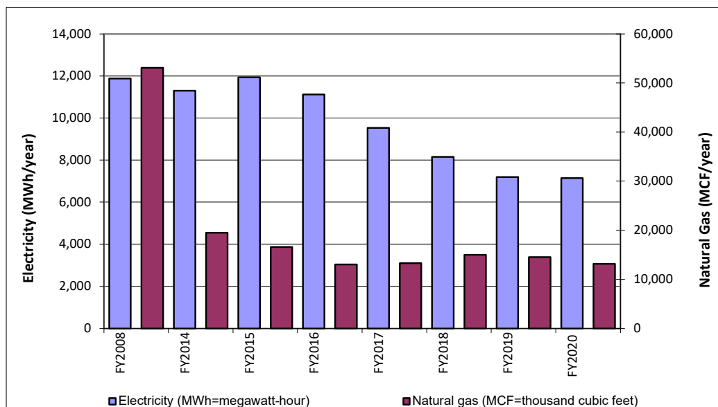
FIGURE 1-2 Energy Use
