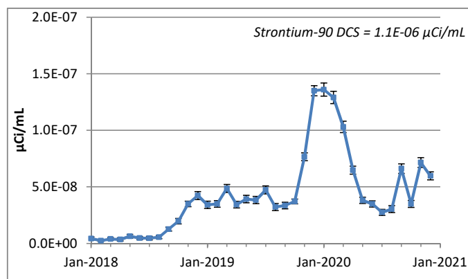
Recent strontium-90 concentrations at WNSW74A
