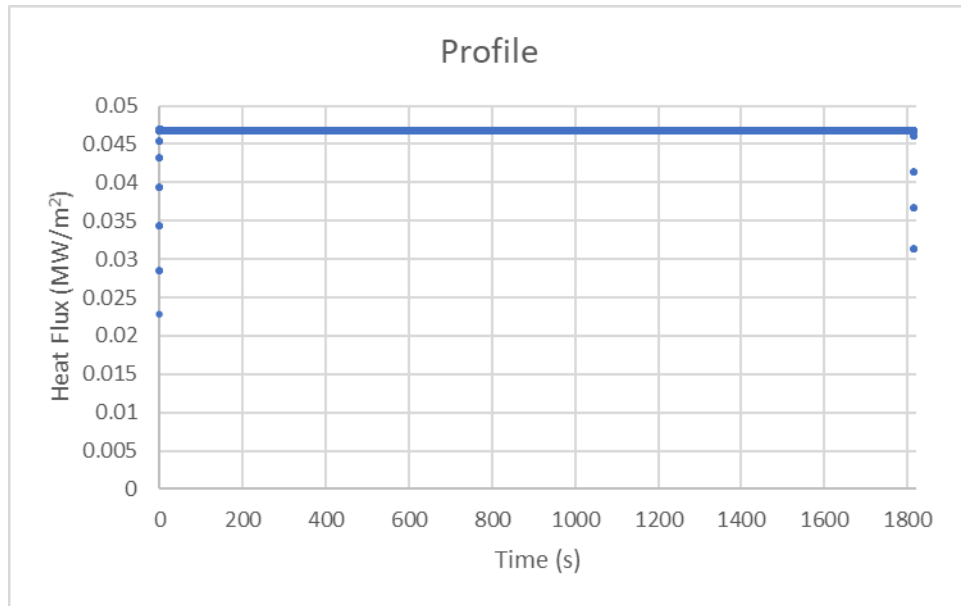
Figure 3-83: Test 1-20 Heat Flux Profile
