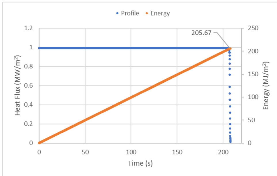
Figure 3-34: Test 1-09 Total Energy
