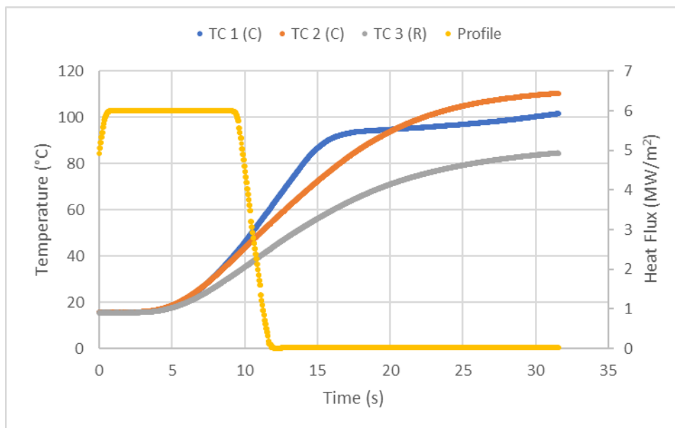
Figure 3-131: Test 1-28 Thermal Monitoring
