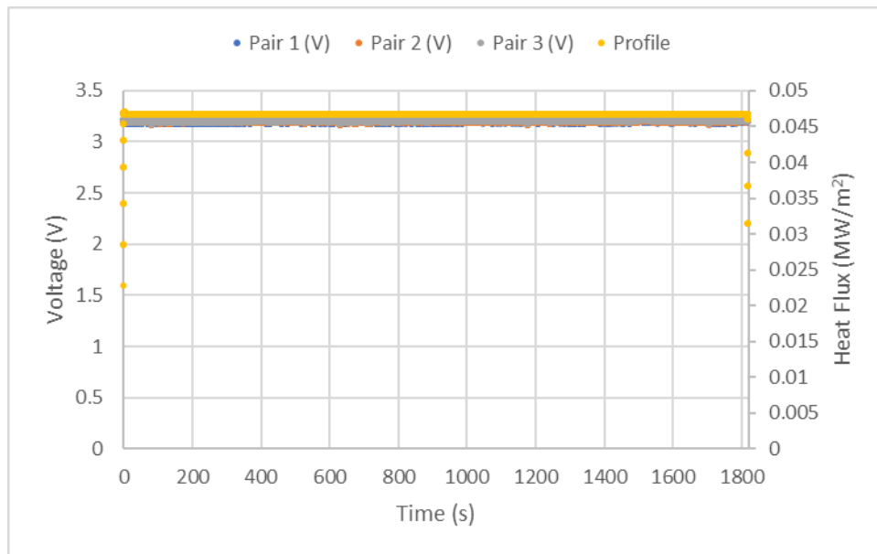
Figure 3-85: Test 1-20 Electrical Monitoring
