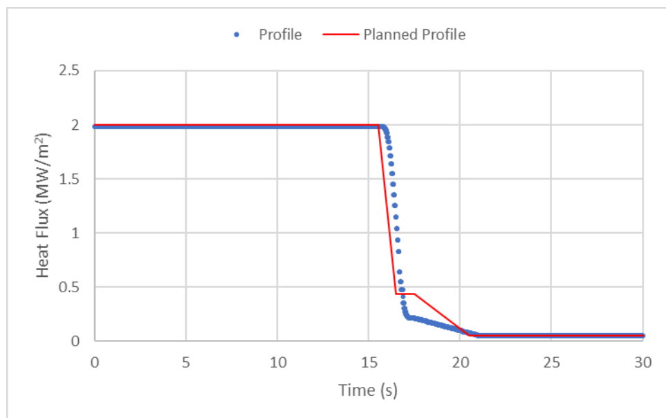
Figure 3-177: Test 1-36 Heat Flux Profile
