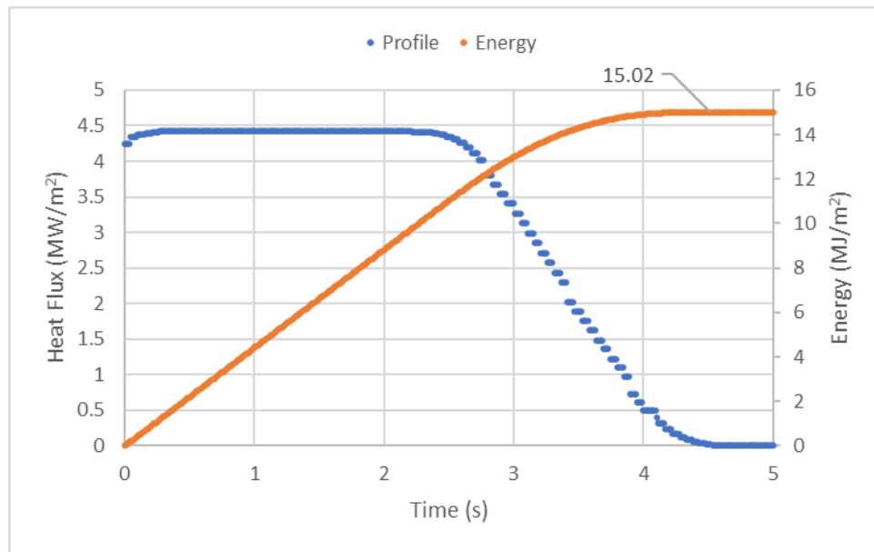
Figure 3-112: Test 1-25 Total Energy
