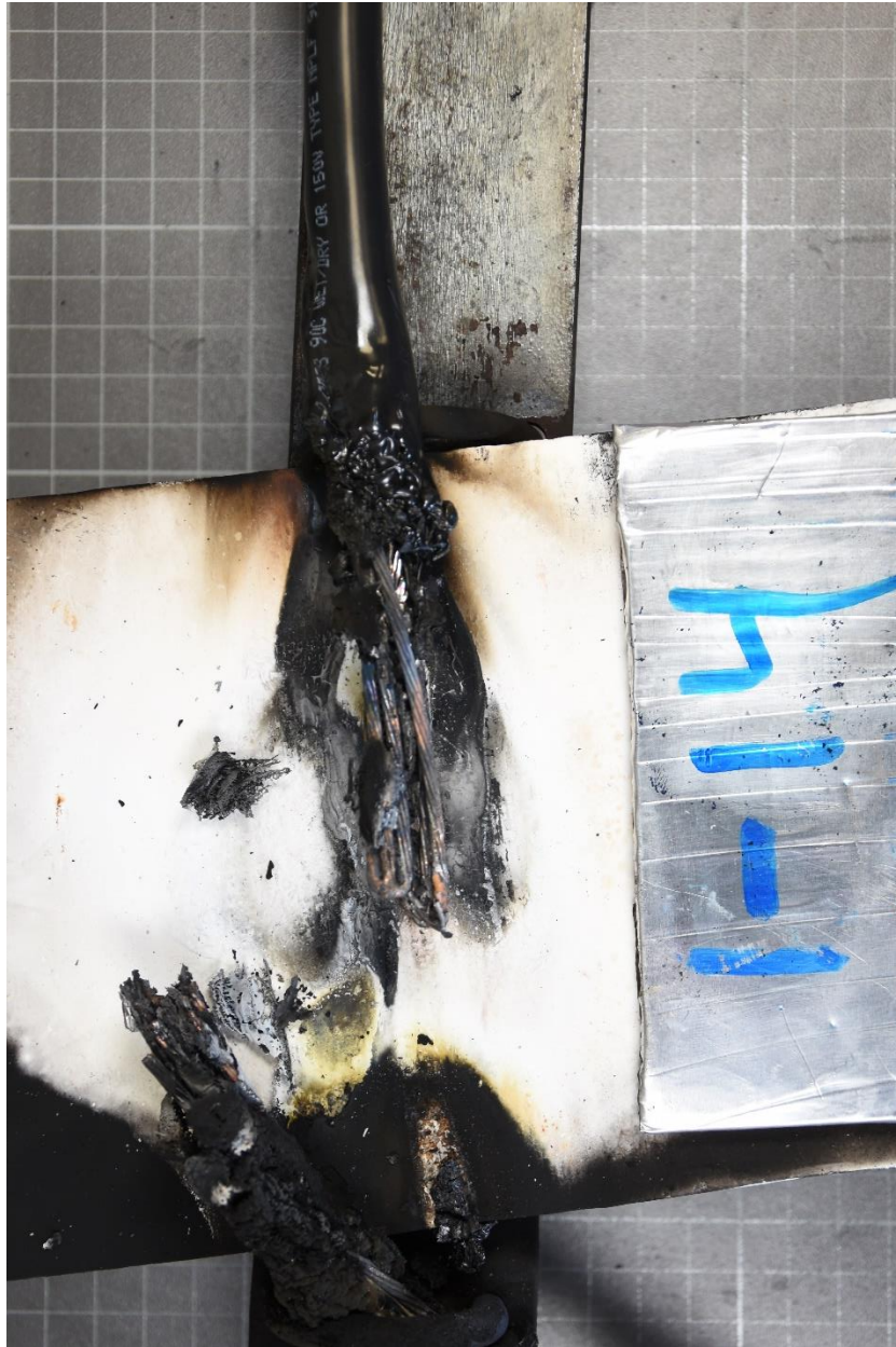
Figure 3-58: Test 1-14 Post-test Photo
