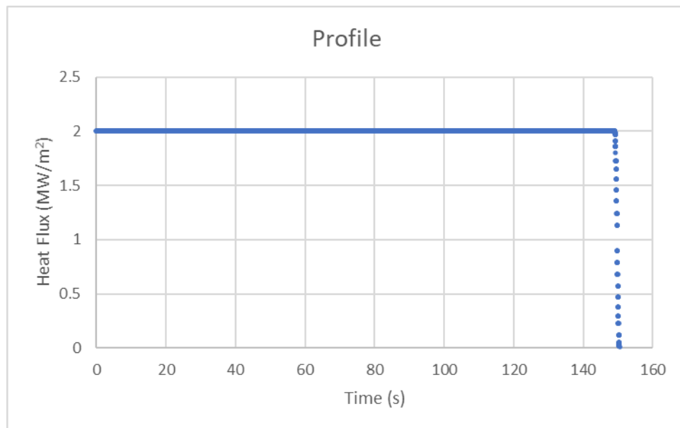
Figure 3-63: Test 1-16 Heat Flux Profile
