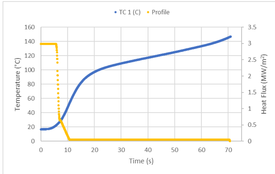
Figure 3-155: Test 1-32 Thermal Monitoring
