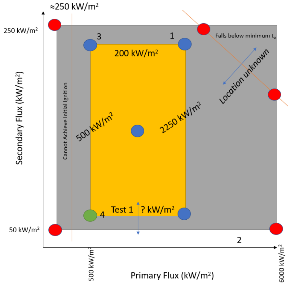
Figure 2-3: Test Plan to resolve Semi-empirical Model
