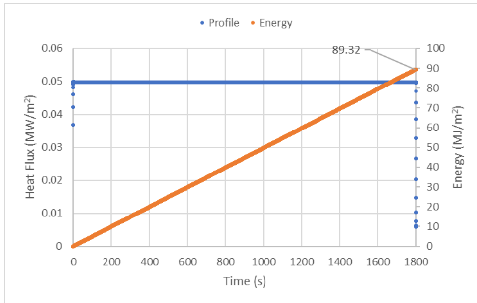
Figure 3-73: Test 1-18 Total Energy
