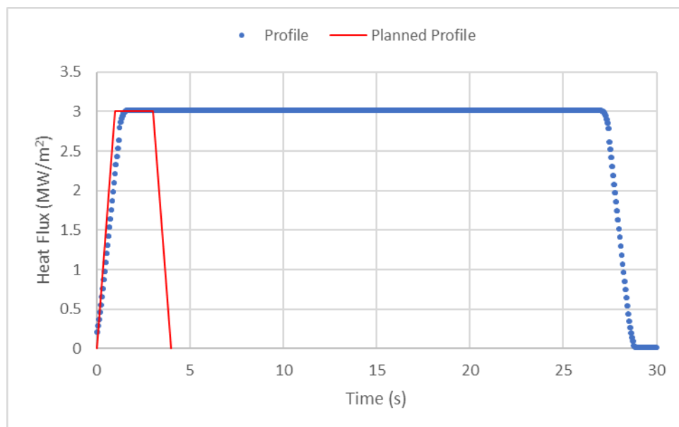
Figure 3-88: Test 1-21 Heat Flux Profile
