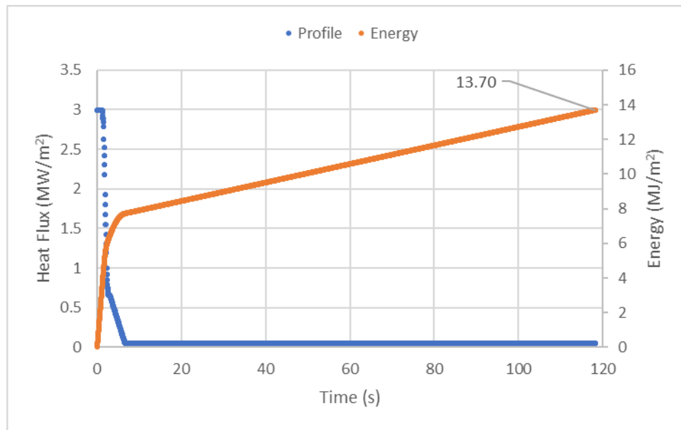
Figure 3-2: Test 1-02 Total Energy
