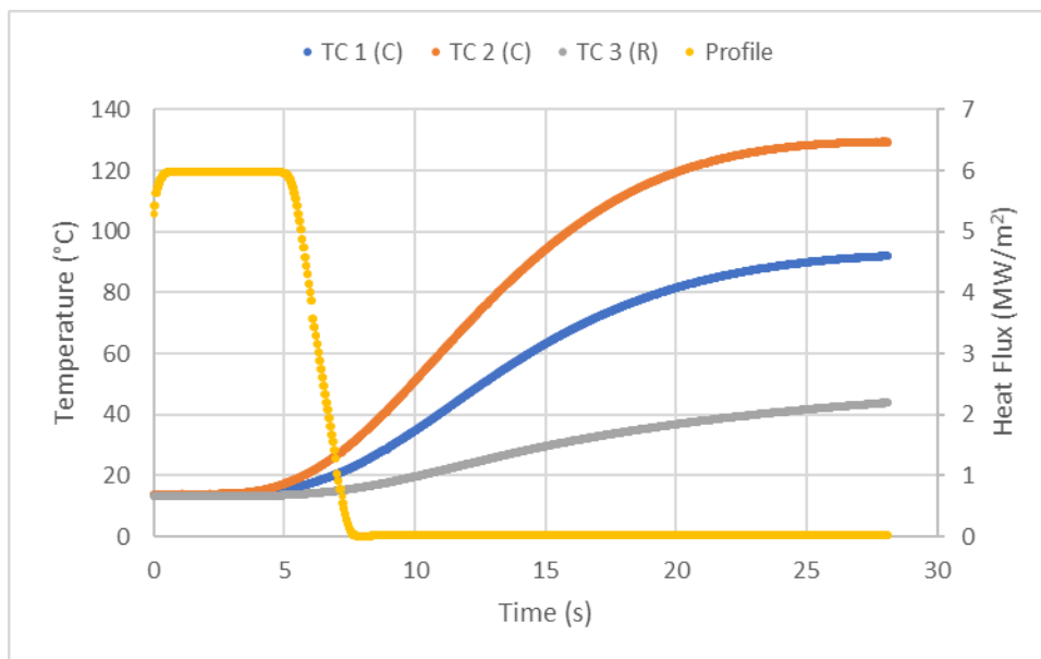
Figure 3-125: Test 1-27 Thermal Monitoring
