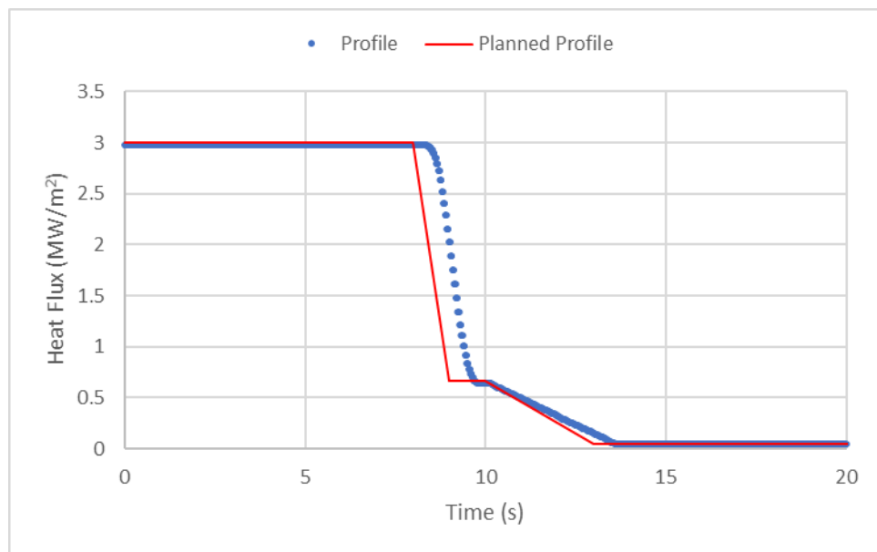
Figure 3-135: Test 1-29 Heat Flux Profile
