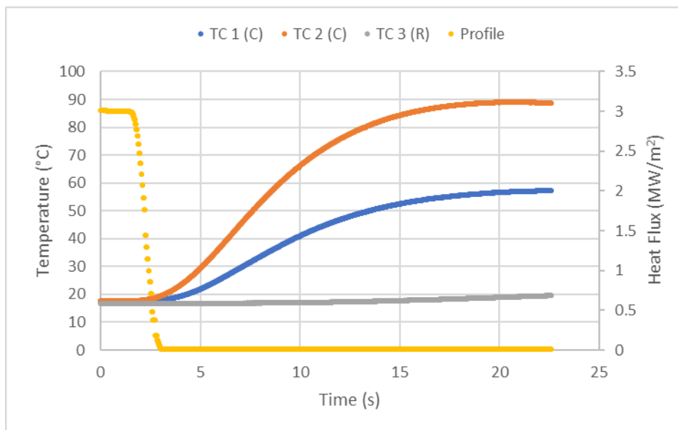
Figure 3-101: Test 1-23 Thermal Monitoring
