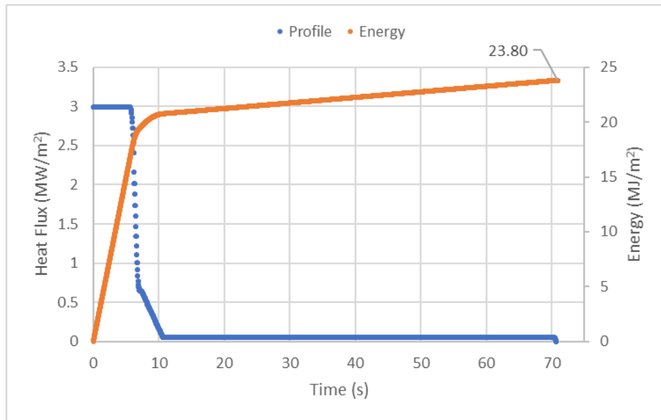
Figure 3-154: Test 1-32 Total Energy
