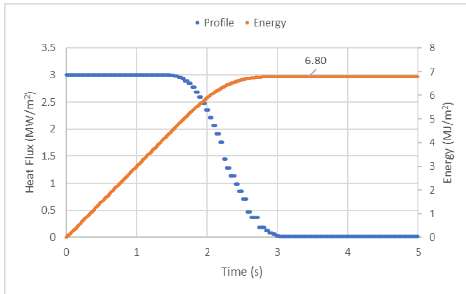
Figure 3-100: Test 1-23 Total Energy
