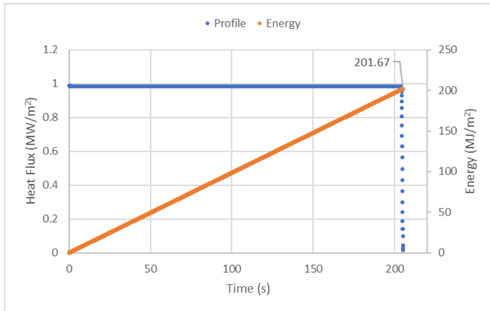
Figure 3-39: Test 1-10 Total Energy
