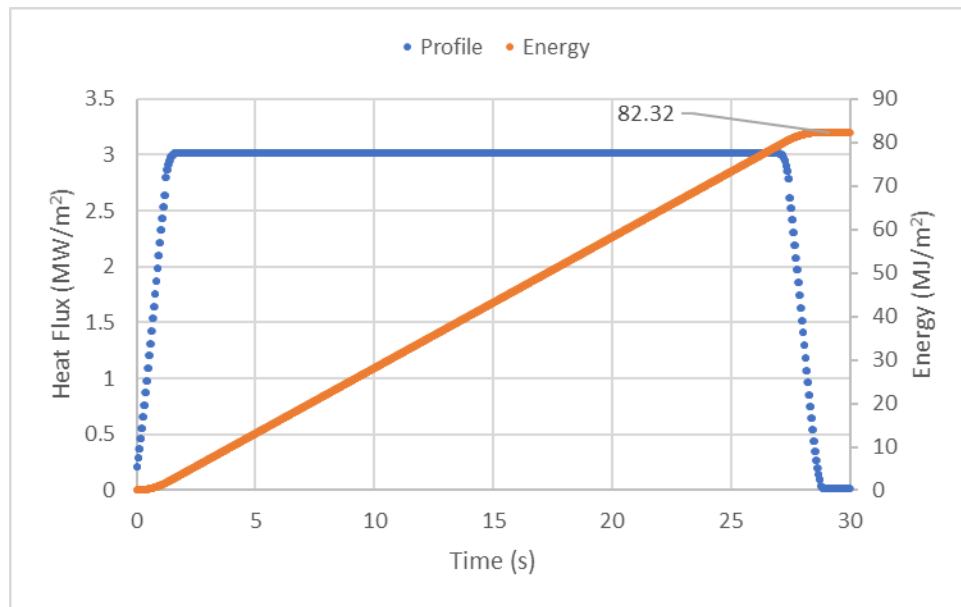
Figure 3-89: Test 1-21 Total Energy
