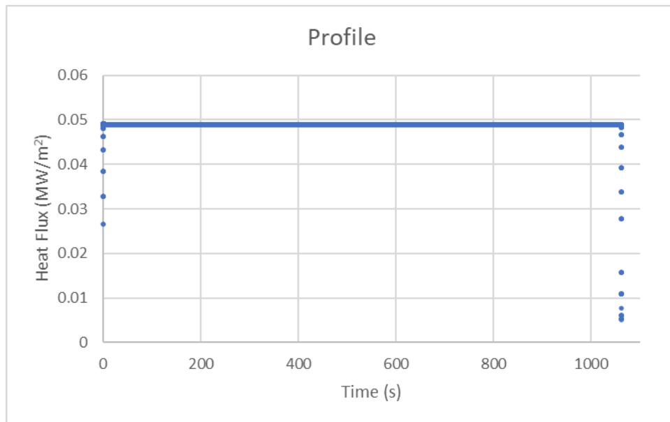
Figure 3-78: Test 1-19 Heat Flux Profile
