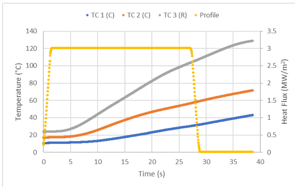
Figure 3-90: Test 1-21 Thermal Monitoring
