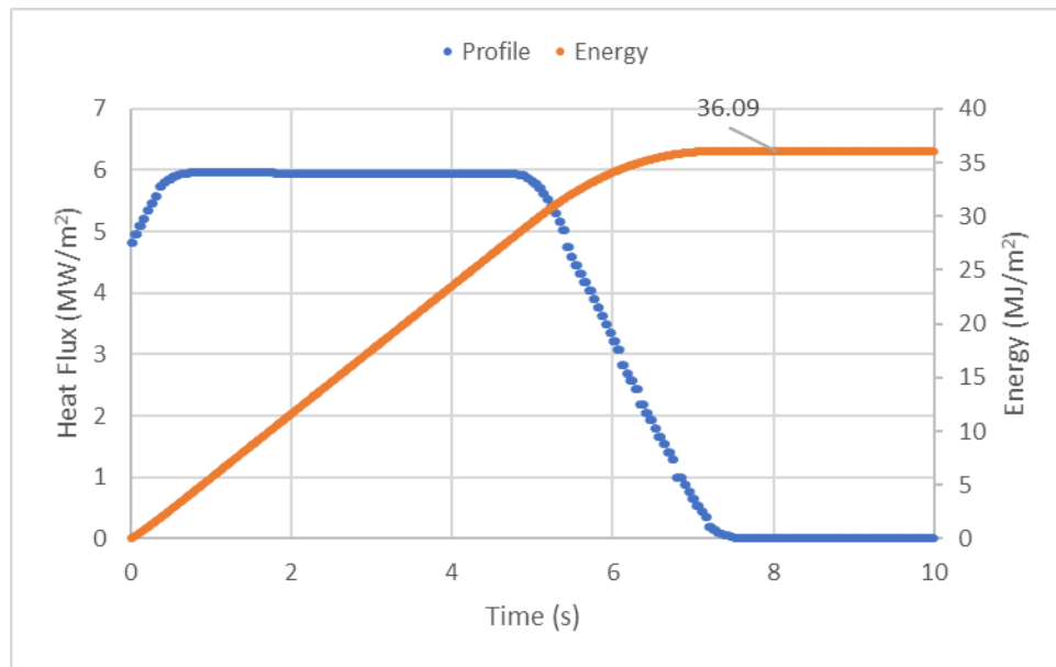
Figure 3-118: Test 1-26 Total Energy
