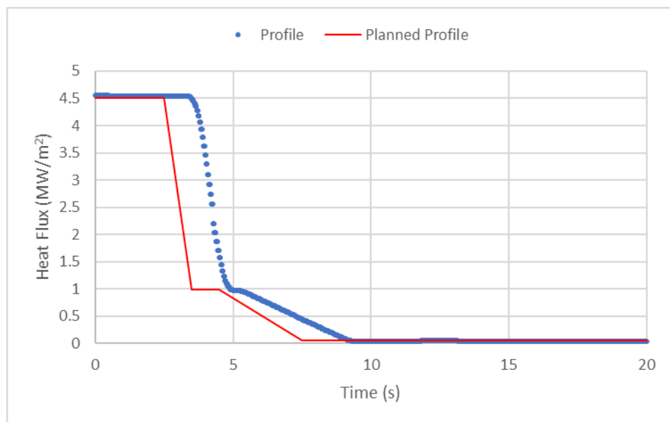
Figure 3-165: Test 1-34 Heat Flux Profile
