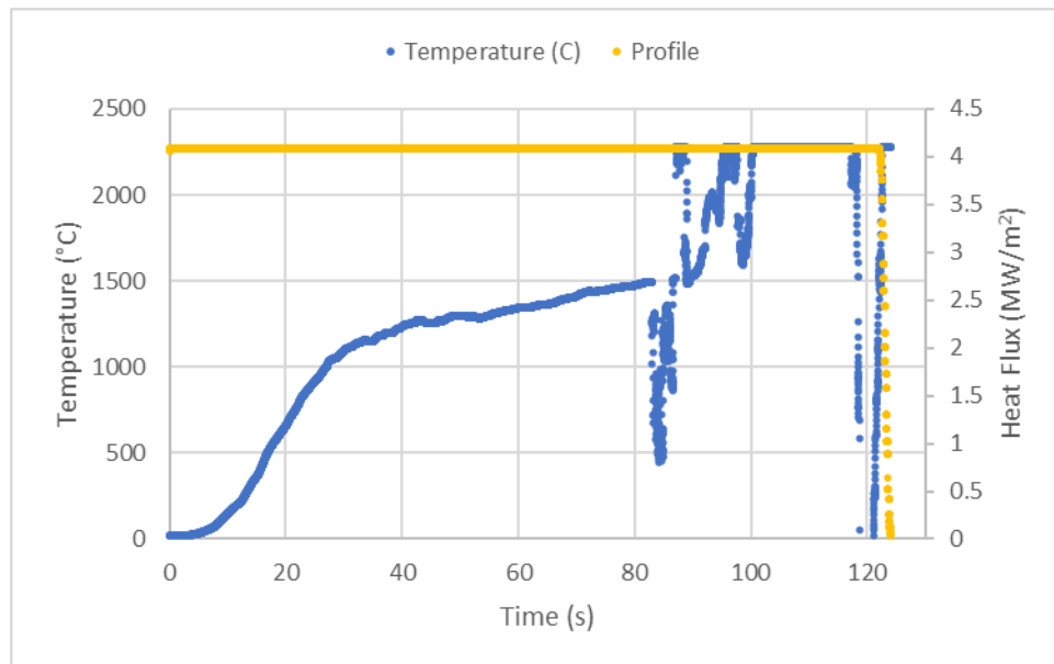
Figure 3-61: Test 1-15 Thermal Monitoring
