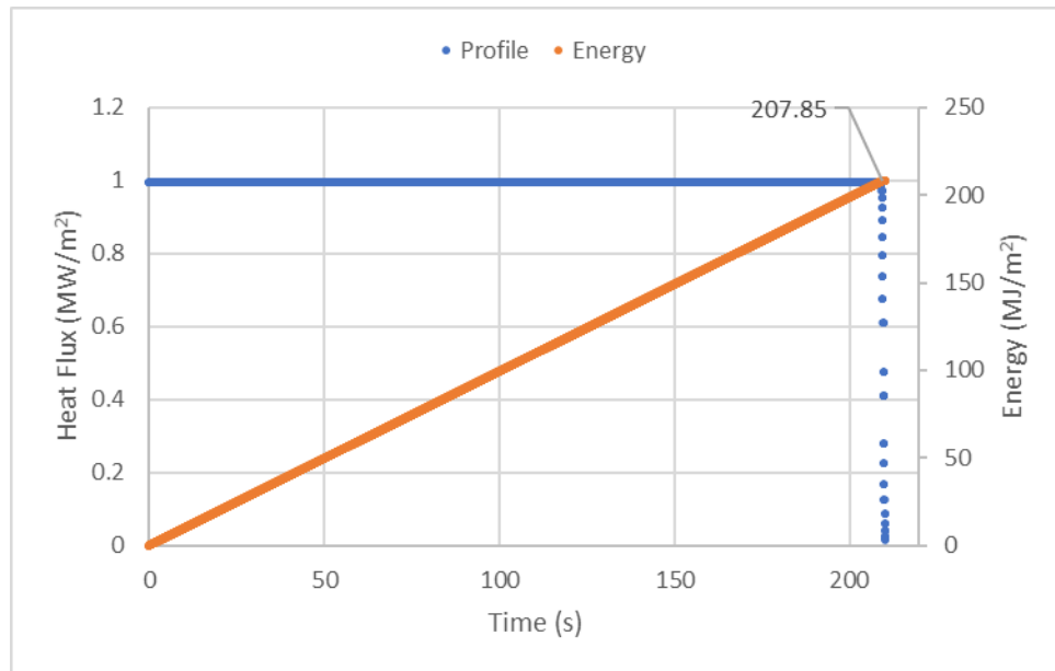
Figure 3-44: Test 1-11 Total Energy
