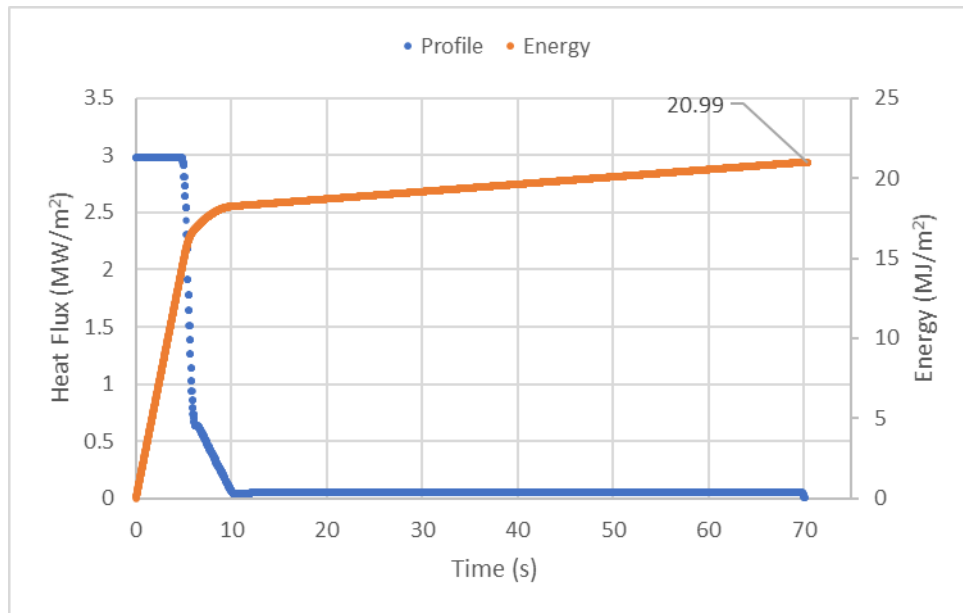
Figure 3-192: Test 1-38 Total Energy
