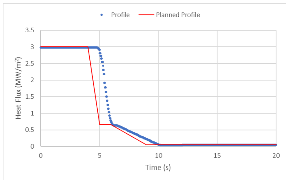
Figure 3-191: Test 1-38 Heat Flux Profile
