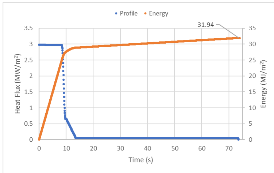
Figure 3-136: Test 1-29 Total Energy
