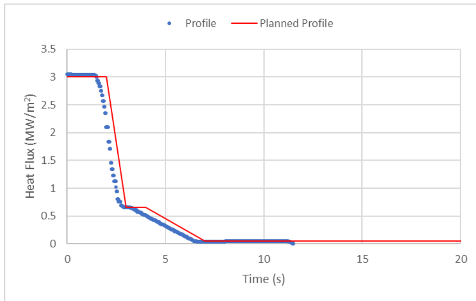
Figure 3-12: Test 1-05 Heat Flux Profile
