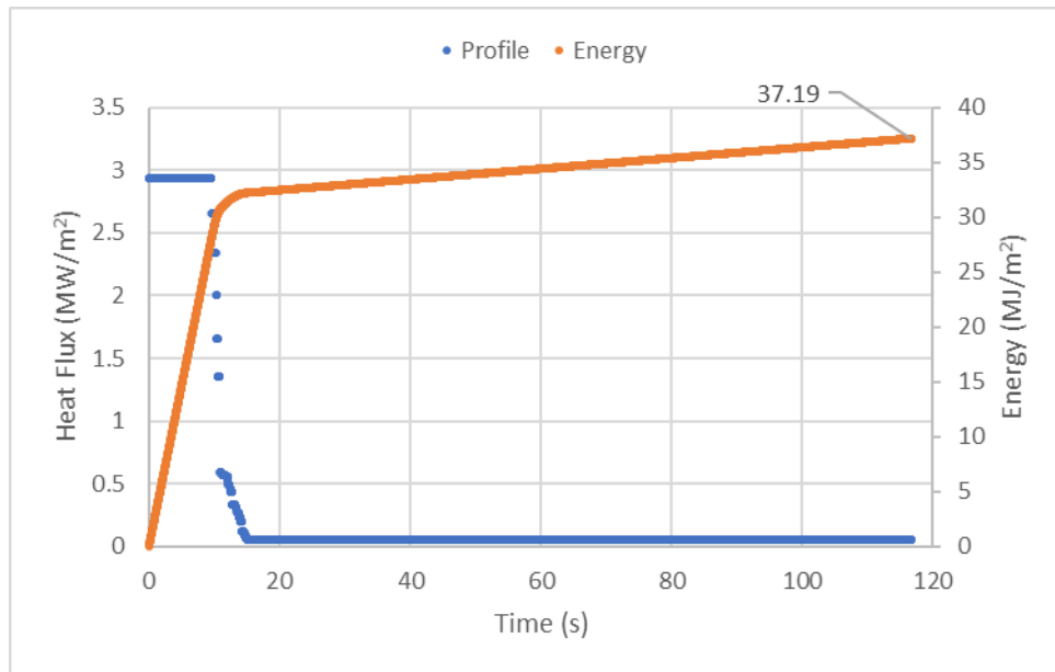
Figure 3-7: Test 1-03 Total Energy
