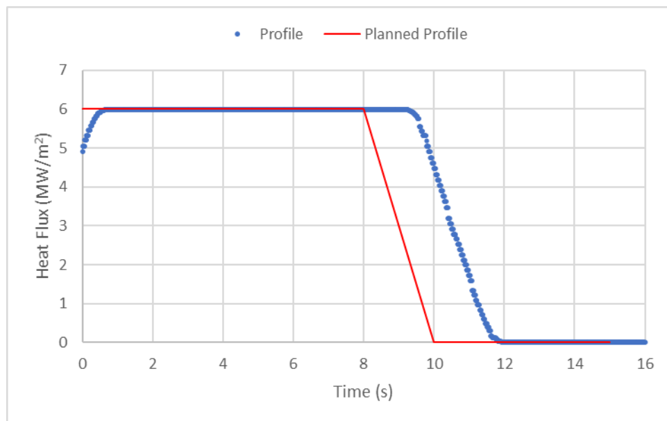
Figure 3-129: Test 1-28 Heat Flux Profile
