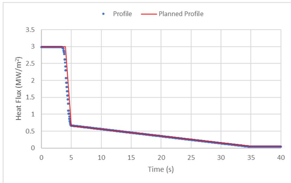
Figure 3-22: Test 1-07 Heat Flux Profile
