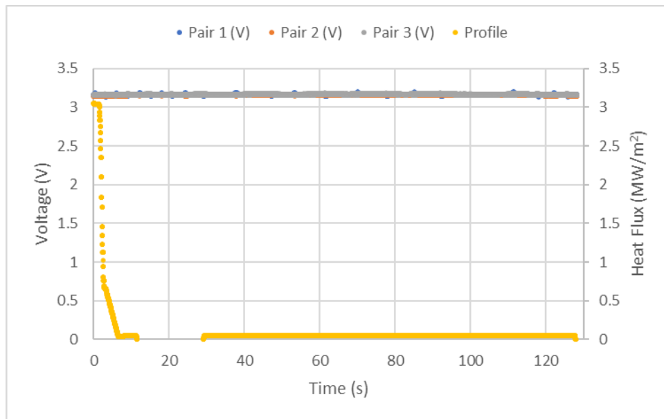
Figure 3-14: Test 1-05 Electrical Monitoring
