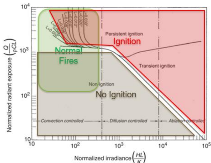
Figure 1-1: Ignition Threshold for Blackened Cellulose (Martin 1965)
