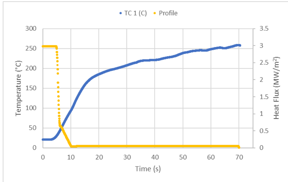
Figure 3-193: Test 1-38 Thermal Monitoring
