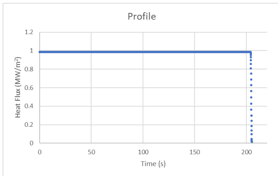
Figure 3-38: Test 1-10 Heat Flux Profile
