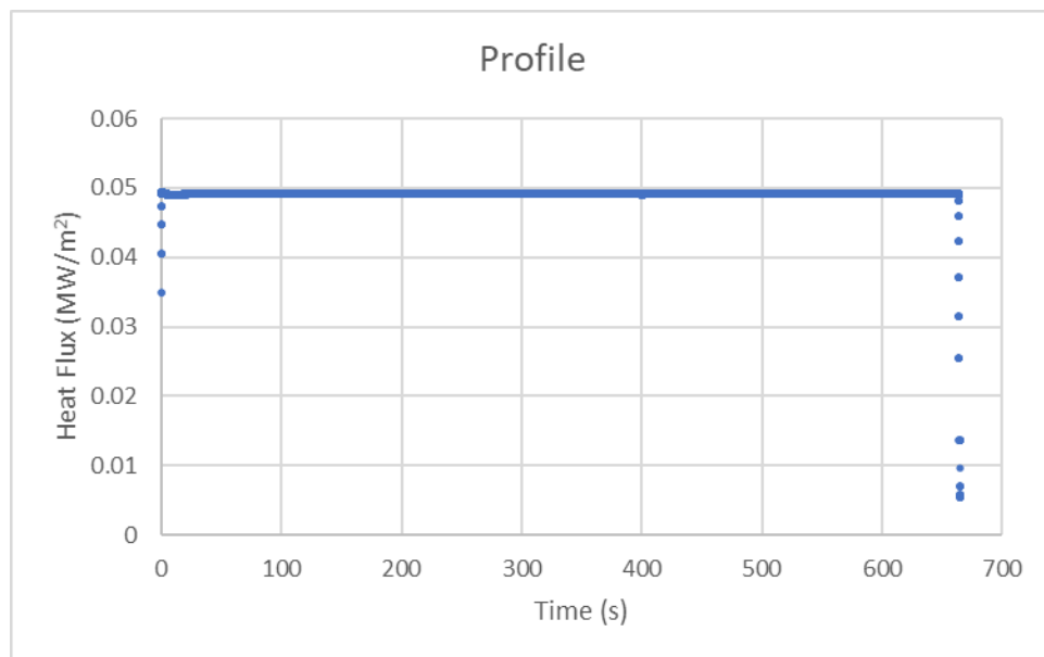
Figure 3-67: Test 1-17 Heat Flux Profile
