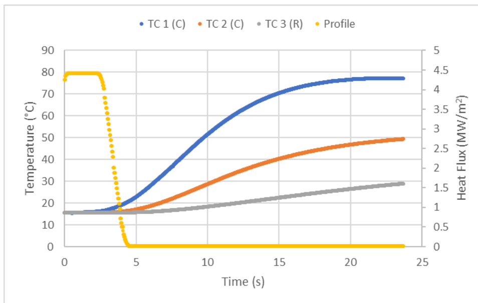
Figure 3-113: Test 1-25 Thermal Monitoring
