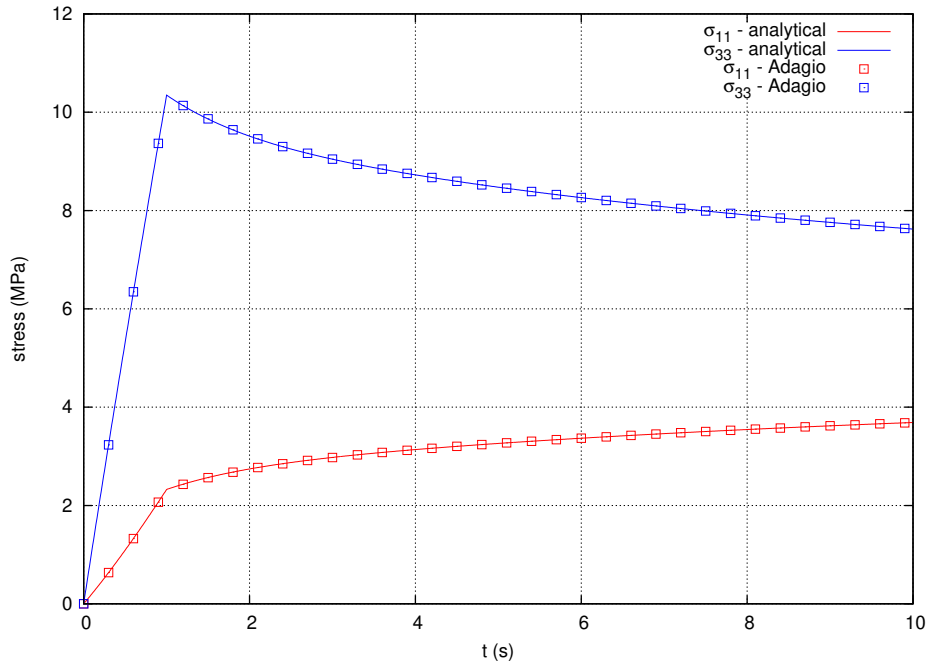
Figure 4-131. The axial and lateral stresses.
