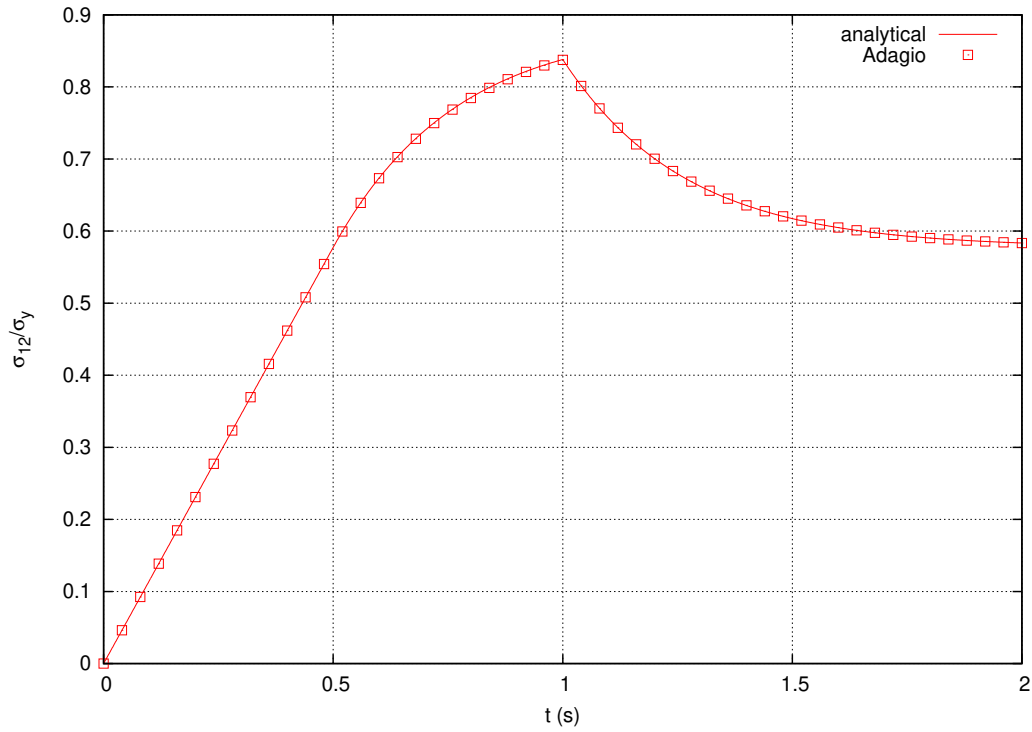
Figure 4-136. Simple shear
