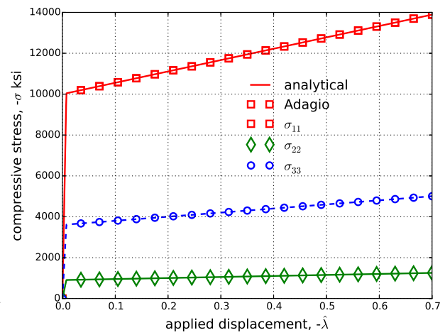
(b) Loading aligned with the W direction
