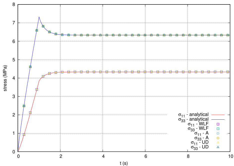
Figure 4-132. The axial and lateral stresses with the shift factor models. (A) denotes the Arrhenius model and (UD) denotes the user defined model.
