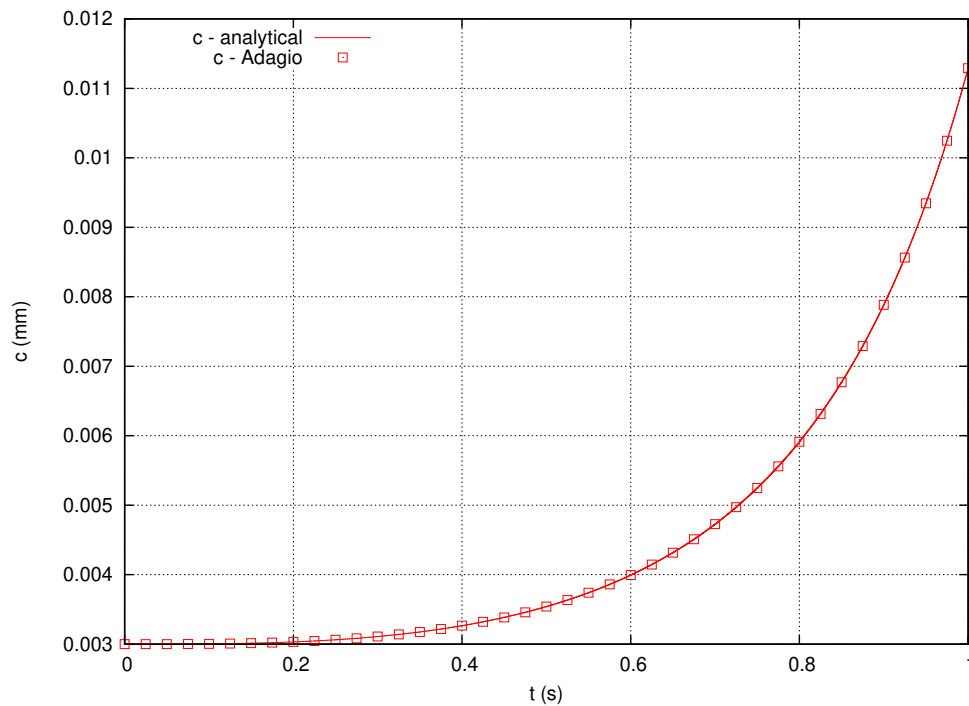
Figure 4-133. Crack size
