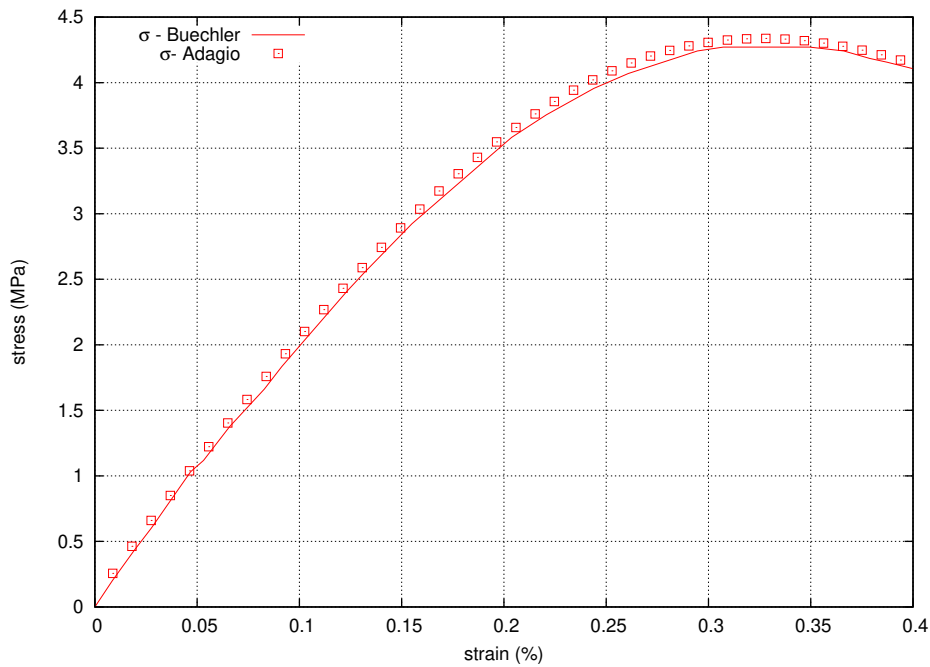
Figure 4-134. Uniaxial compression
