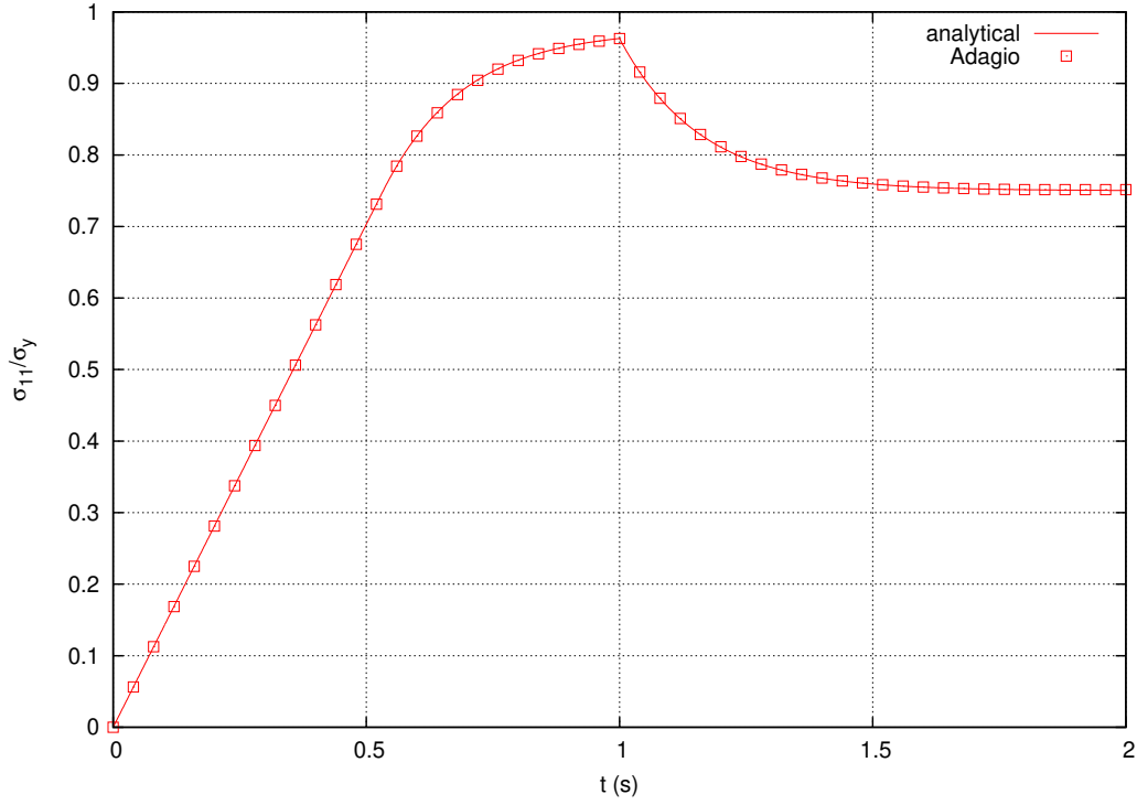
Figure 4-135. Uniaxial tension
