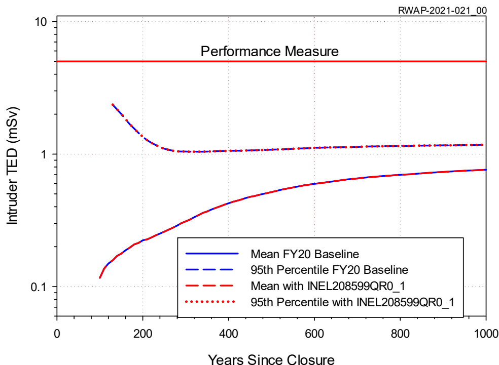
Figure 3. Acute Construction Intrusion Scenario TED Time History with and without the INEL208599QR0_1 Waste Stream
