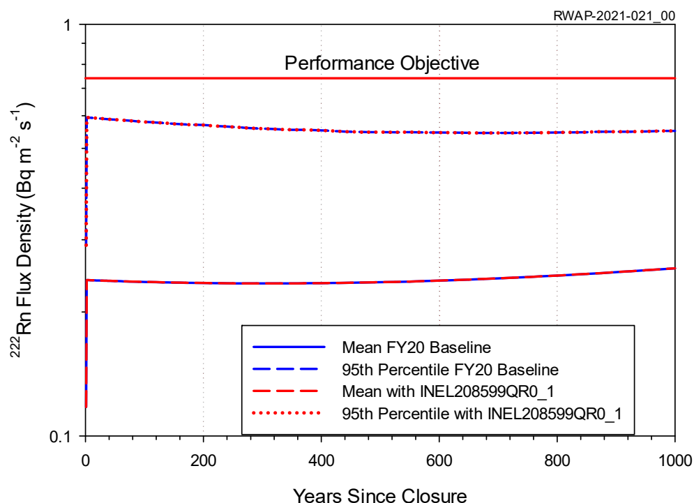
Figure 4. ^{222}\text{Rn} Flux Density Time History with and without the INEL208599QR0_1 Waste Stream
