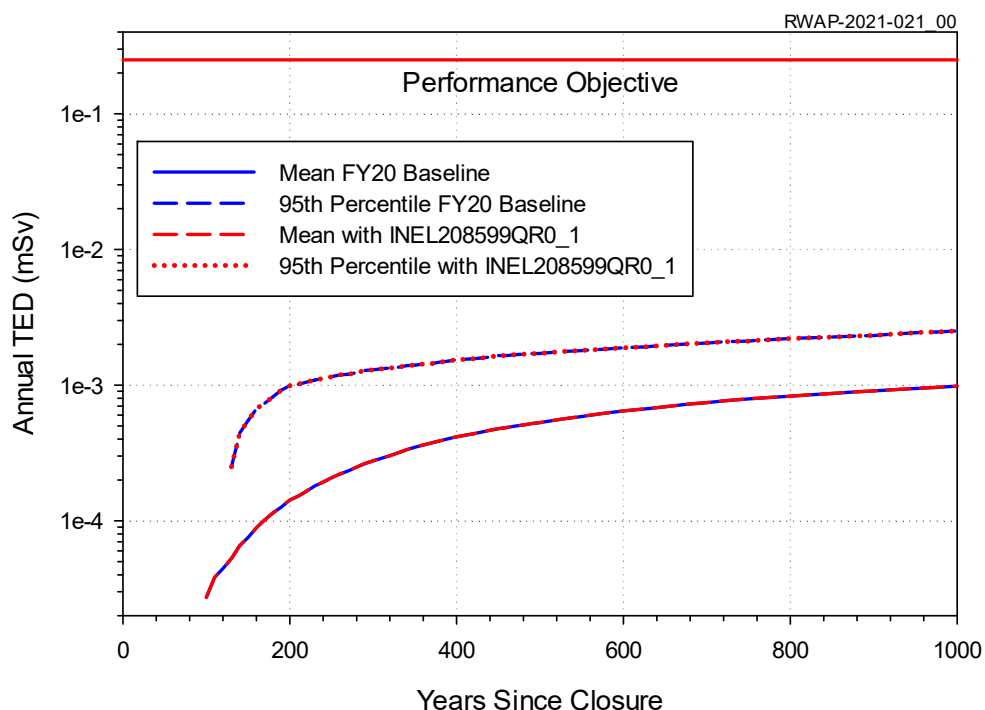
Figure 2. All-Pathways Annual TED Time History for a Resident at the 100-m Boundary with and without INEL208599QR0_1 Waste Stream
