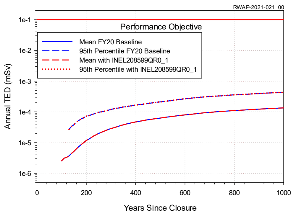
Figure 1. Air Pathway Annual TED Time History for a Resident at the 100-m Boundary with and without the INEL208599QR0_1 Waste Stream
