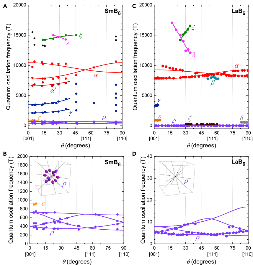
Figure 7. Comparison of Angular Dependence of Quantum Oscillation Frequencies in SmB 6 and LaB 6
