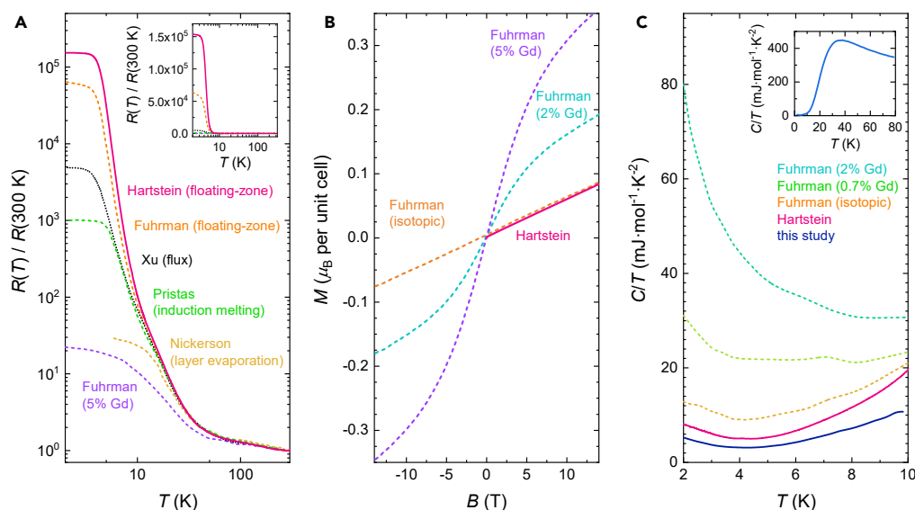
Figure 1. Comparison of Electrical Transport, Magnetic, and Thermal Properties of \text{SmB}_6 Single Crystals
