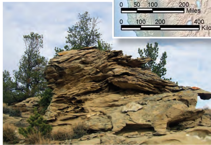
Saline rock formations near Belfry, Montana. (Courtesy of John Talbott, BSCSP)
