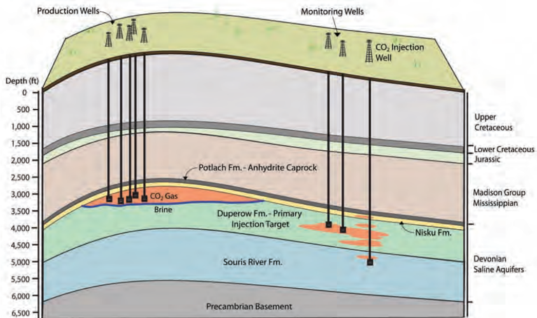
Schematic graphic of Kevin Dome in northcentral Montana.
