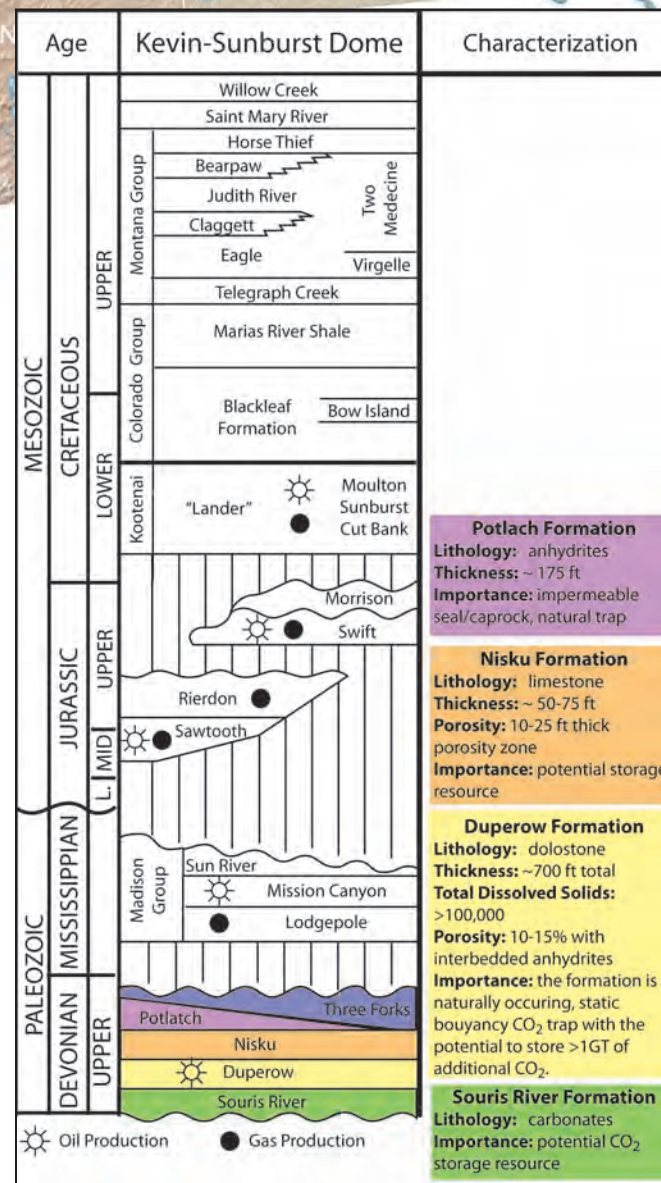
Stratigraphic column highlighting formations of interest at Kevin Dome.
