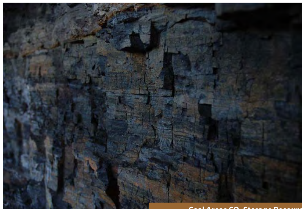
Many subsurface coal seams are potential storage opportunities.
