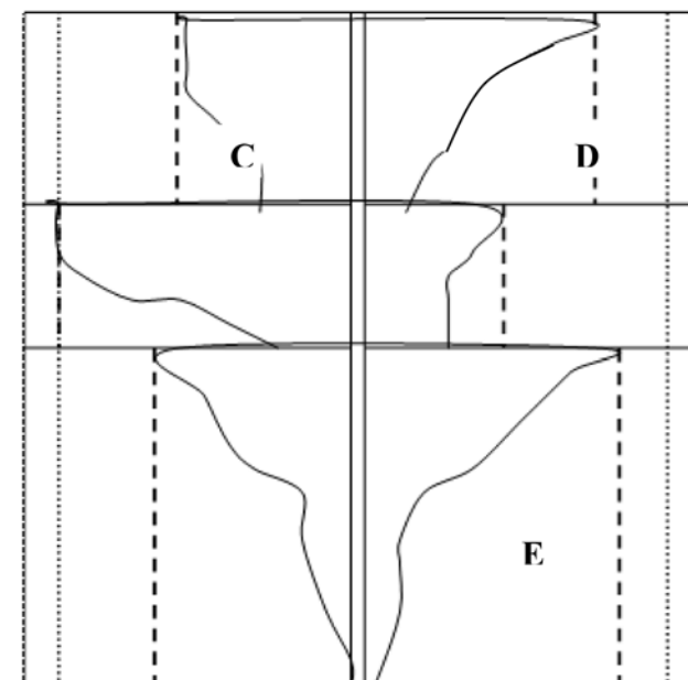
Figure 3: Side view of injection well and plume area. The outer vertical dotted lines are defined by the outer areal circle (Depicted by B in Figure 2). The “plume” area enclosed within each interval that is bound by vertical dashed lines represents the numerator of the E L term (area enclosed within C); the denominator is the entire space outlined by the dotted line (area enclosed within D). Within the area bound by the dashed lines, the lower portion is not contacted due to gravity (area depicted by E) and is removed by the E g term. The E d term then defines the CO 2 displacement efficiency in the plume region.
