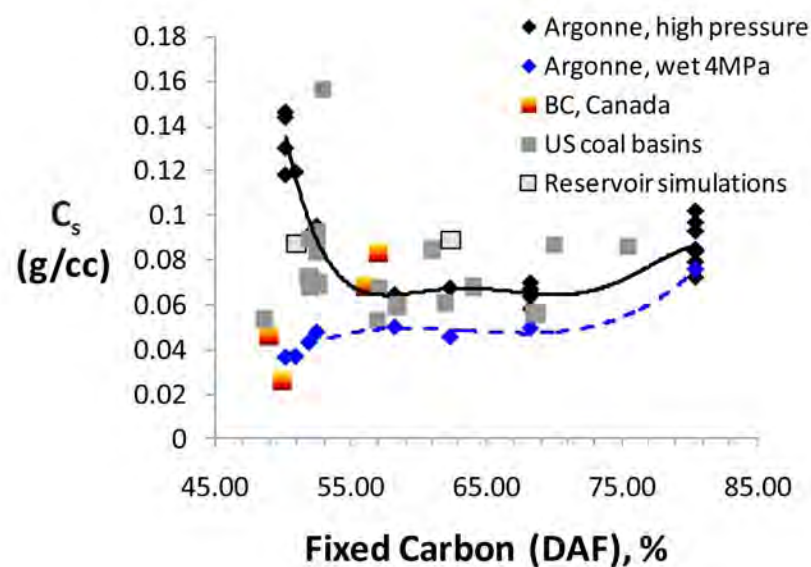
Figure 1. Average CO 2 Sorption (expressed in g/cc) vs. Coal Rank (expressed as percent fixed carbon on a dry and ash free basis (daf)). Red and gray solid squares represent experimental data for Canadian and North American coals, respectively. Black and blue solid diamonds represent experimental data for Argonne premium coals at saturation (high pressure) and at low pressure (4 MPa wet), respectively. Gray solid squares with black outline represent data for two reservoir simulations. (Botnen et al., 2009; Bromhal et al., 2005; Busch et al., 2003; Chikatamarla et al., 2004; Clarkson and Bustin, 1999; Day et al., 2008a; Durucan and Q., 2009; Fitzgerald et al., 2005; Fitzgerald et al., 2006; Goodman et al., 2007; Harpalani and Mitra, 2010; Harpalani et al., 2006; Jessen et al., 2008; Ozdemir and Schroeder, 2009; Reeves et al., 2005; Romanov and Soong, 2008; Ross et al., 2009; Siemons and Busch, 2007).
