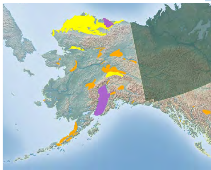
Alaska coal base map from Alaska Division of Geological and Geophysical Surveys Special Report 37, 1986.
