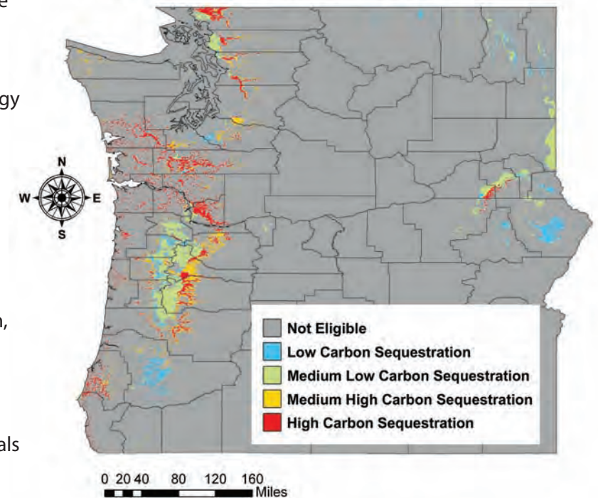
Carbon Sequestration Potential with Hybrid Poplars in Oregon and Washington without Irrigation
