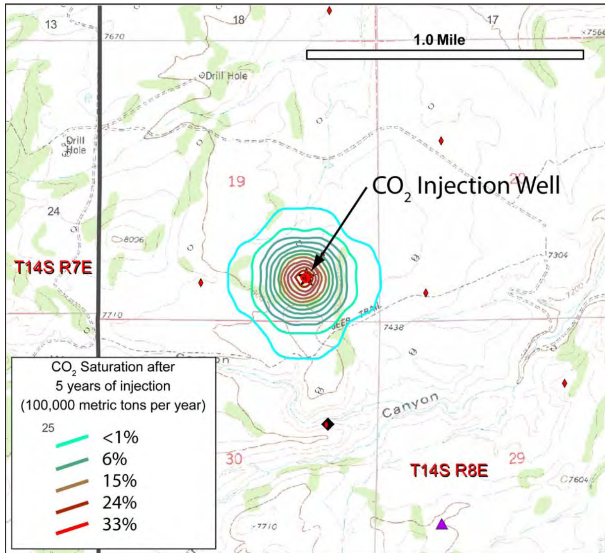
Simulated CO 2 migration within the Navajo Sandstone in the Gordon Creek Field, assuming 5 years of injection, 100,000 metric tons per year. Maximum migration diameter is approximately 0.5 miles.
