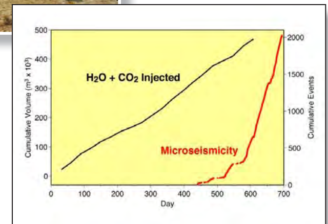
Graph showing correlation between microseismicity and H 2 O + CO 2 injection at the Aneth Oil Field, Utah.
