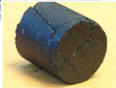
Sample core of coal. (Courtesy of Eric Robertson, INL)
