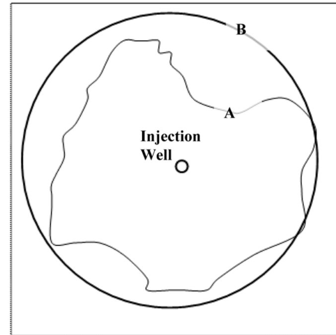
Figure 2: Top-view of injection well and plume area. The area within the irregular shape inside the circle is the areal view of the 3-dimensional CO 2 plume (A). The area inside the larger circle (B) is the accessible pore volume for areal displacement. The areal displacement term, E A = net area contacted by CO 2 (A) / Total area (B).
