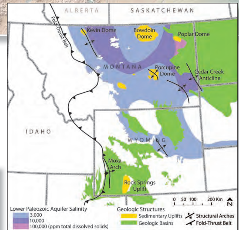
Geologic structures and formation salinity in Montana and Wyoming.
