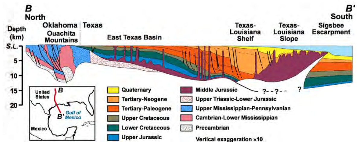
Geologic cross section across the Gulf Coast showing the thick wedge of Cretaceous and Tertiary age sediments that offer numerous large capacity saline formations. Source: Modified from Arbenz (1988), Plate II, cross section D-D' and Salvador (1991), Plate 6, cross section B-B'.
