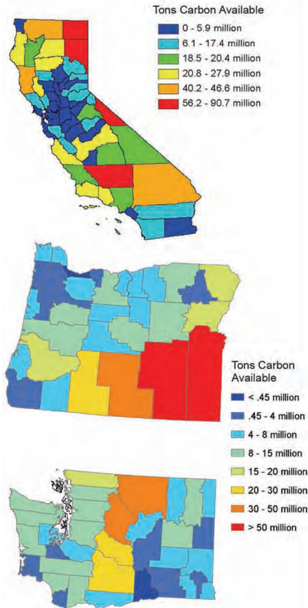
Potential Sequestration Through Afforestation After 40 Years
