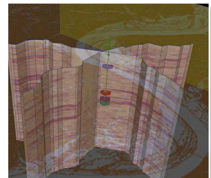
Processed image of 2-D seismic survey transects. Color discs correspond to the top surface of major geologic formations.
