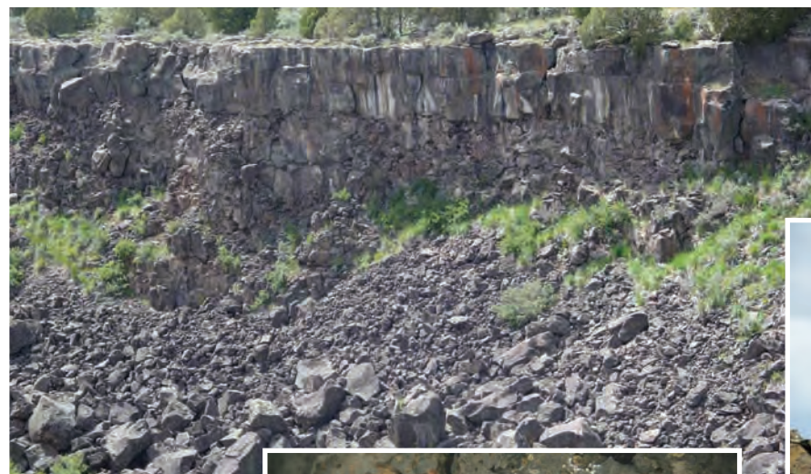
At left, an example of a basalt flow. (Courtesy of Travis McLing, INL)
