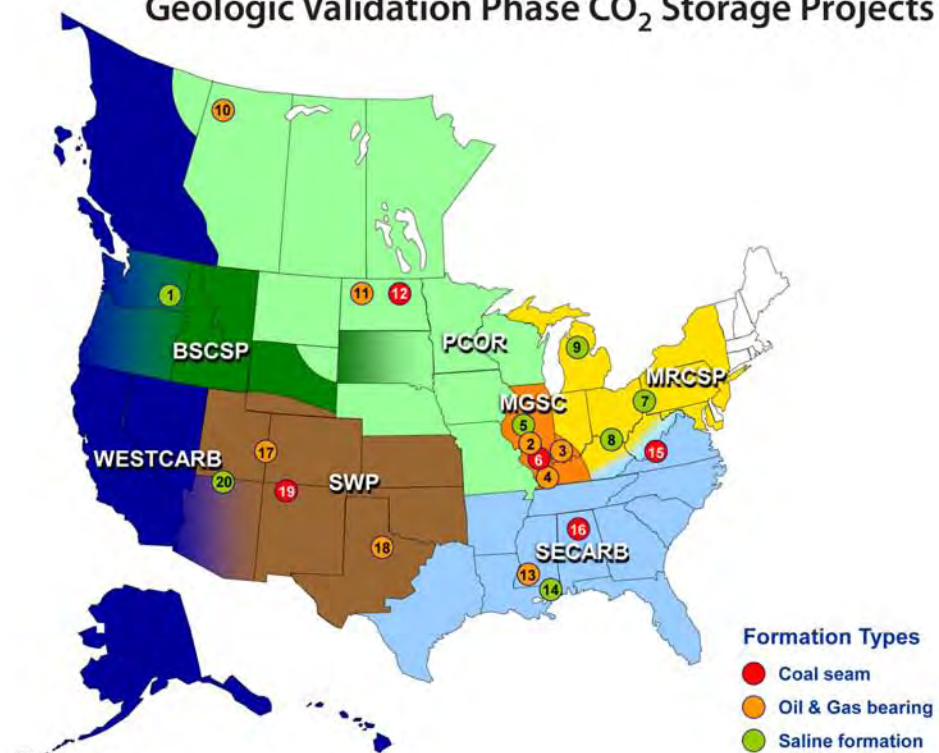
Geologic Validation Phase CO 2 Storage Projects
