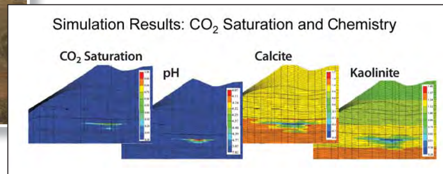
Predictive results for simulation of 100,000 metric tons (110,000 tons) of CO 2 injected into the SACROC field. Diagrams show simulated results 2 months after injection.
