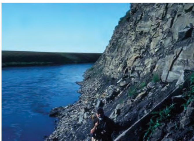
Nanushuk Formation coalbed on the Kukpowruk River, North Slope, Alaska. (Photo courtesy of Gary D. Stricker, USGS)
