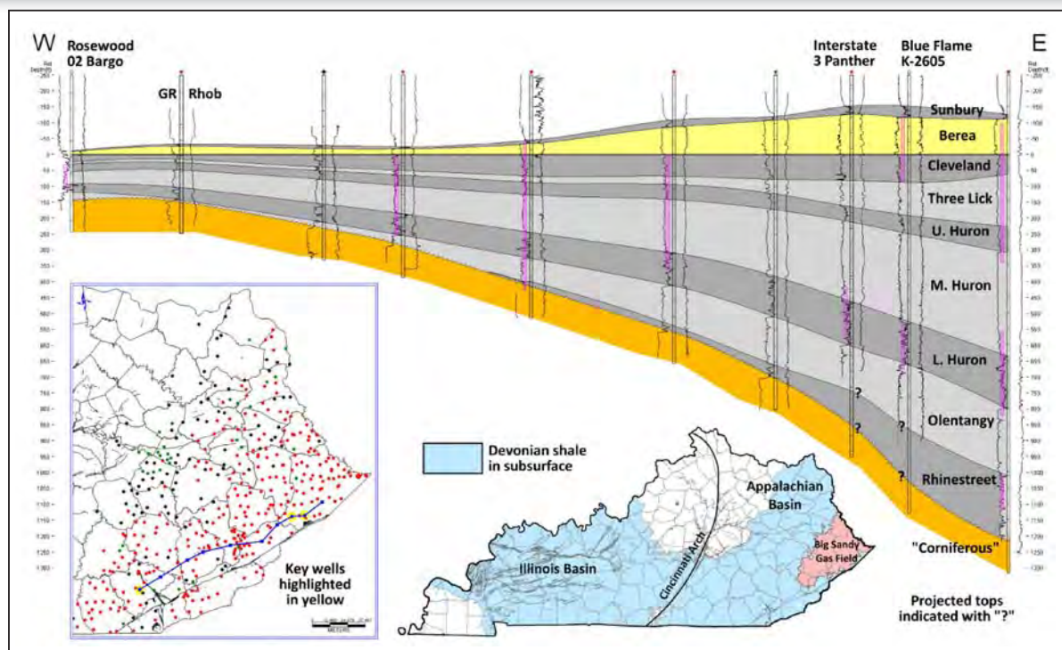
Geologic cross section showing thickening trend of Devonian shales in eastern Kentucky.
