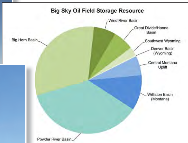
Proportion of CO 2 Storage Resource by Basins in the BSCSP Region.
