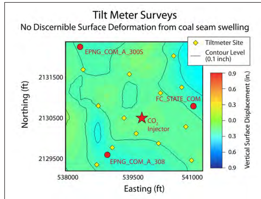
Tilt meter results indicated no systematic surface deformation after injection.
