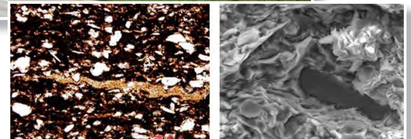
Photomicrograph of shale samples showing organic material.
