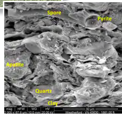
Photomicrograph (2,000X magnification) of black shale, from 1,881 feet deep in Kentucky Geological Survey No. 1 Blan well.
