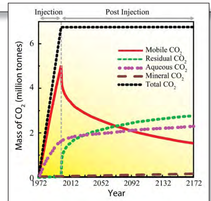
Using known CO 2 injection history from the SACROC field, long-term CO 2 trapping mechanisms were estimated.
