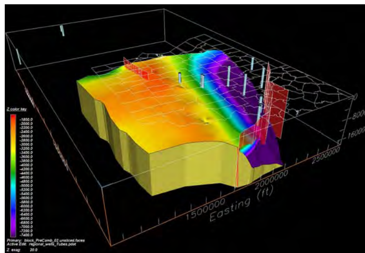
3-D block diagram of deep rock formations and regional 'piggyback' exploration wells.
