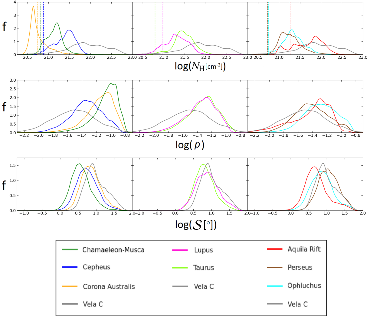
Figure 4. PDFs for each cloud's N_{\text{H}} ( top ), p ( middle ), and S ( bottom ) values on the smoothed scale of 15' FWHM. The y axis in this figure shows the probability density, labelled here as f . Probability density is defined by the area under the curve which it creates: the probability of an x value being lower than a given quantity within the bounds of the curve is equal to the area under the curve to the left of that quantity. Each column displays the data from a specific subset of clouds, divided to increase the clarity of the plots. Vela C is shown in every plot as a reference for comparison. Note that the vertical dashed lines in the N_{\text{H}} PDFs indicate the column density threshold that each clouds sightline must be greater than to be included in our analysis, as displayed in Table 1 and discussed in Section 2.1. The column density N_{\text{H}} PDFs thus include all of each map's sightlines, however only sightlines that passed the selection criteria described in Section 2.1 were used for the p and S PDFs shown in this figure.
