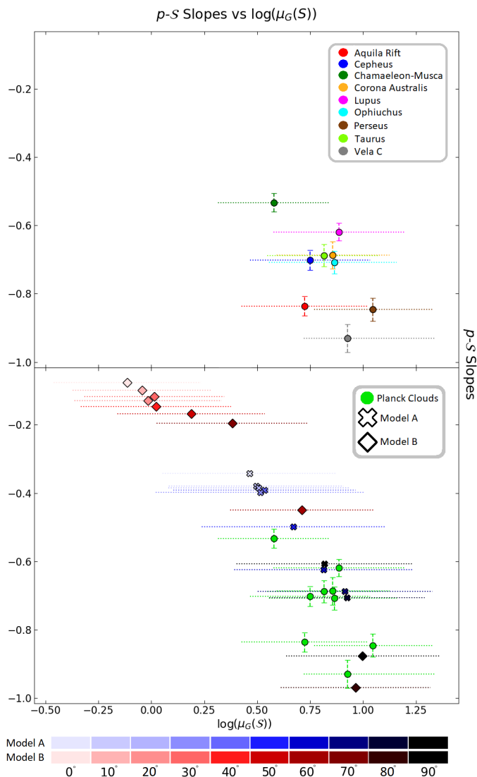
Figure 8. Correspondence between the slope of a cloud’s p vs S relationship and the geometric mean of S (in log scale), for both observed data (top and bottom panels) and those measured from synthetic observations (King et al. 2018; bottom panel) of a more turbulent cloud (Model A; thick plus) and a more magnetically-dominated cloud (Model B; diamonds). The average magnetic field inclination angles for the synthetic observations are represented by the color map depicted beneath the plot, with the inclination angle increasing from 0^\circ to 90^\circ in 10^\circ intervals. The dotted horizontal lines on the x-axis show the MAD of each cloud’s S values and are thus a representation of the distribution of S -values. The error bars on the y axis represent 3\sigma confidence intervals of slope values obtained from bootstrap estimates.
