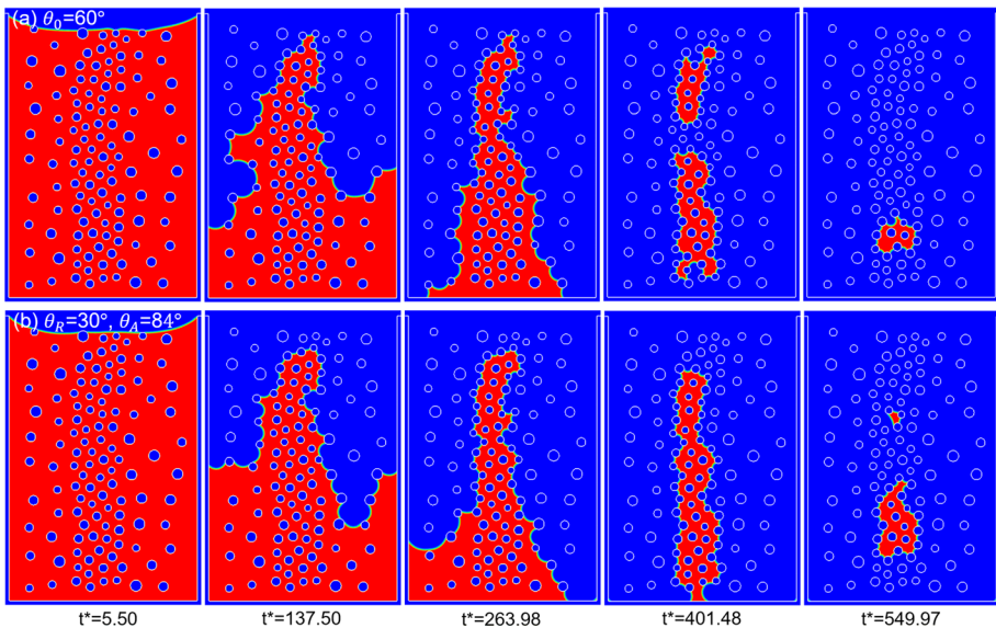
Fig. 13 Drying of a dual-porosity porous medium a using a constant contact angle of \theta_0 = 60^\circ and b considering contact angle hysteresis of ( \theta_R = 30^\circ , \theta_A = 84^\circ ) at different dimensionless time t^* . Subfigures a and b correspond to Supplementary movies 9 and 10, respectively
