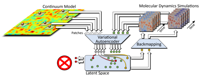
Fig. 10. Multiscale simulation of RAS-membrane biology for cancer research. As the continuum model (left) evolves, patches around the RAS proteins (shaded balls) are projected into a high-dimensional latent space, which is used to drive an importance sampling. Patches that are different from previous simulations (yellow) are used to initialize new MD simulations, whereas patches too close to existing samples (red) are discarded. Significant challenges exist in the analysis of high-dimensional latent spaces to improve the sampling.
