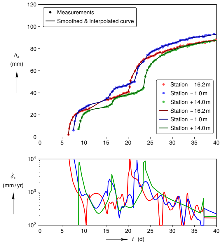
Figure B-7. Room B smoothed and interpolated horizontal closure curves compared against reconstructed mining sequence closure measurements during mining in the top plot. Closure rate curves computed from the smoothed closure curves during mining in the bottom plot.
