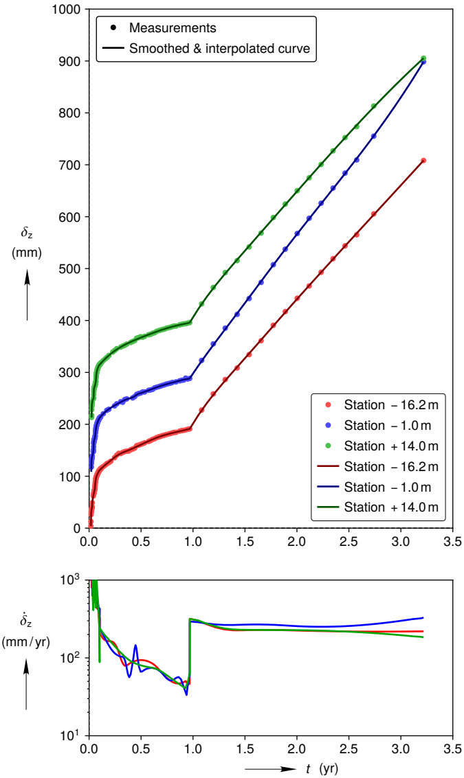
Figure B-10. Room B smoothed and interpolated full vertical closure curves compared against re-constructed mining sequence closure measurements in the top plot. (Each successive station's vertical closure curve and measurements are shifted up by 100 mm to enhance legibility.) Closure rate curves computed from the smoothed closure curves in the bottom plot.
