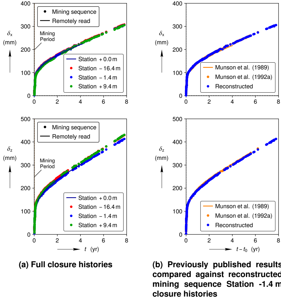
Figure 3-4. Full Room D horizontal and vertical closure histories.
