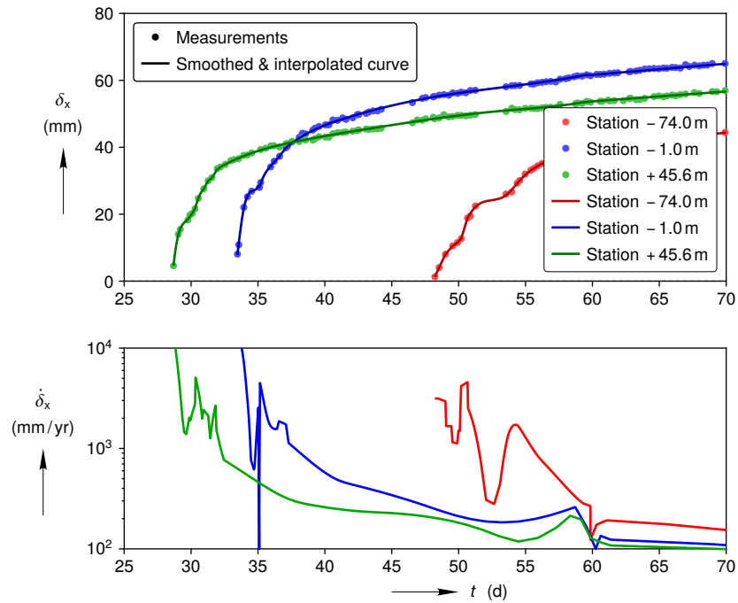
Figure C-7. Room G smoothed and interpolated horizontal closure curves compared against reconstructed mining sequence closure measurements during mining in the top plot. Closure rate curves computed from the smoothed closure curves during mining in the bottom plot.
