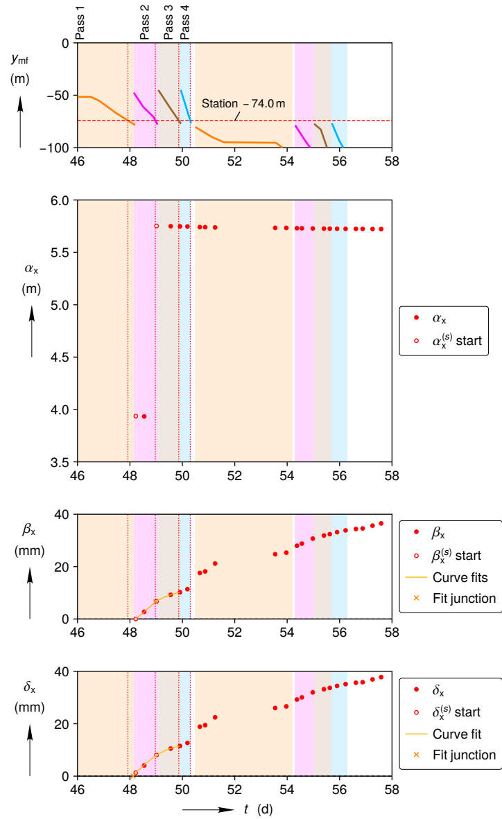
(a) Reconstruction during mining period
