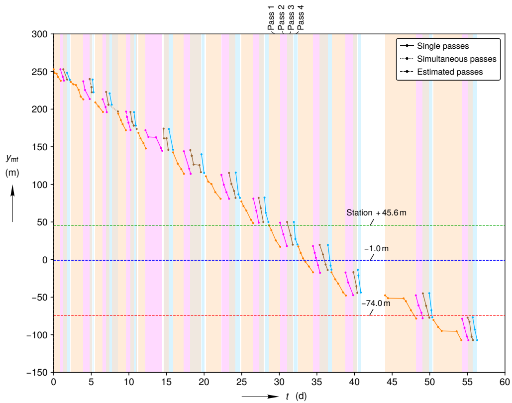
(c) Mining face position
