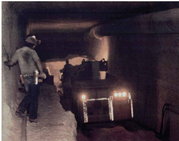
(a) Multi-pass mining of a test room (Munson et al. 1992a)
