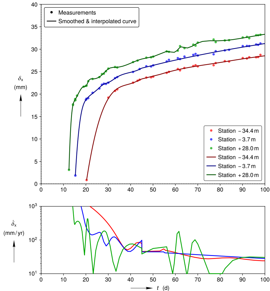
Figure D-7. Room Q smoothed and interpolated horizontal closure curves compared against reconstructed mining sequence closure measurements during mining in the top plot. Closure rate curves computed from the smoothed closure curves during mining in the bottom plot.
