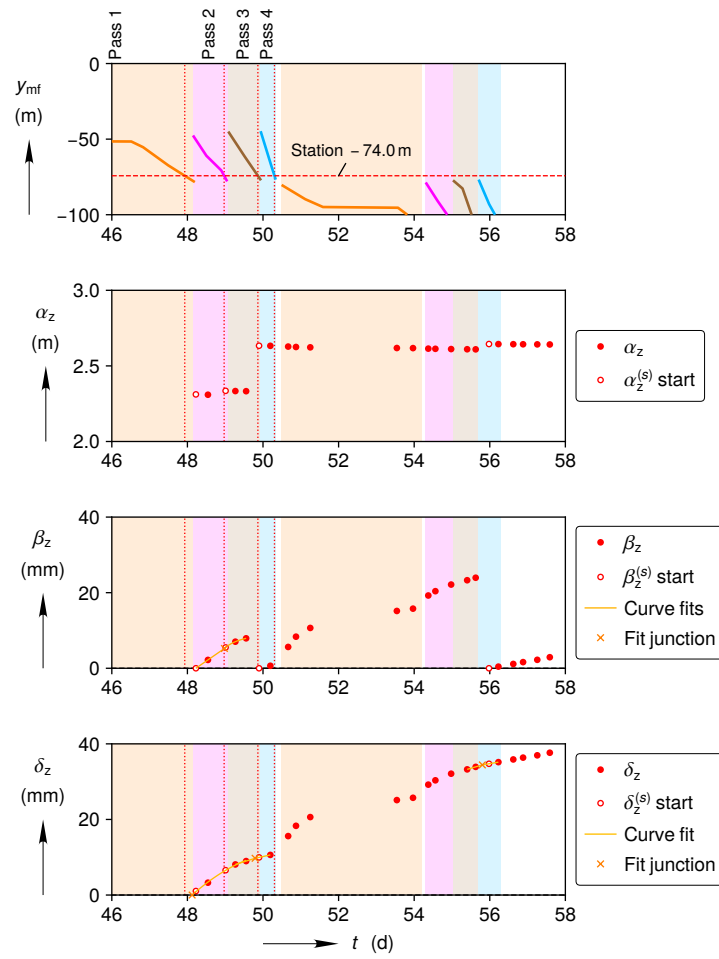
(a) Reconstruction during mining period
