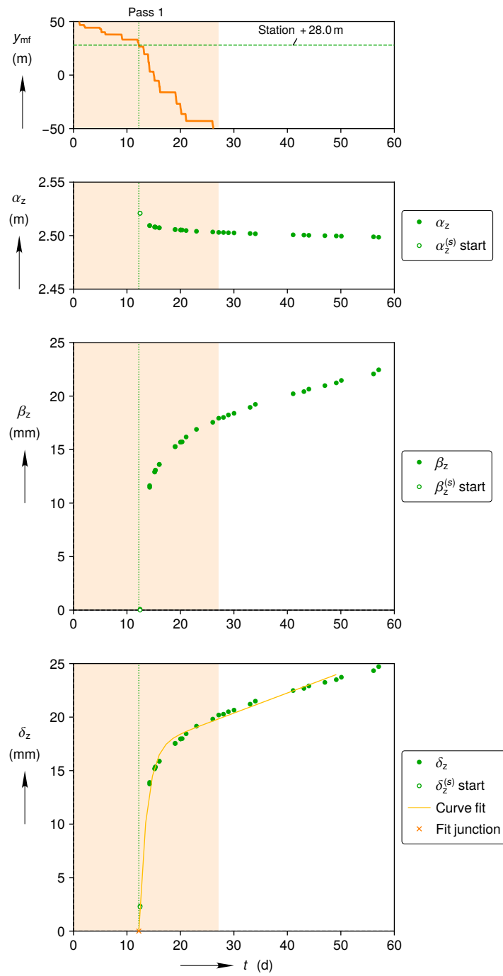
(a) Reconstruction during mining period
