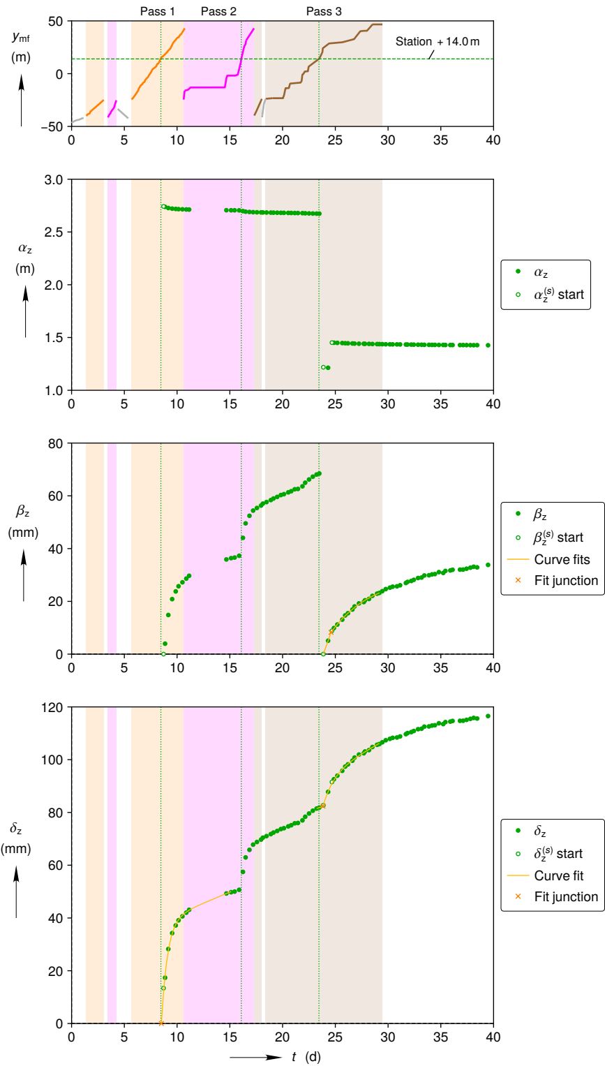
(a) Reconstruction during mining period
