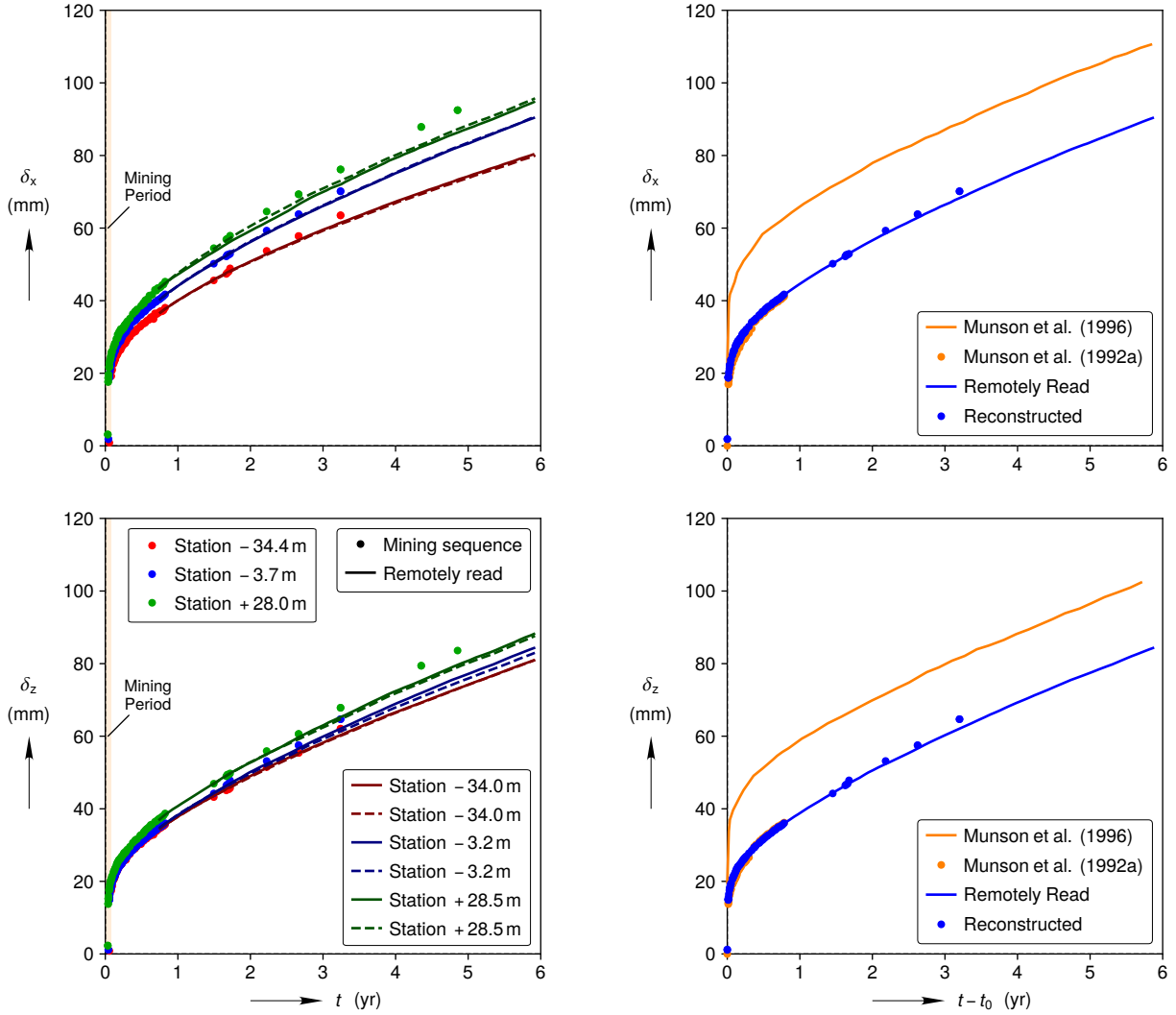
(a) Mining sequence and remotely read closure histories
