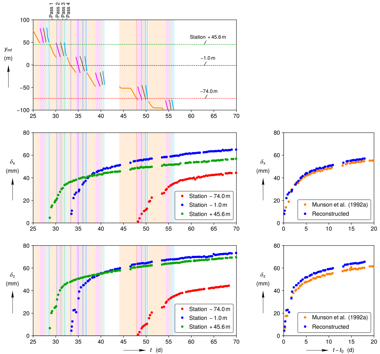
(a) Mining face position and mining sequence closure histories (b) Previously published results compared against reconstructed mining sequence Station -1.0 m closure histories
