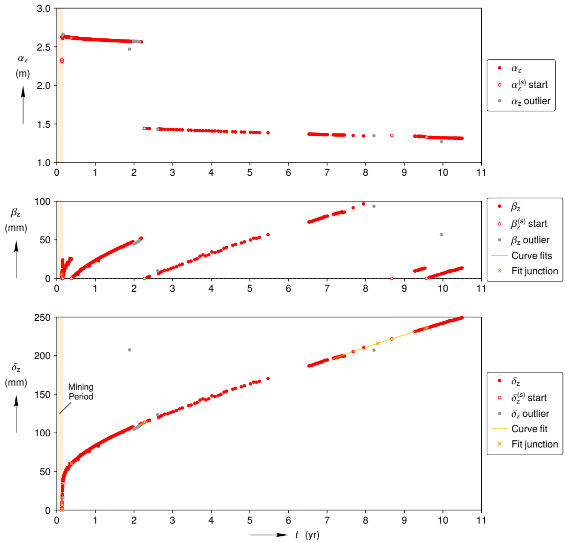
(b) Full reconstruction
