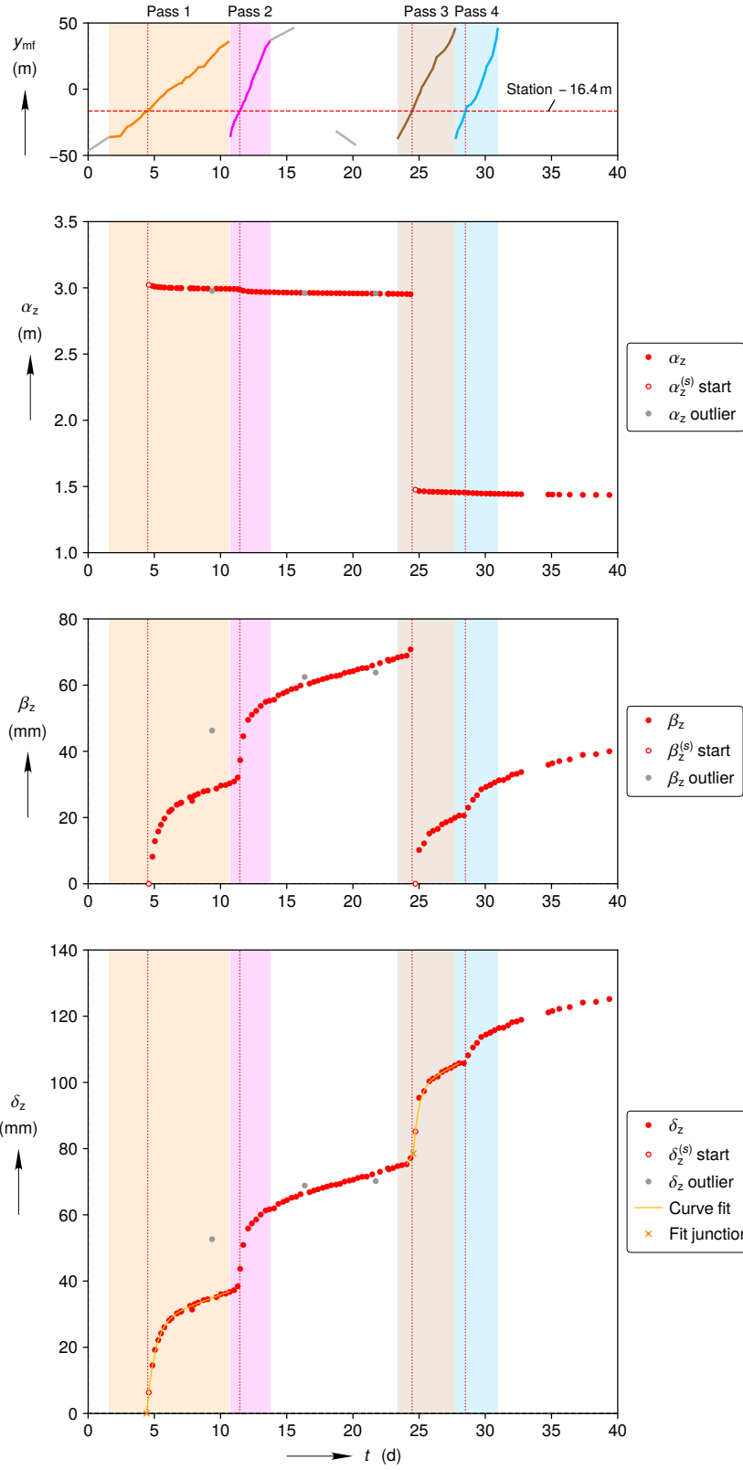
(a) Reconstruction during mining period
