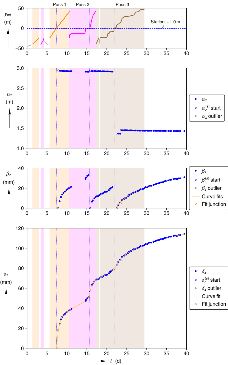
(a) Reconstruction during mining period
