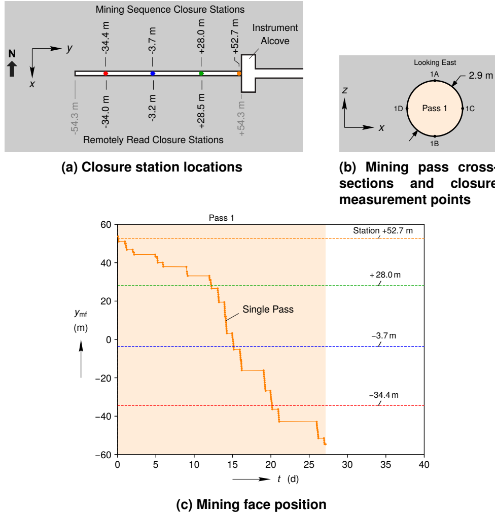
Figure 3-13. Room Q plan view, mining cross-section, and mining face position. The mining face position is derived from Fig. 2.2.23 in Munson et al. (1992a).
