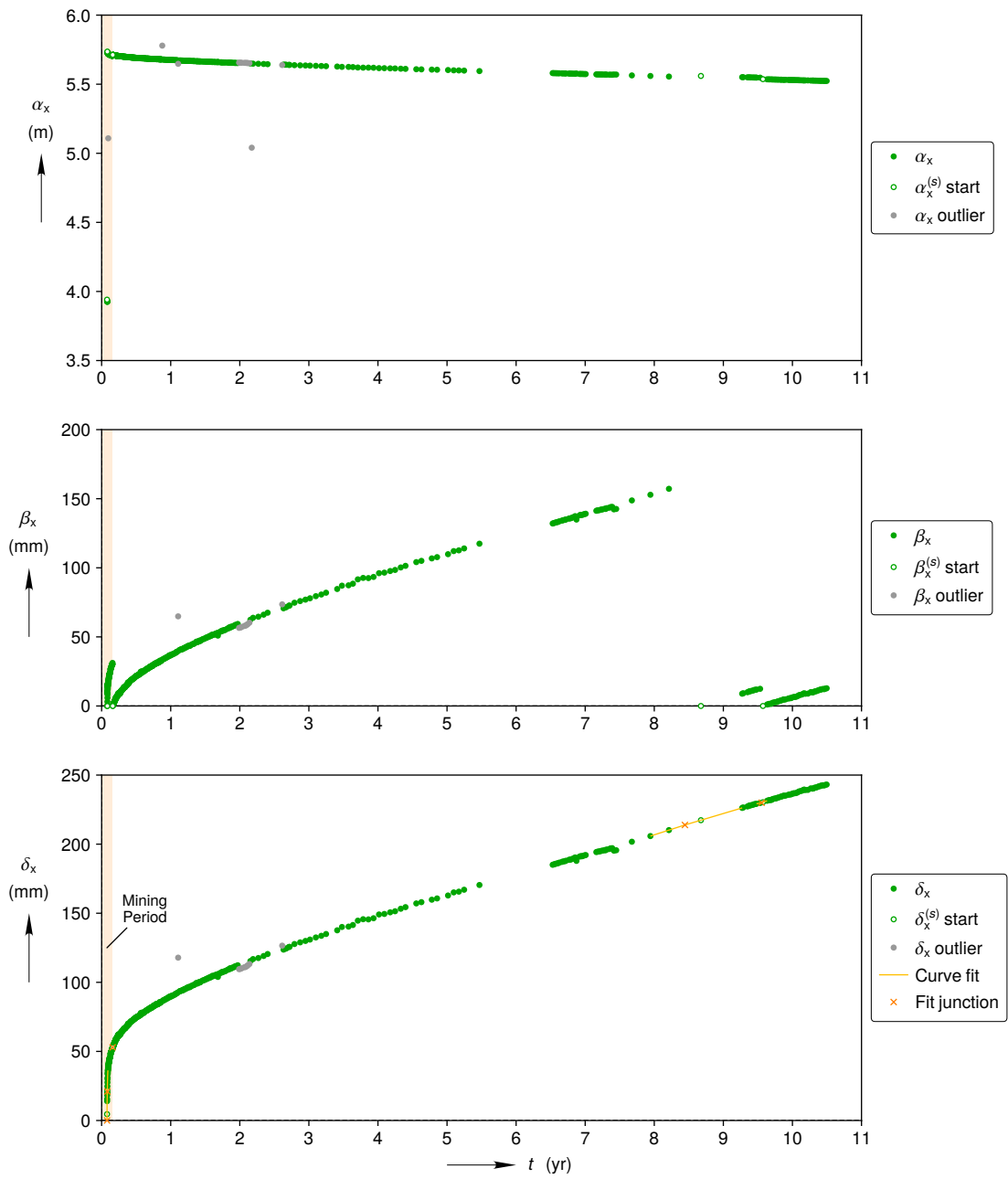
(b) Full reconstruction
