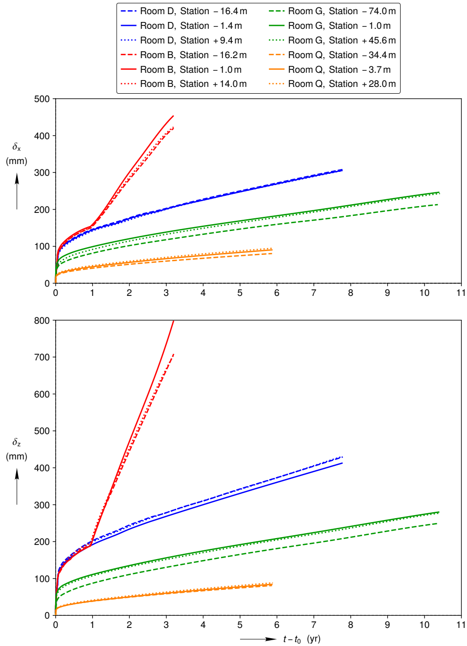
Figure 3-16. Room D, B, G, and Q horizontal (top plot) and vertical (bottom plot) smoothed and interpolated closure histories compared.
