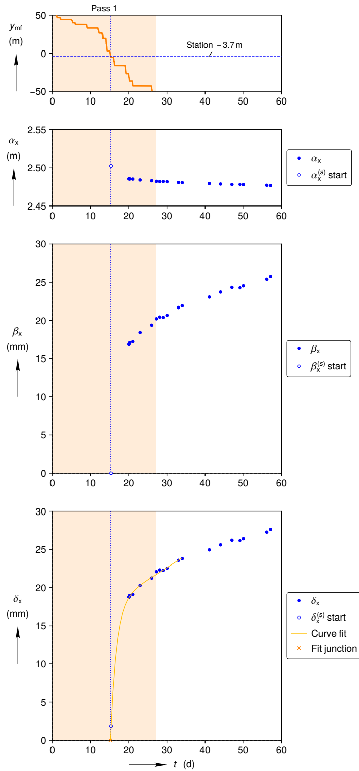
(a) Reconstruction during mining period
