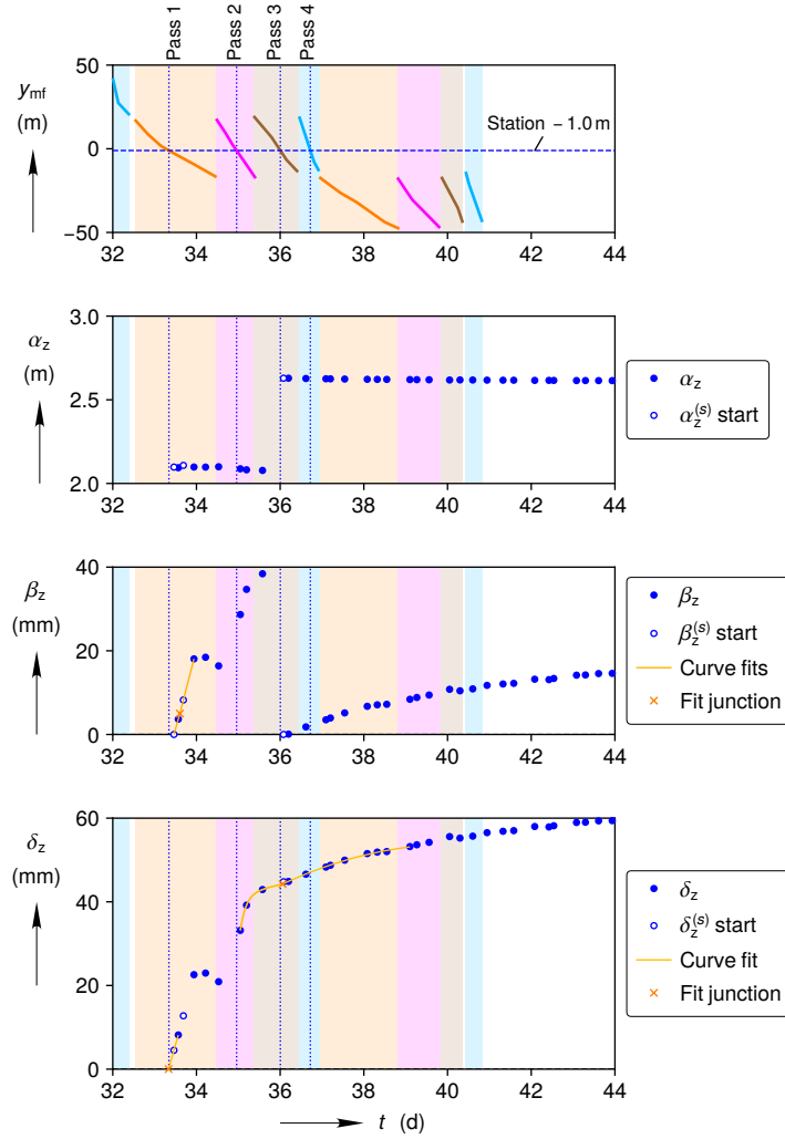
Figure 3-10. Early Room G mining sequence Station -1.0 m vertical closure reconstruction process.
