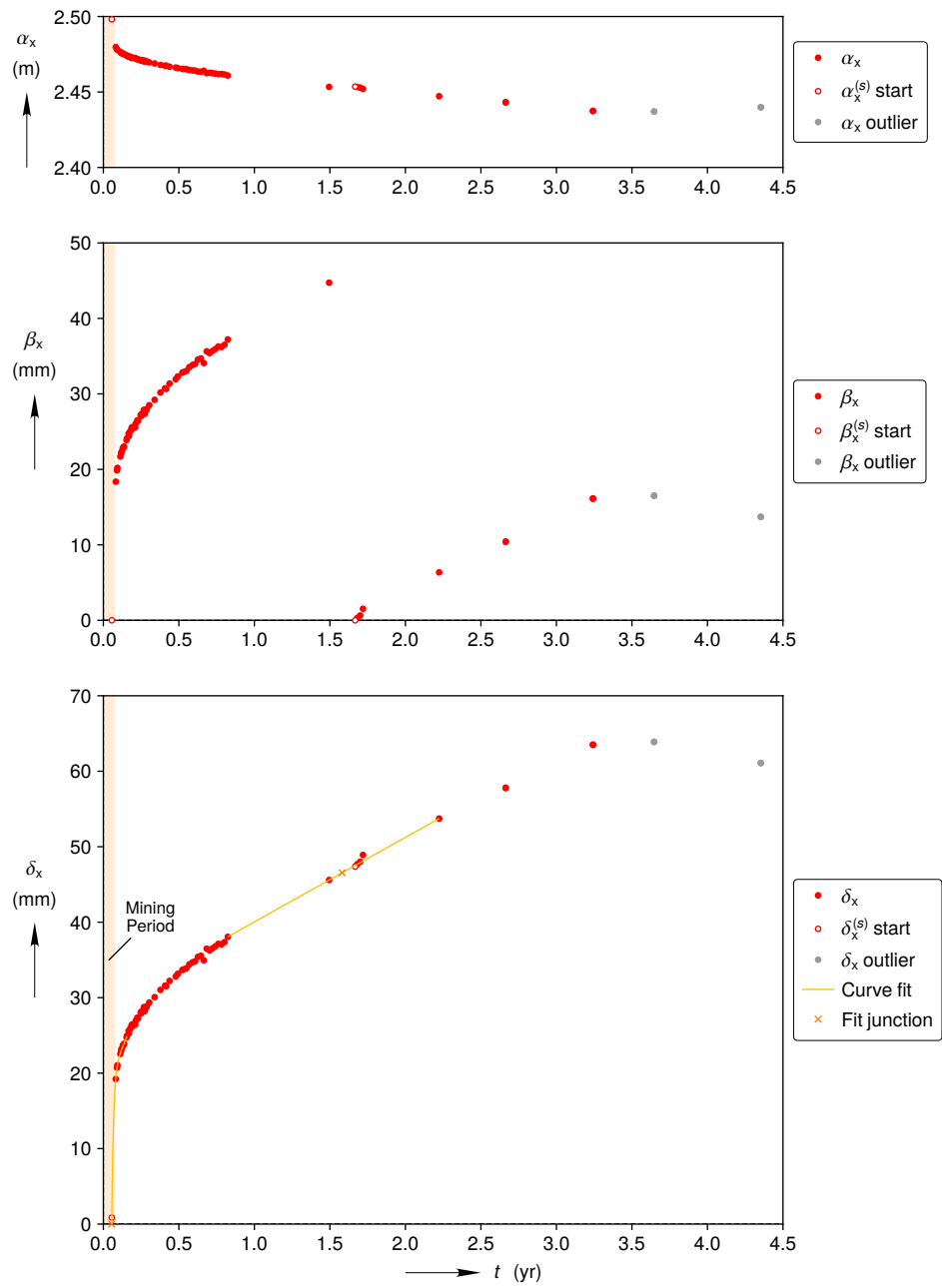
(b) Full reconstruction
