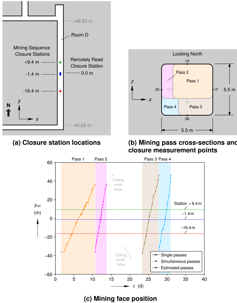
Figure 3-1. Room D plan view, mining cross-section, and mining face position. The mining cross-section and mining face position were respectively derived from Fig. 2.2.12 and 2.2.13 in Munson et al. (1992a).
