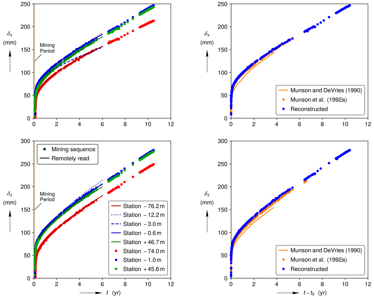
(a) Mining sequence and remotely read closure histories
