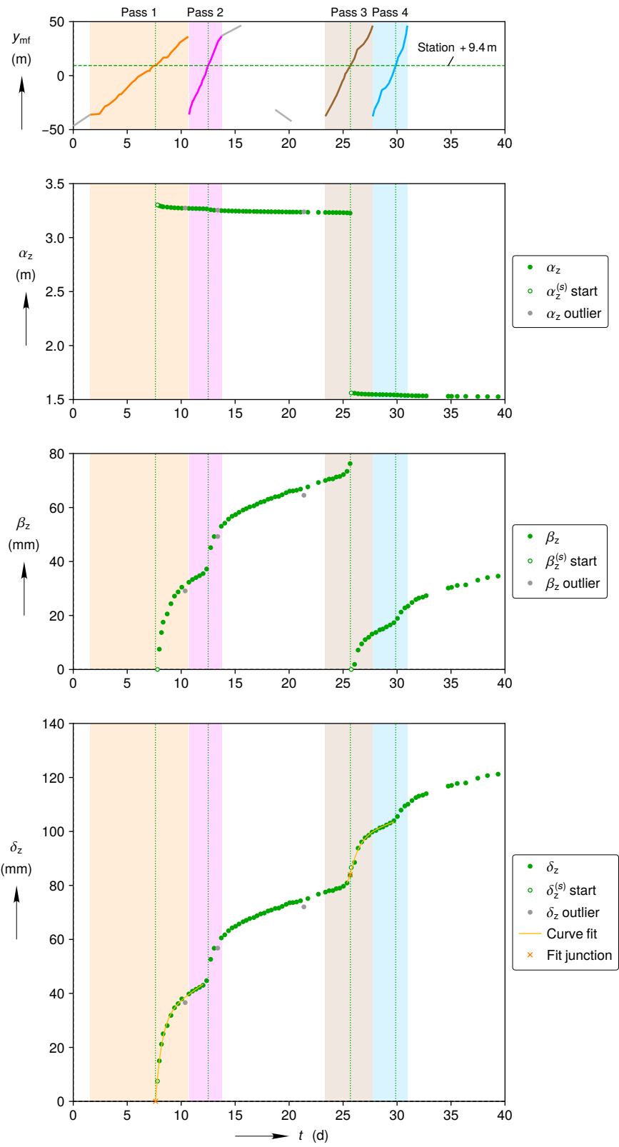
(a) Reconstruction during mining period
