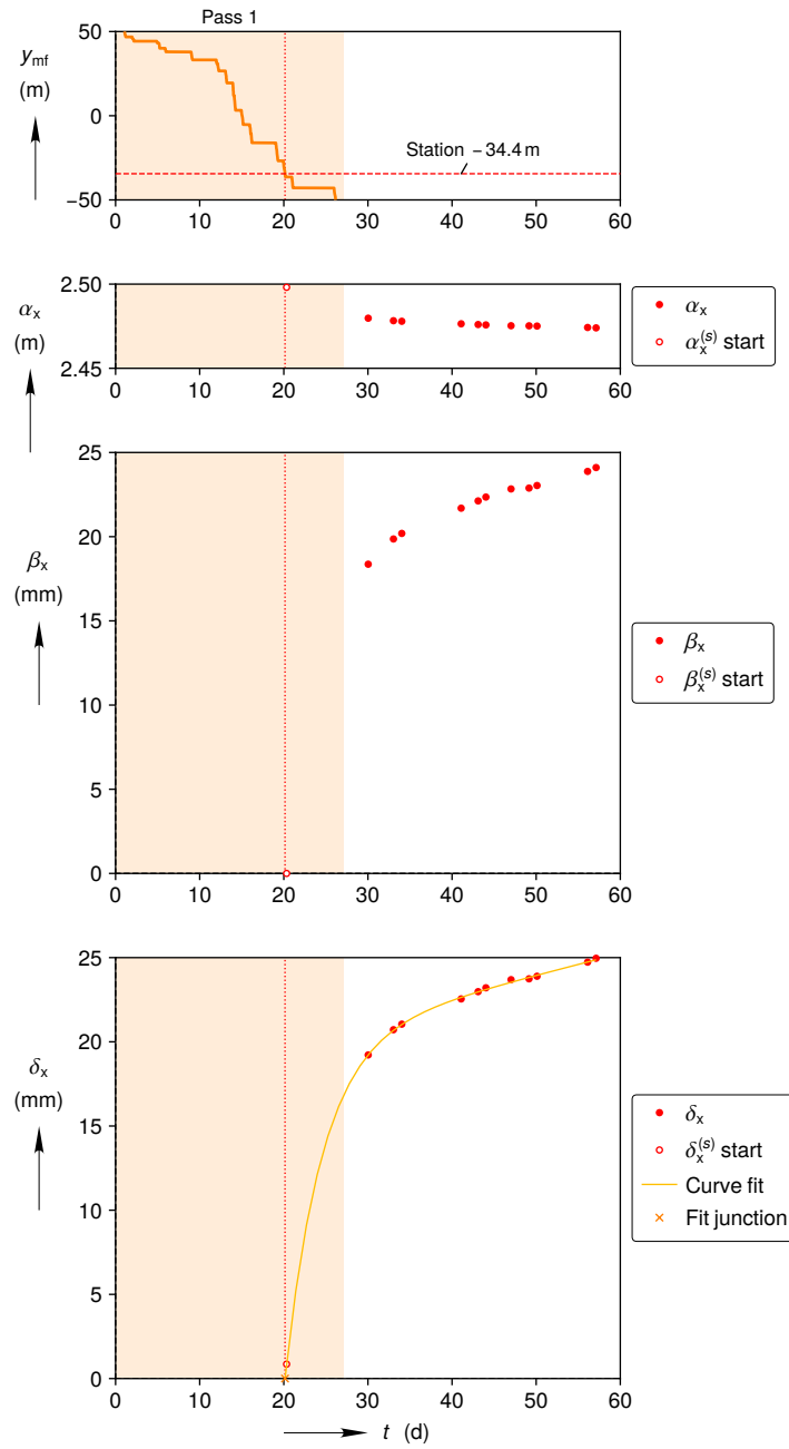
(a) Reconstruction during mining period
