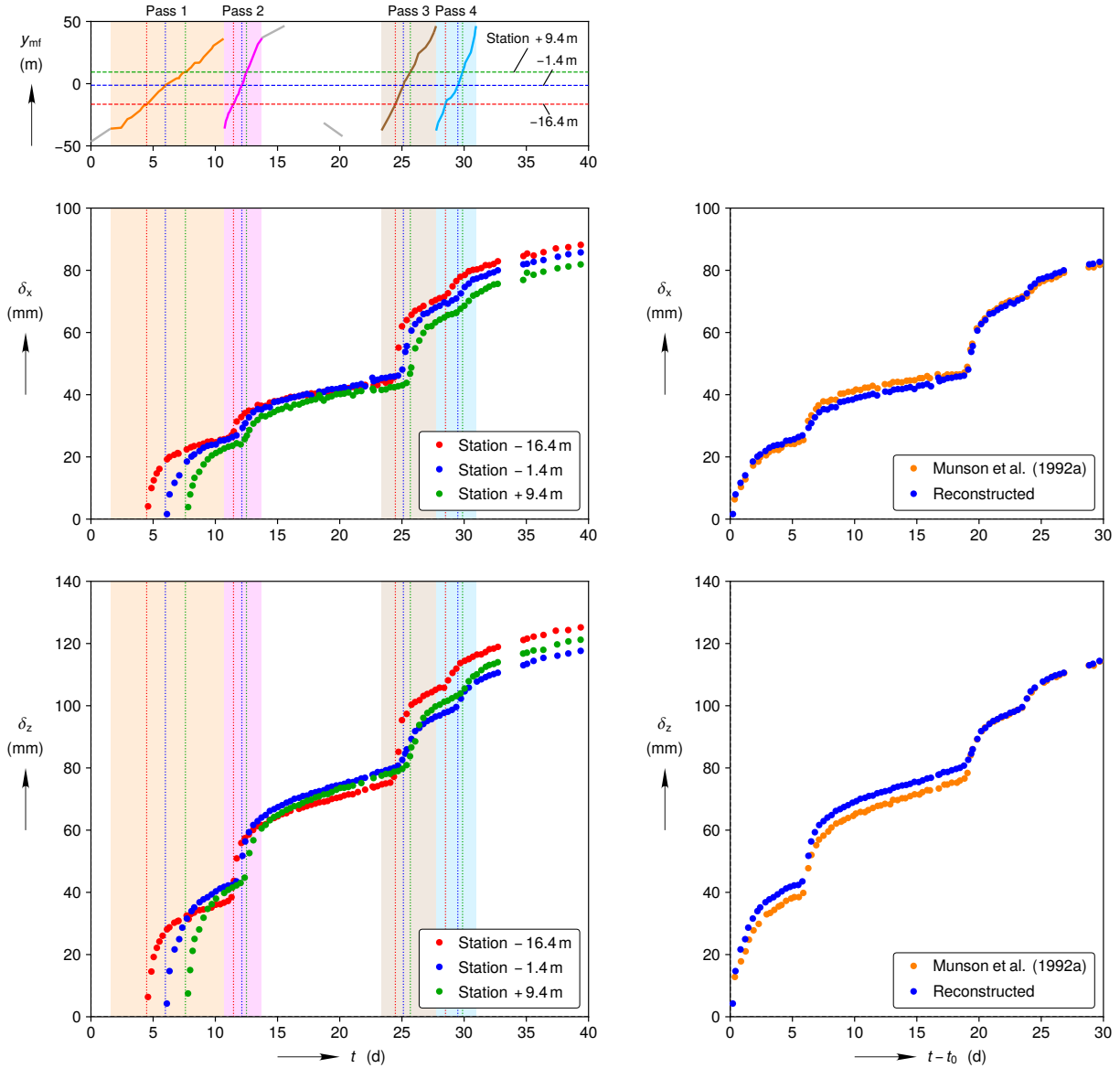
(a) Mining face position and mining sequence closure histories
