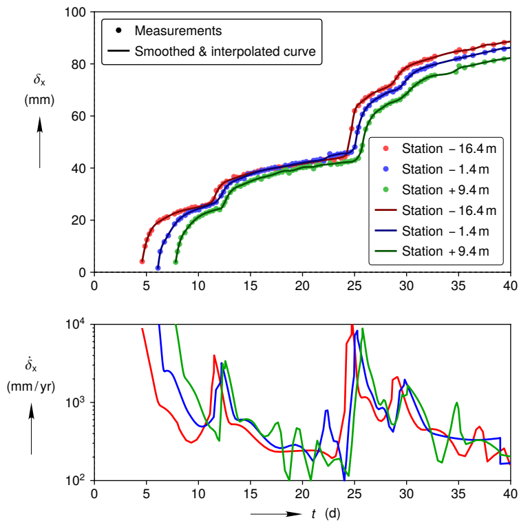
Figure A-7. Room D smoothed and interpolated horizontal closure curves compared against reconstructed mining sequence closure measurements during mining in the top plot. Closure rate curves computed from the smoothed closure curves during mining in the bottom plot.
