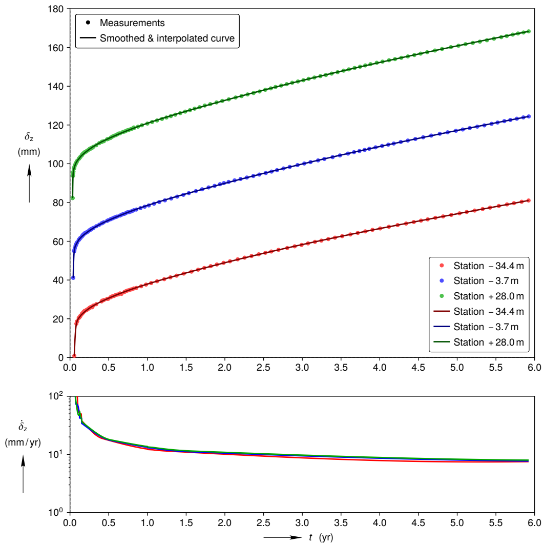
Figure D-10. Room Q smoothed and interpolated full vertical closure curves compared against spliced together mining sequence and remotely read closure measurements in the top plot. (Each successive station's vertical closure curve and measurements are shifted up by 40 mm to enhance legibility.) Closure rate curves computed from the smoothed closure curves in the bottom plot.
