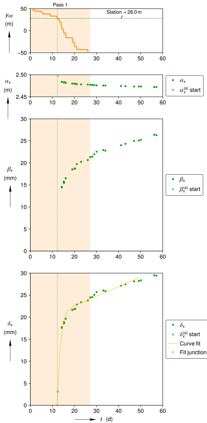
(a) Reconstruction during mining period
