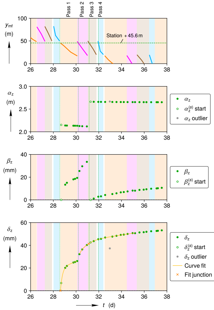
(a) Reconstruction during mining period
