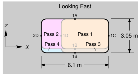
(b) Mining pass cross-sections and closure measurement points
