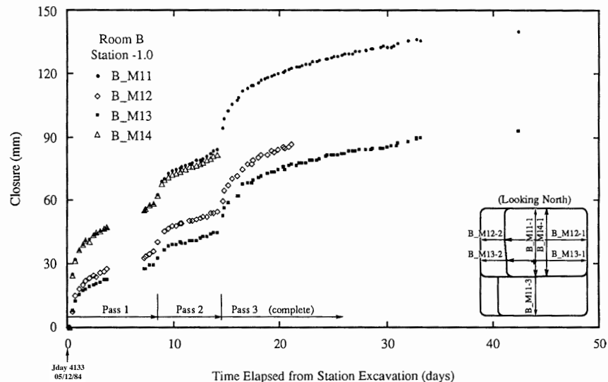
Figure 1-4. Room B Station -1.0 m early mining sequence closure measurements (Fig. 5.2.1b in Munson et al. (1992a)).
