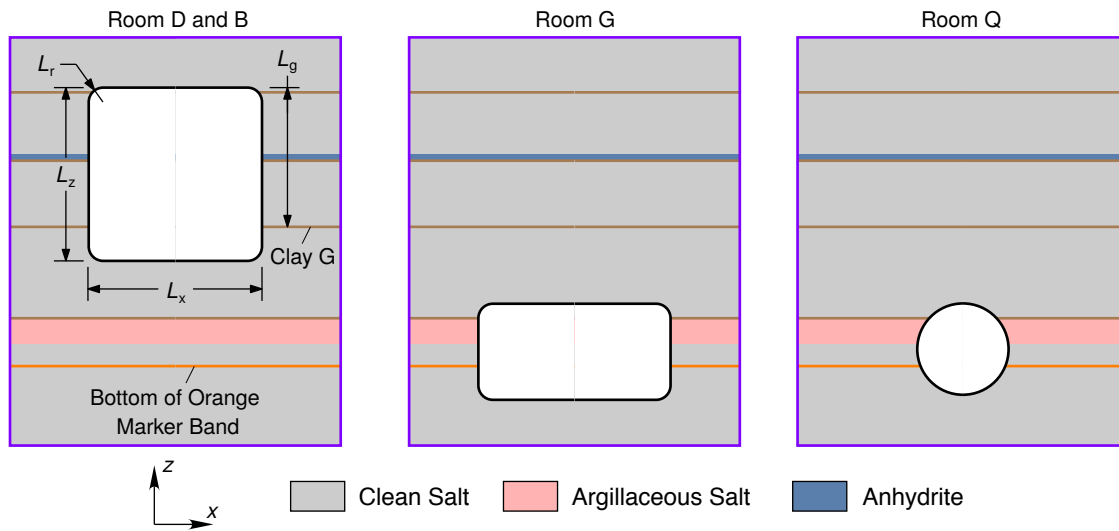
Figure 1-2. Rooms D, B, G, and Q nominal initial cross-sectional geometries and locations.
