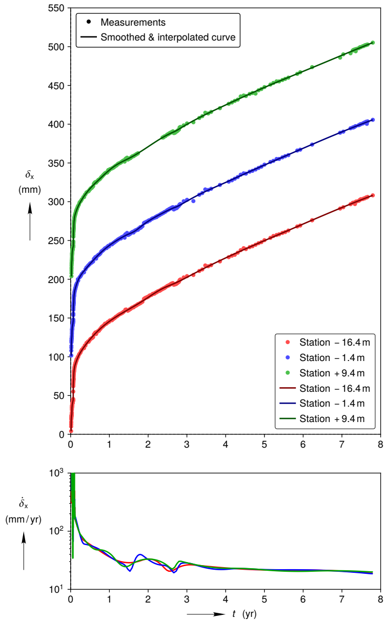
Figure A-8. Room D smoothed and interpolated full horizontal closure curves compared against reconstructed mining sequence closure measurements in the top plot. (Each successive station's horizontal closure curve and measurements are shifted up by 100 mm to enhance legibility.) Closure rate curves computed from the smoothed closure curves in the bottom plot.
