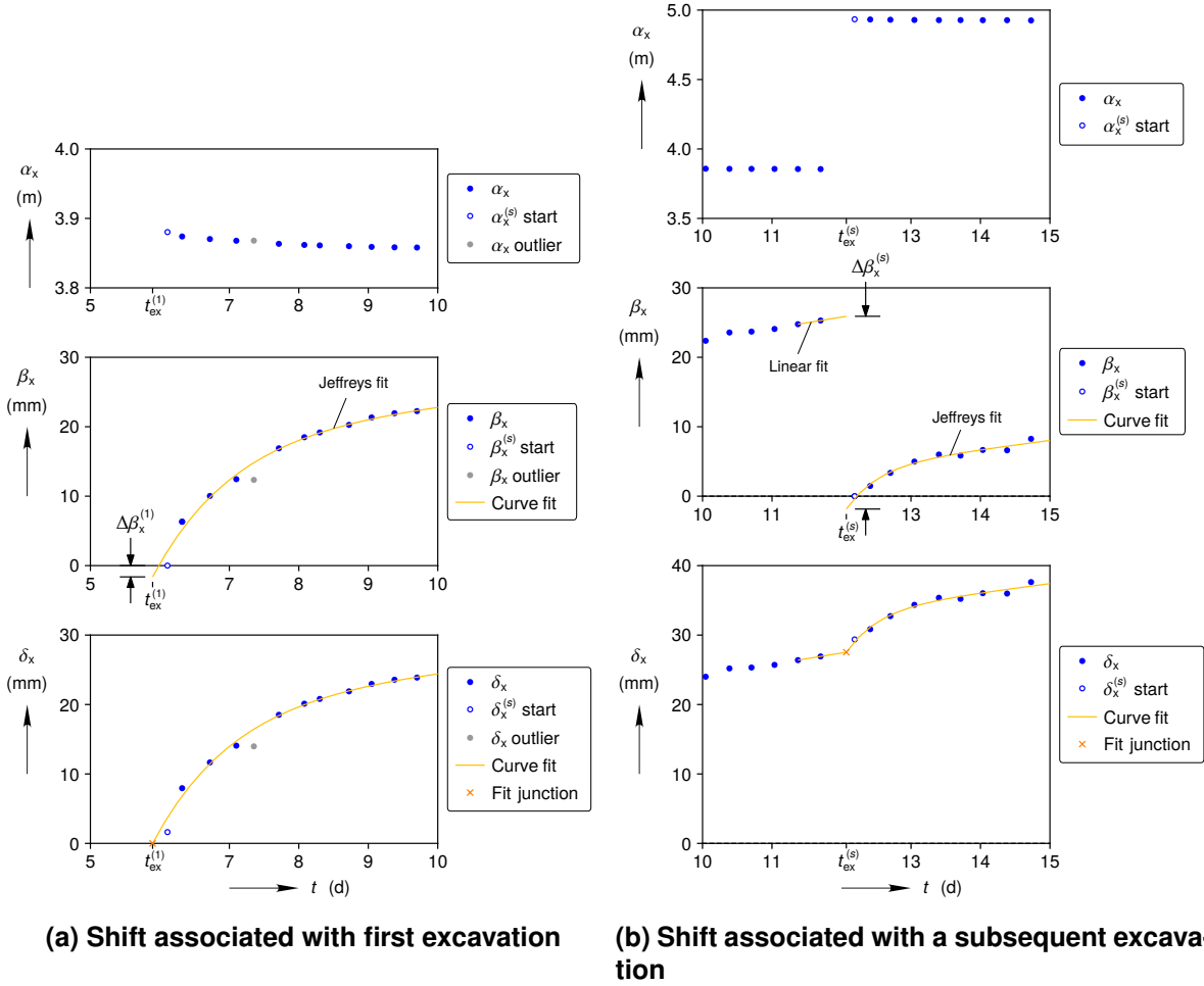
Figure 2-4. Examples of closure segment shifts.
