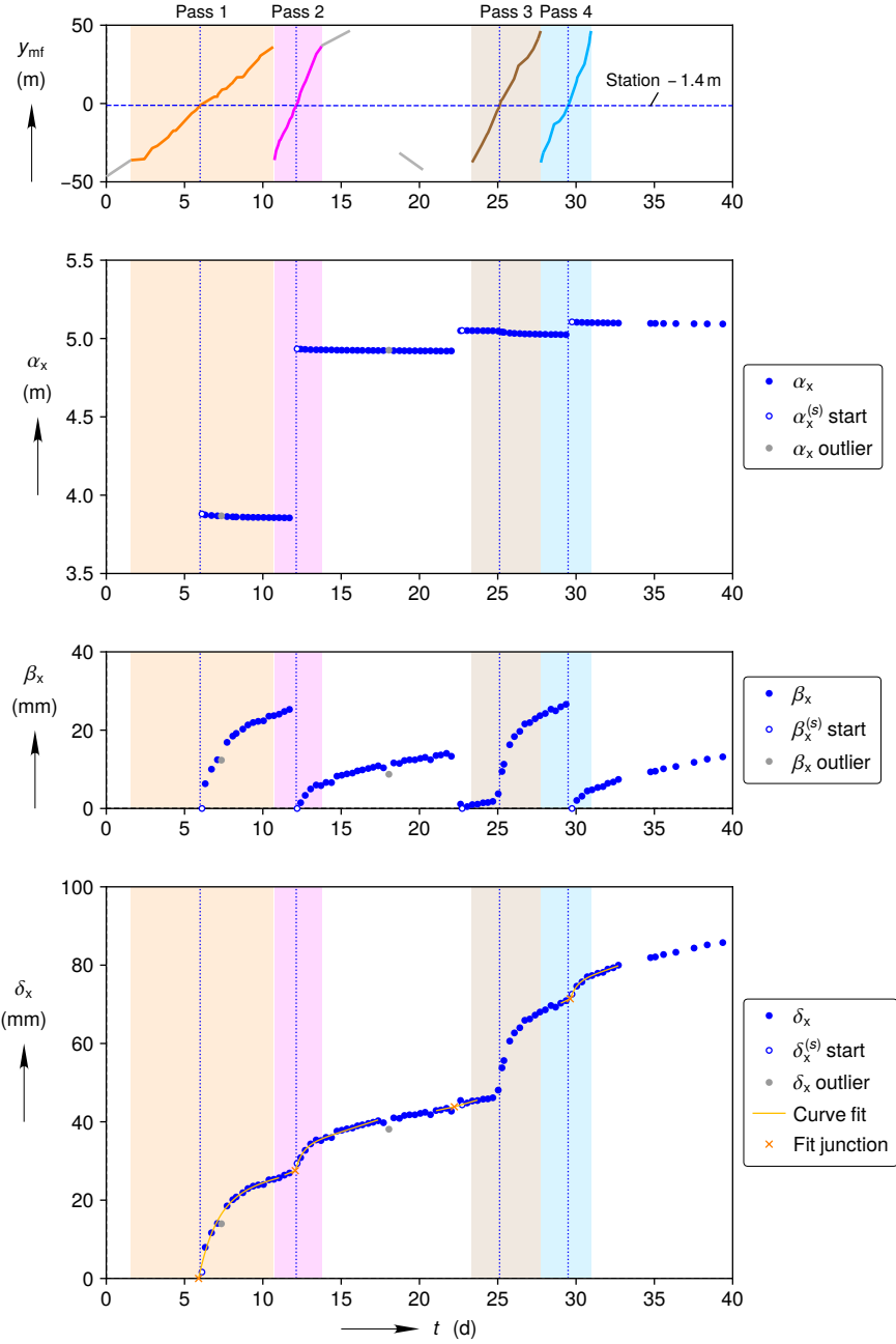
Figure 3-2. Room D mining sequence station -1.4 m horizontal closure reconstruction process during mining.
