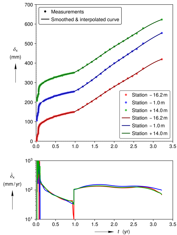
Figure B-8. Room B smoothed and interpolated full horizontal closure curves compared against reconstructed mining sequence closure measurements in the top plot. (Each successive station's horizontal closure curve and measurements are shifted up by 100 mm to enhance legibility.) Closure rate curves computed from the smoothed closure curves in the bottom plot.
