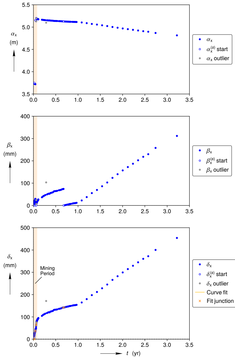
(b) Full reconstruction
