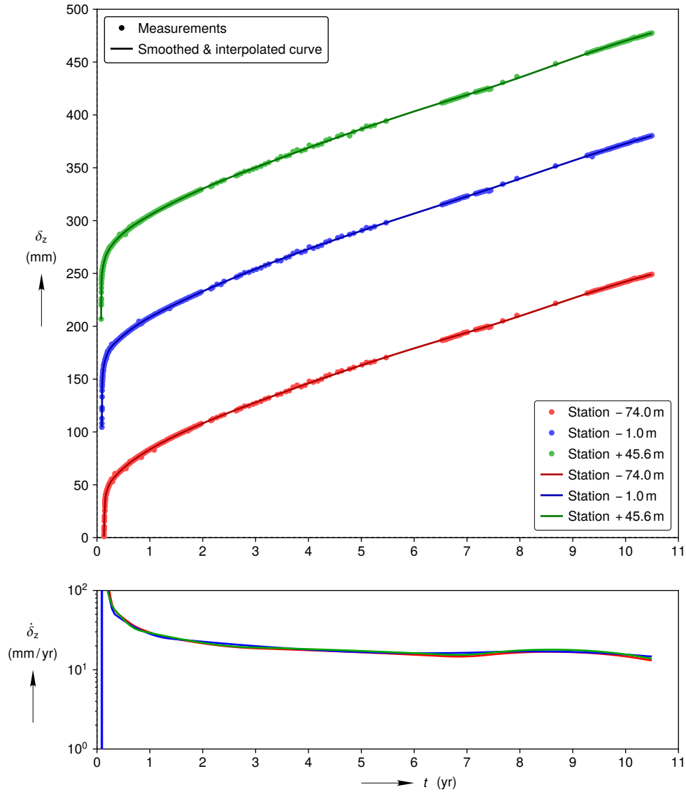
Figure C-10. Room G smoothed and interpolated full vertical closure curves compared against re-constructed mining sequence closure measurements in the top plot. (Each successive station's vertical closure curve and measurements are shifted up by 100 mm to enhance legibility.) Closure rate curves computed from the smoothed closure curves in the bottom plot.
