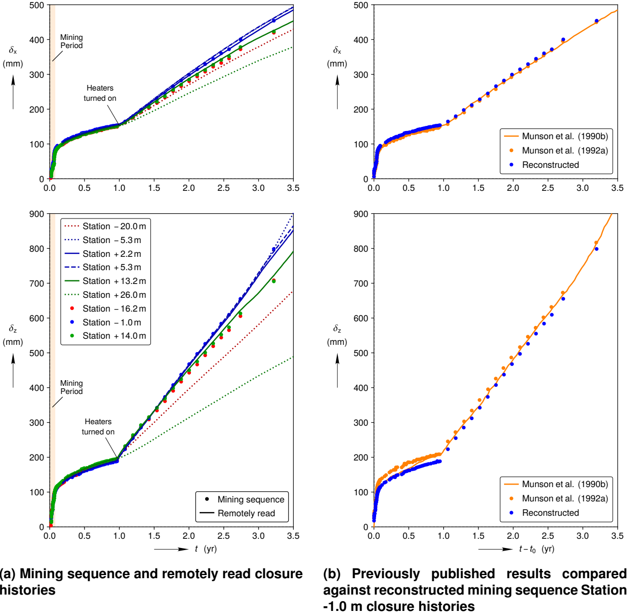
Figure 3-8. Full Room B horizontal and vertical closure histories.
