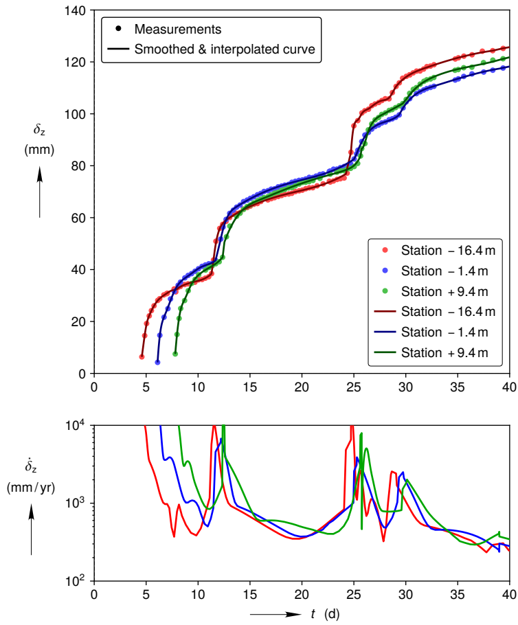
Figure A-9. Room D smoothed and interpolated vertical closure curves compared against reconstructed mining sequence closure measurements during mining in the top plot. Closure rate curves computed from the smoothed closure curves during mining in the bottom plot.
