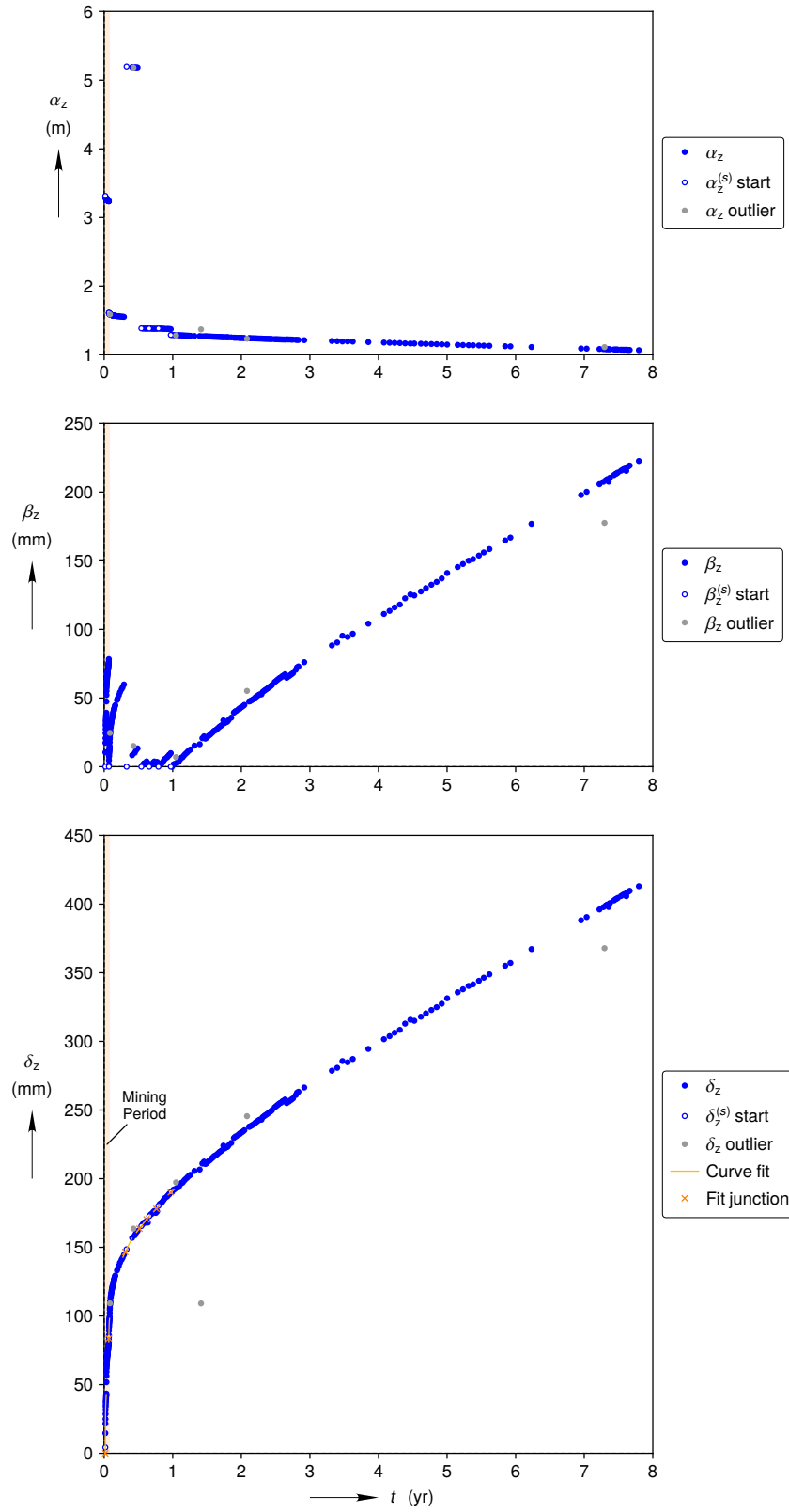
(b) Full reconstruction
