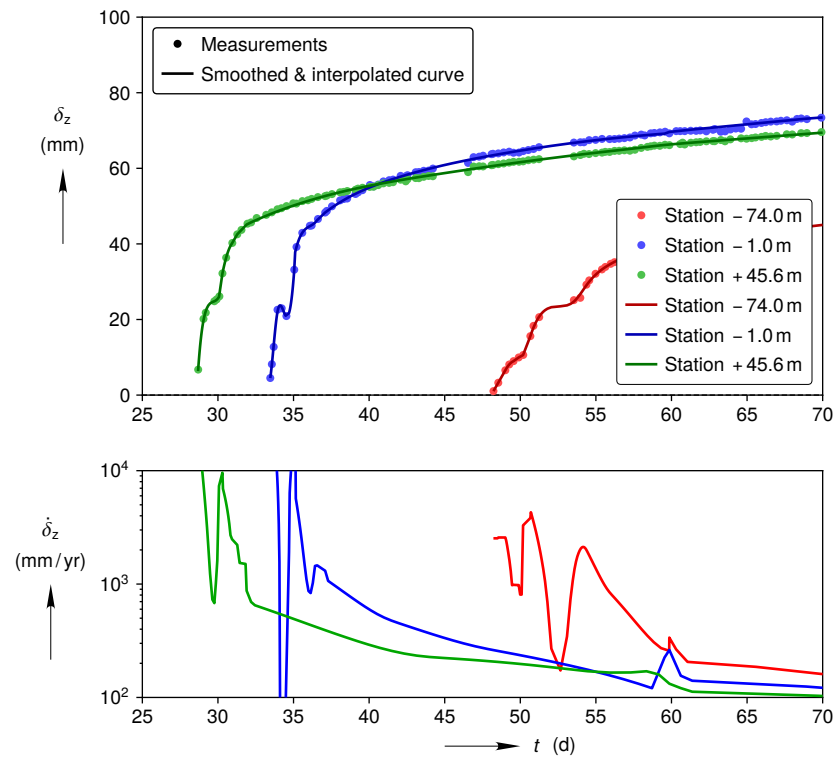
Figure C-9. Room G smoothed and interpolated vertical closure curves compared against reconstructed mining sequence closure measurements during mining in the top plot. Closure rate curves computed from the smoothed closure curves during mining in the bottom plot.
