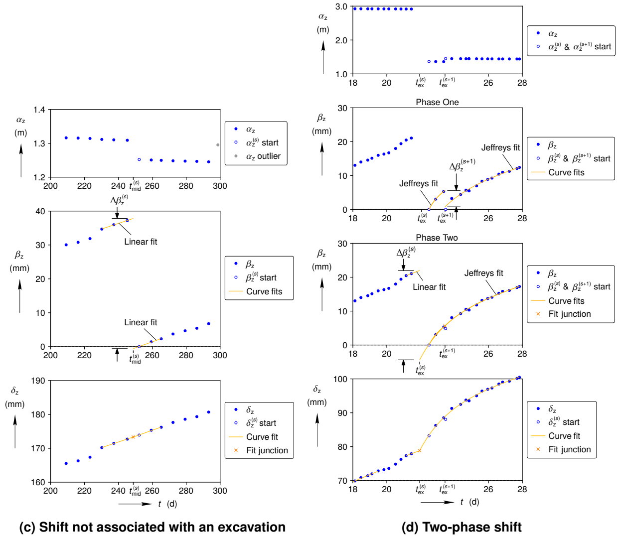
Figure 2-4. (Continued) Examples of closure segment shifts.
