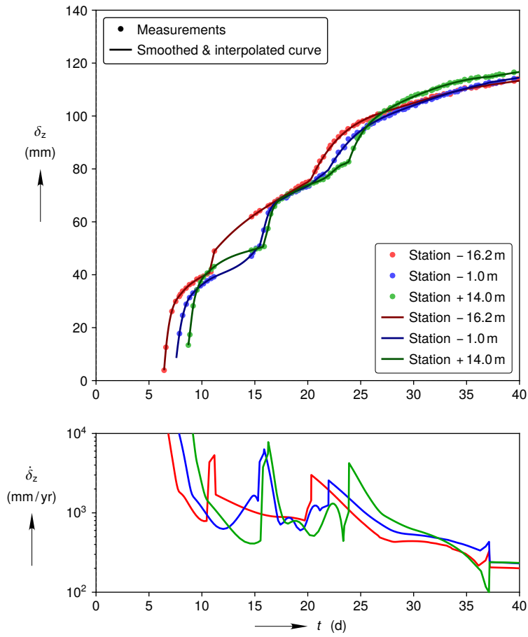
Figure B-9. Room B smoothed and interpolated vertical closure curves compared against reconstructed mining sequence closure measurements during mining in the top plot. Closure rate curves computed from the smoothed closure curves during mining in the bottom plot.
