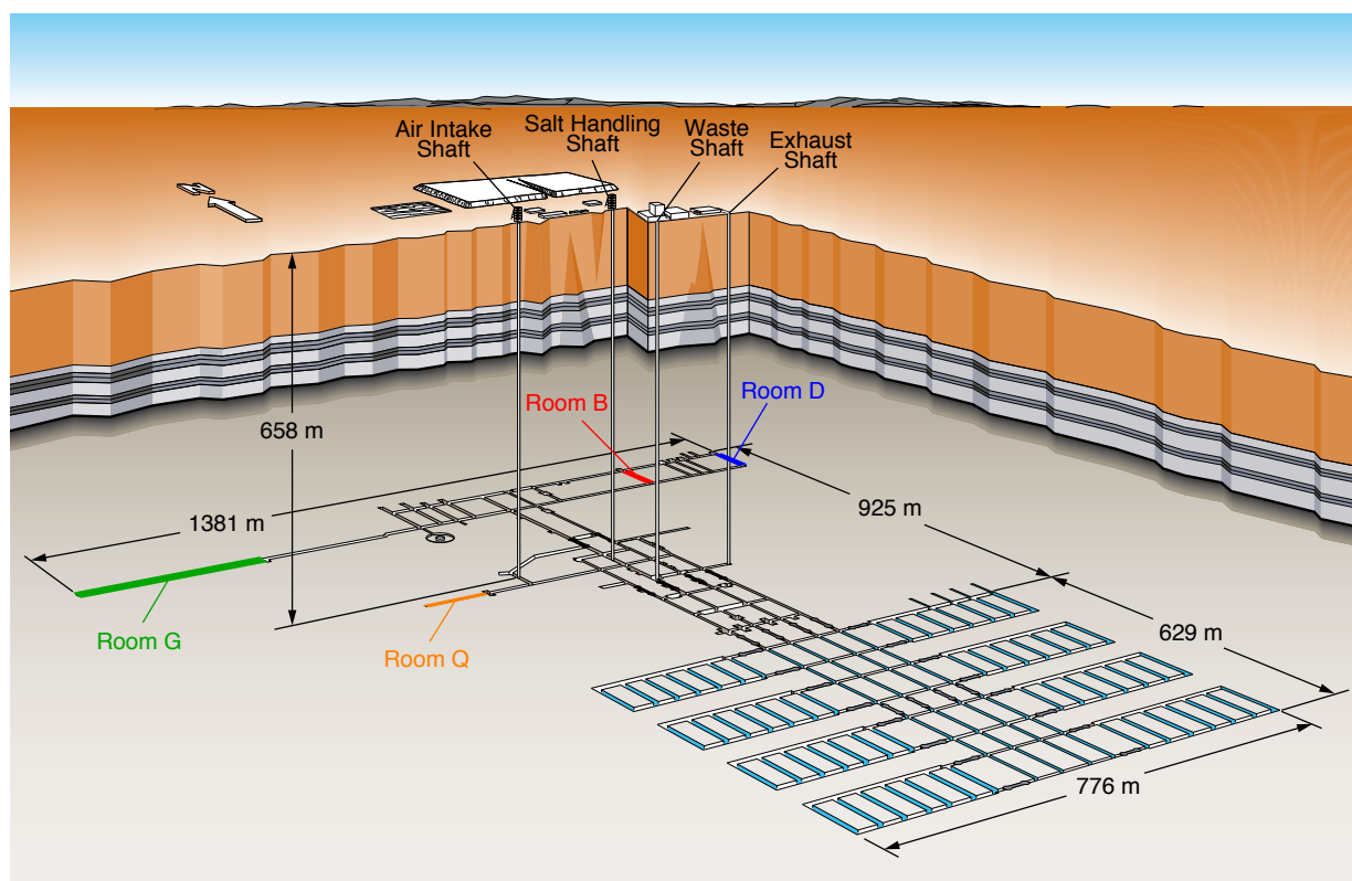
Figure 1-1. WIPP layout showing the location of Rooms D, B, G, and Q.
