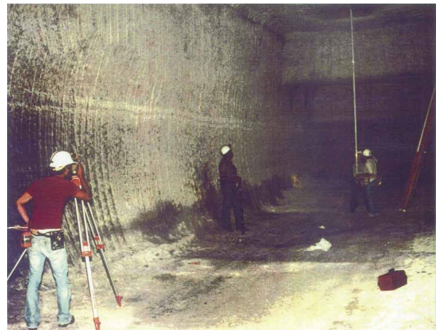
(b) Room D being surveyed (Munson et al. 1988)
