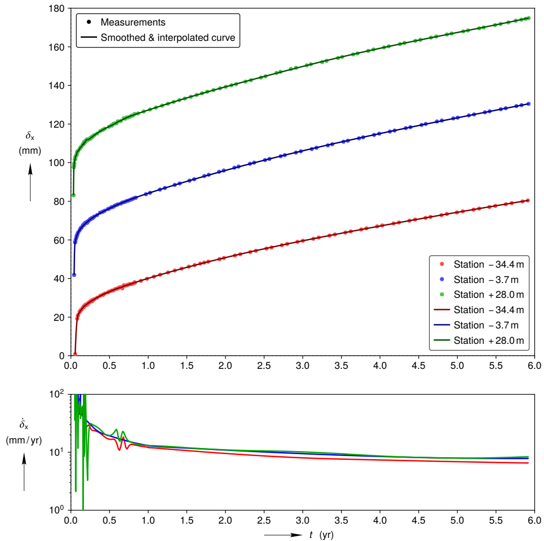
Figure D-8. Room Q smoothed and interpolated full horizontal closure curves compared against spliced together mining sequence and remotely read closure measurements in the top plot. (Each successive station's horizontal closure curve and measurements are shifted up by 40 mm to enhance legibility.) Closure rate curves computed from the smoothed closure curves in the bottom plot.
