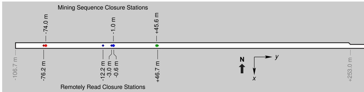
(a) Closure station locations
