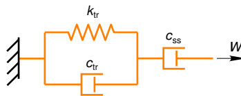
Figure 2-3. Jeffreys element: a spring in parallel with a dashpot, which are both in series with a second dashpot.
