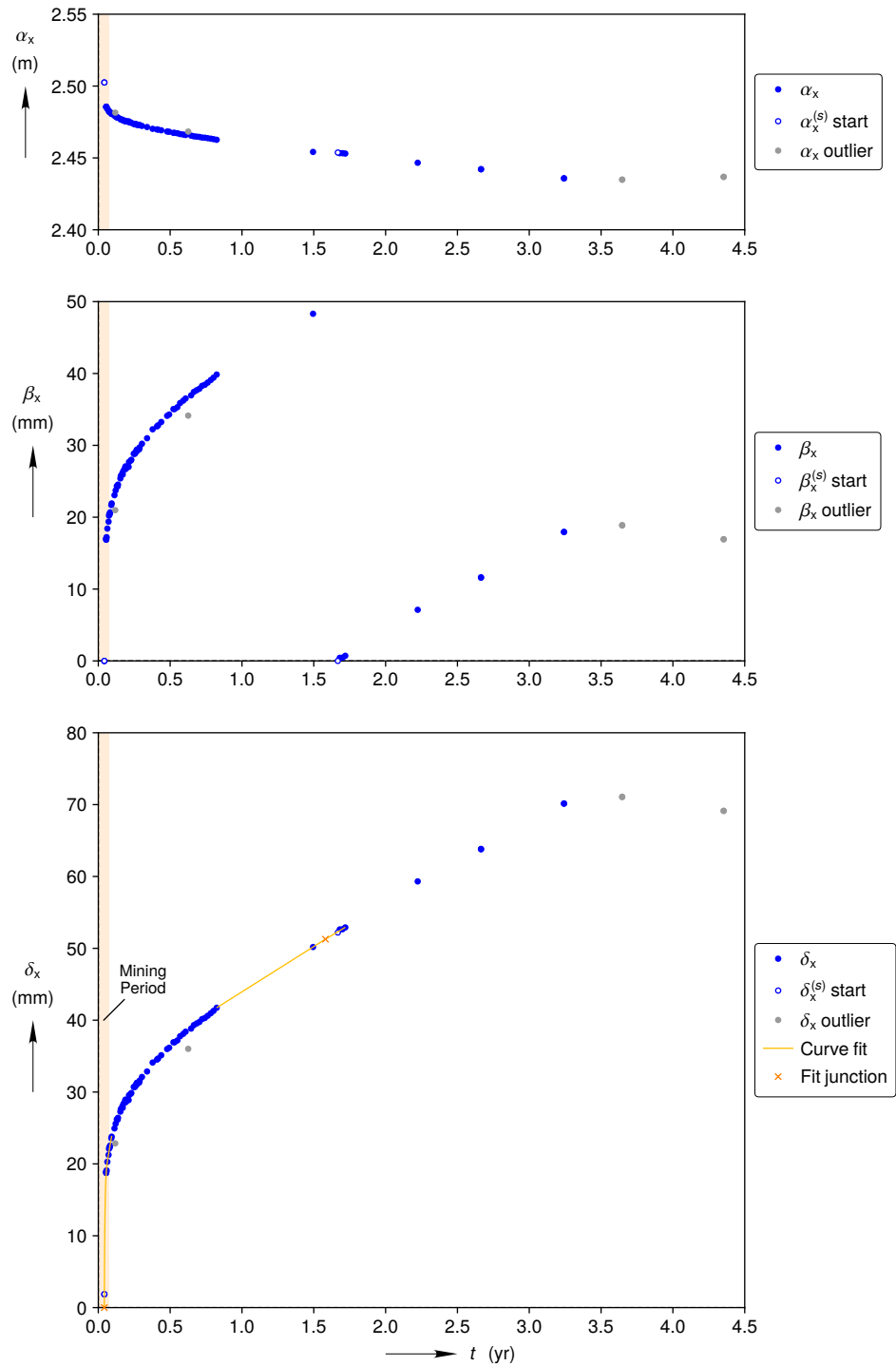
(b) Full reconstruction
