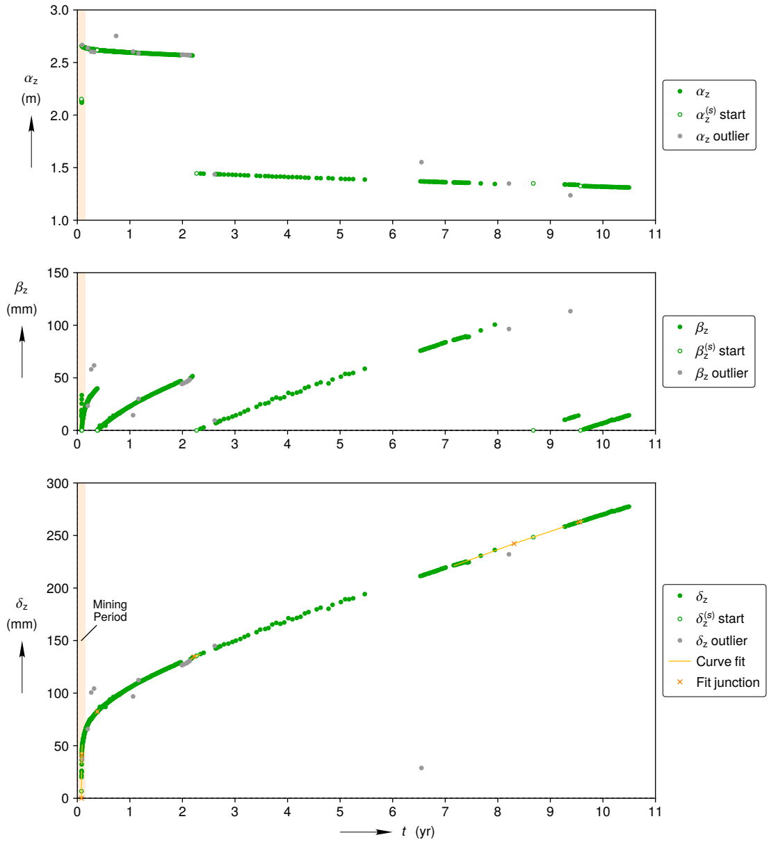
(b) Full reconstruction
