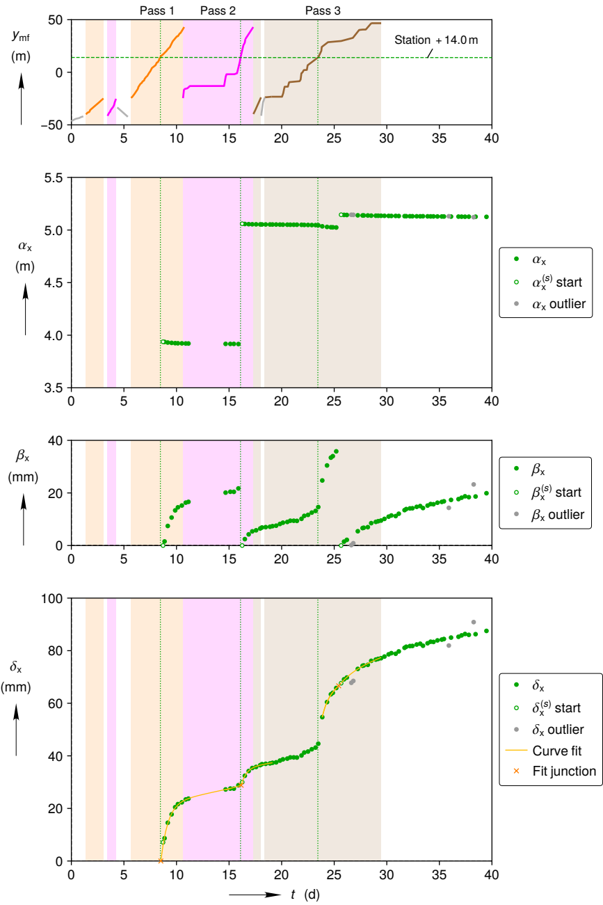
(a) Reconstruction during mining period
