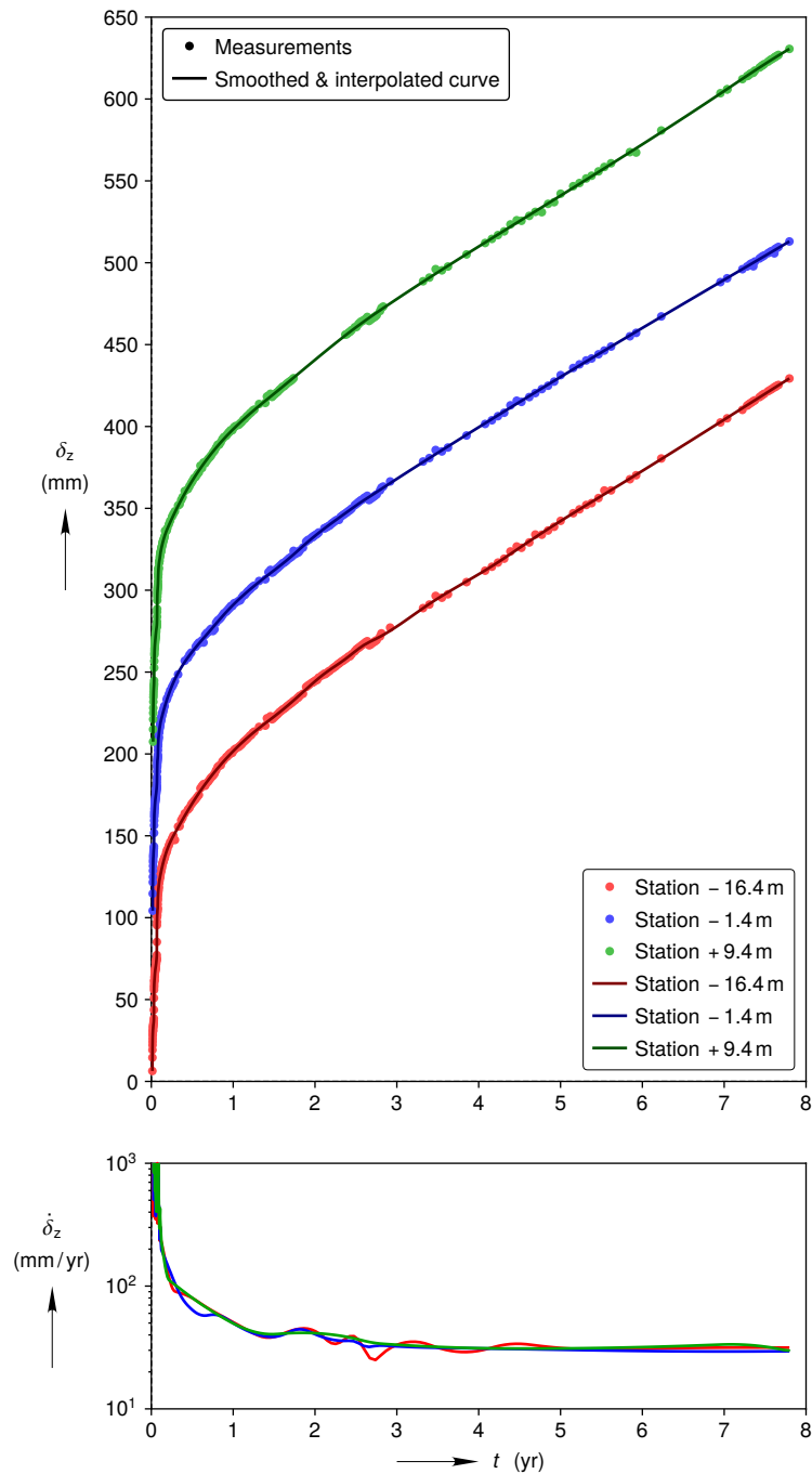
Figure A-10. Room D smoothed and interpolated full vertical closure curves compared against re-constructed mining sequence closure measurements in the top plot. (Each successive station's vertical closure curve and measurements are shifted up by 100 mm to enhance legibility.) Closure rate curves computed from the smoothed closure curves in the bottom plot.
