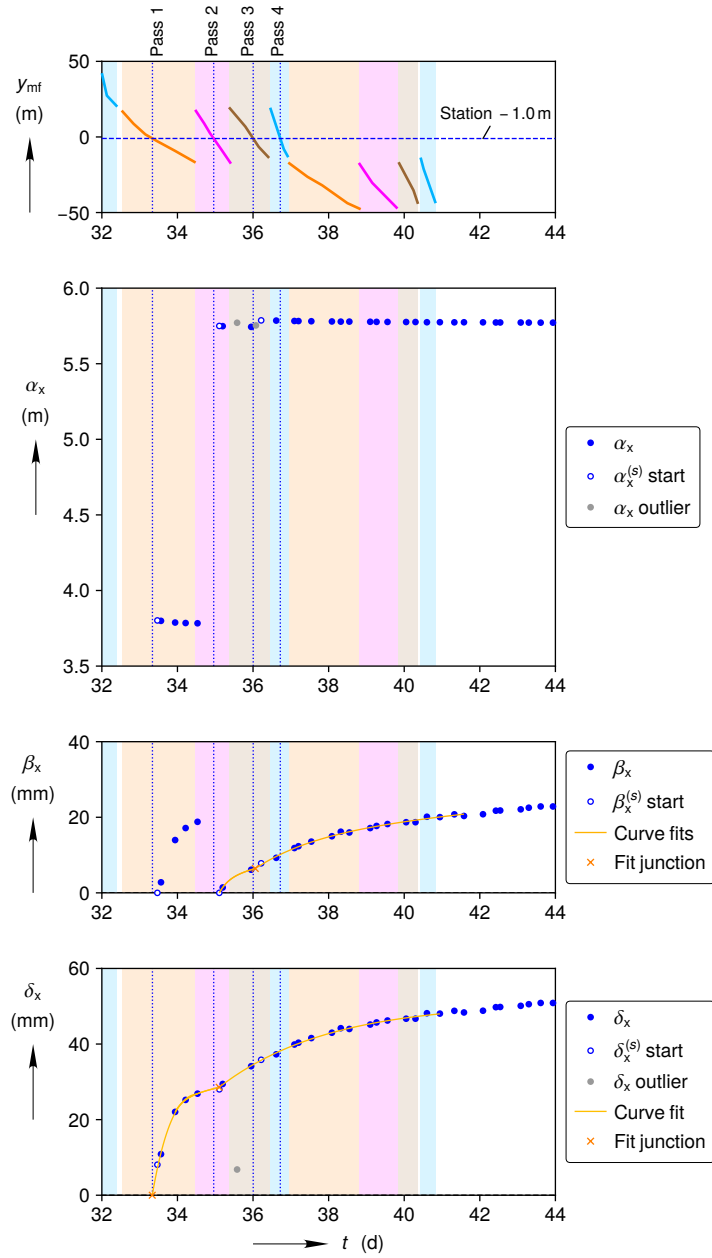
(a) Reconstruction during mining period
