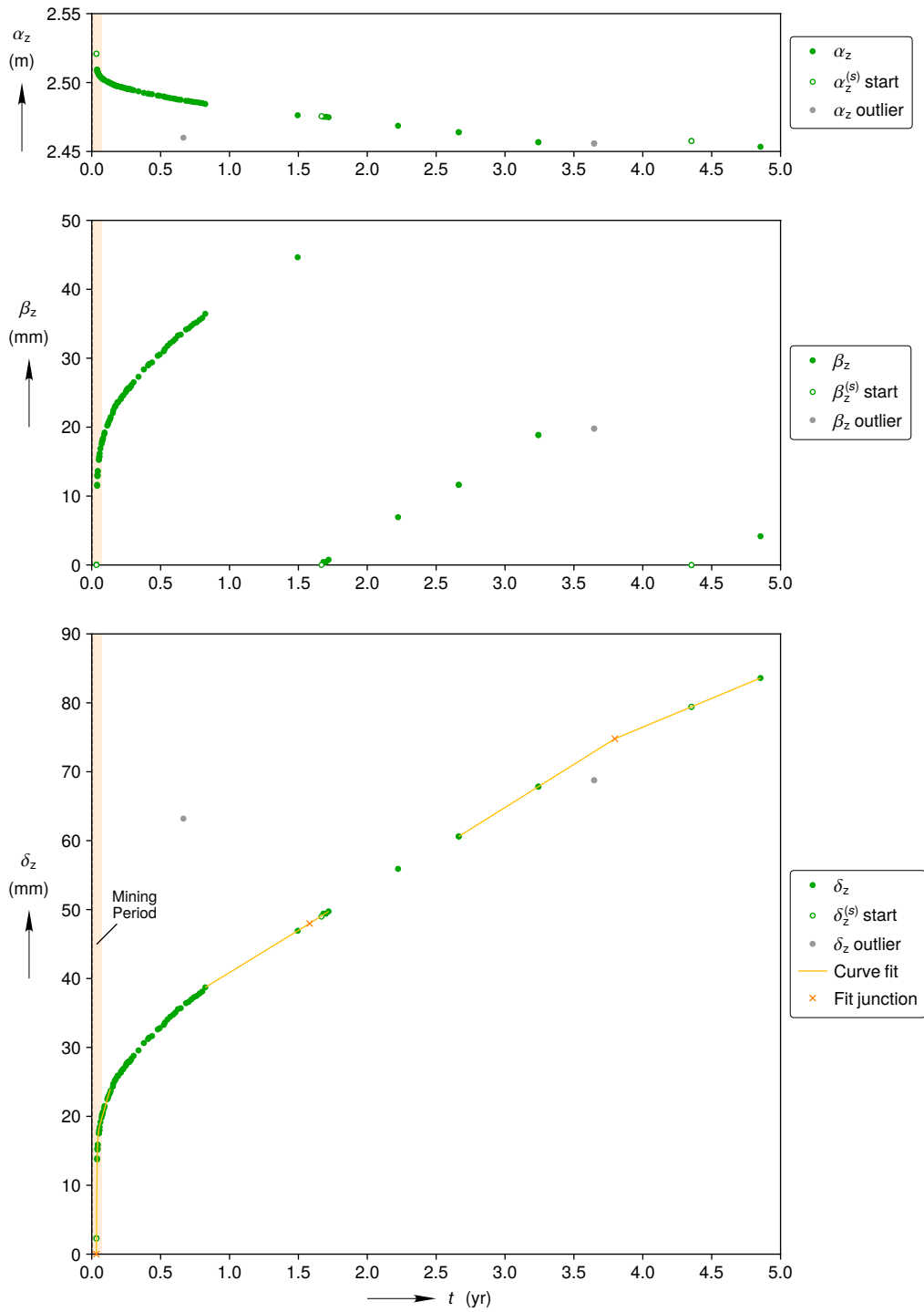
(b) Full reconstruction
