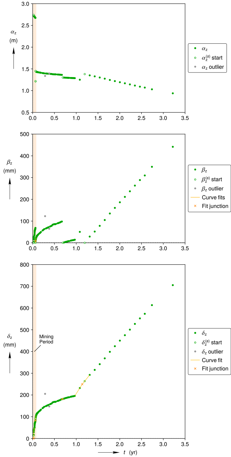
(b) Full reconstruction
