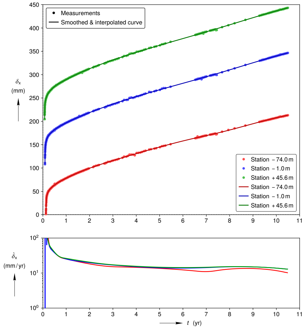
Figure C-8. Room G smoothed and interpolated full horizontal closure curves compared against reconstructed mining sequence closure measurements in the top plot. (Each successive station's horizontal closure curve and measurements are shifted up by 100 mm to enhance legibility.) Closure rate curves computed from the smoothed closure curves in the bottom plot.
