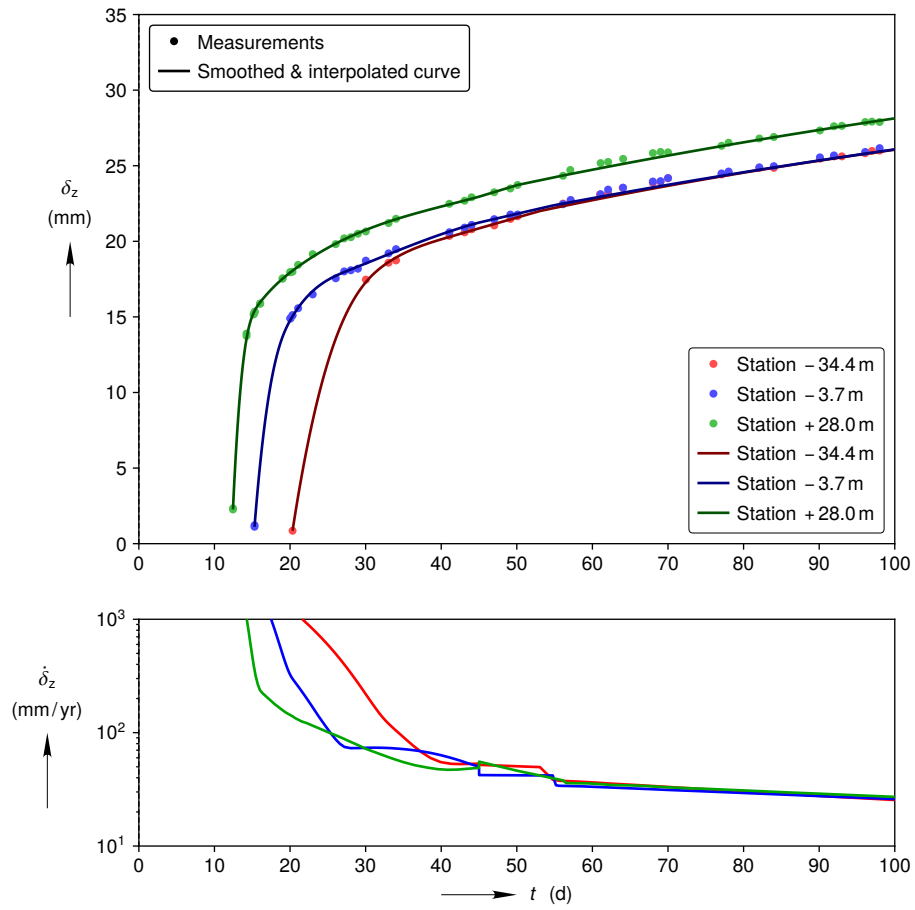
Figure D-9. Room Q smoothed and interpolated vertical closure curves compared against reconstructed mining sequence closure measurements during mining in the top plot. Closure rate curves computed from the smoothed closure curves during mining in the bottom plot.
