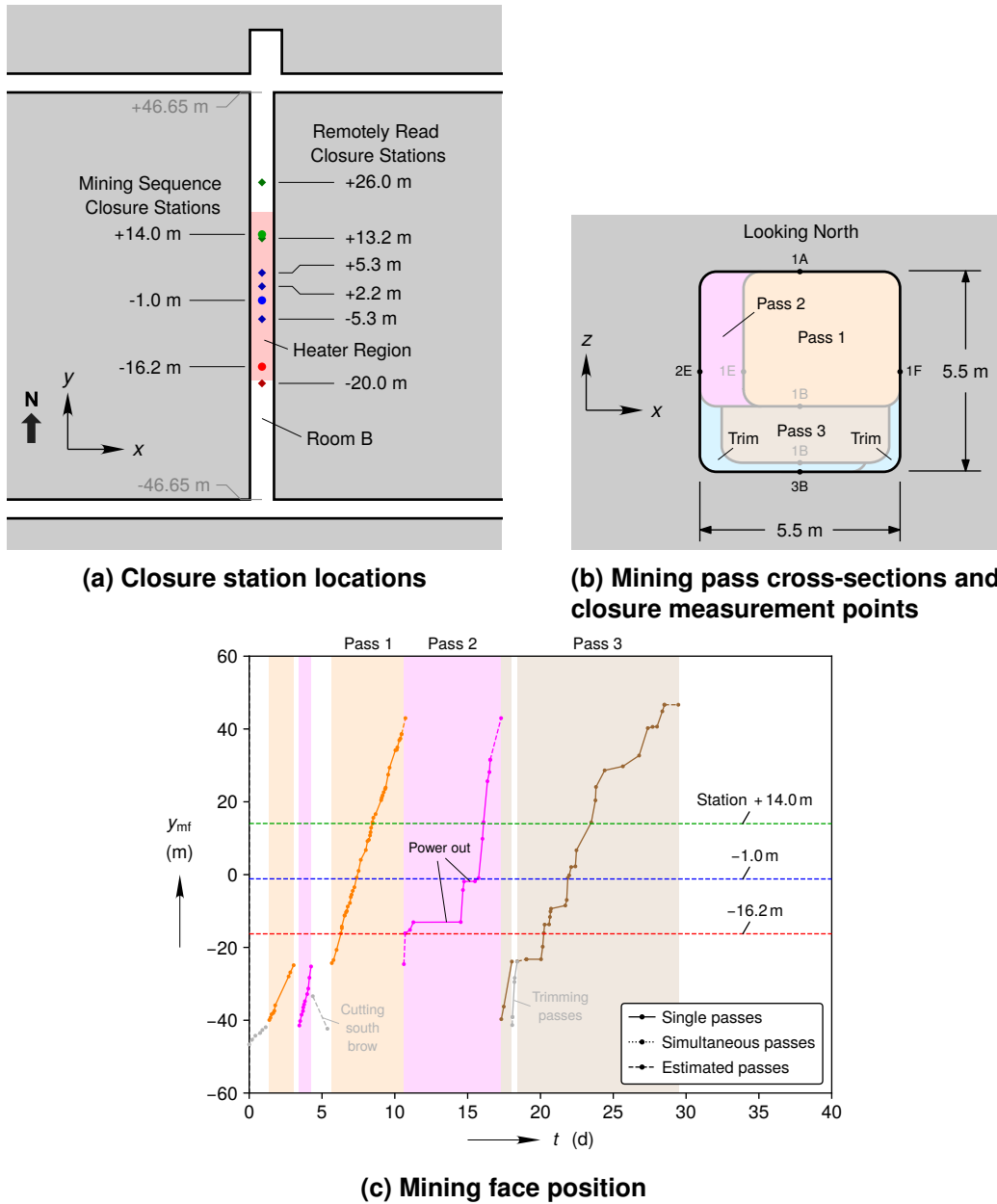
Figure 3-5. Room B plan view, mining cross-section, and mining face position. The mining cross-section and mining face position are derived from Fig. 2.2.10 and 2.2.11, and Table 2.2.1, in Munson et al. (1992a).
