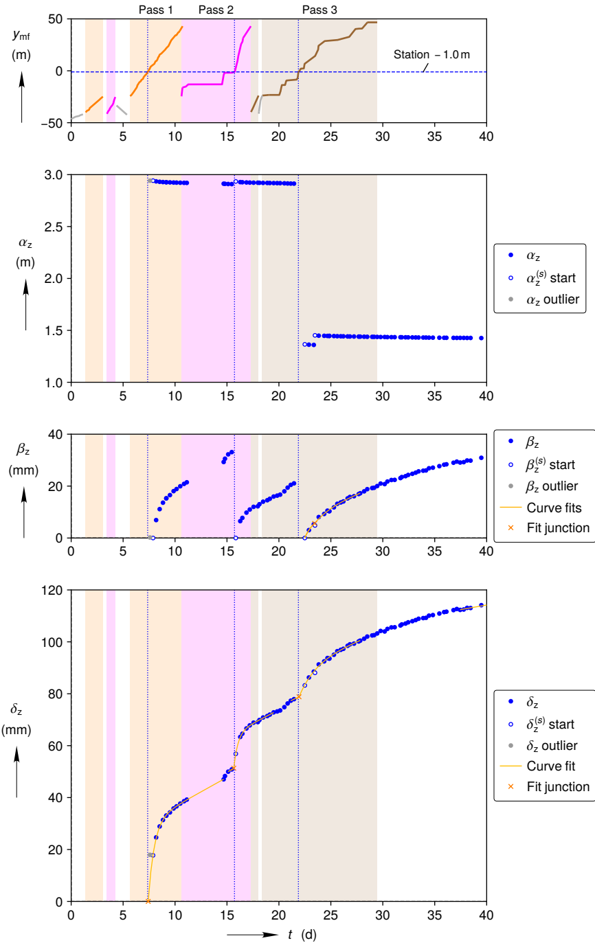
Figure 3-6. Room B mining sequence station -1.0 m vertical closure reconstruction process during mining.
